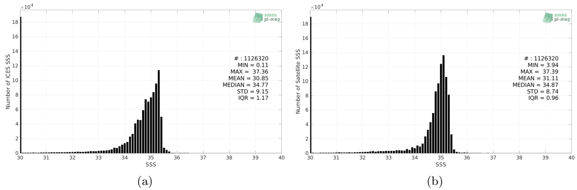
Figure 2: Histograms of SSS from ICES (a) and SMOS SSS L4 v1 - Weekly (CMEMS-CNR) (b) considering all match-up pairs per bins of 0.1 over the SMOS coastal zone (<800km) 60N-60S Pi-MEP region and for the full satellite product period.
