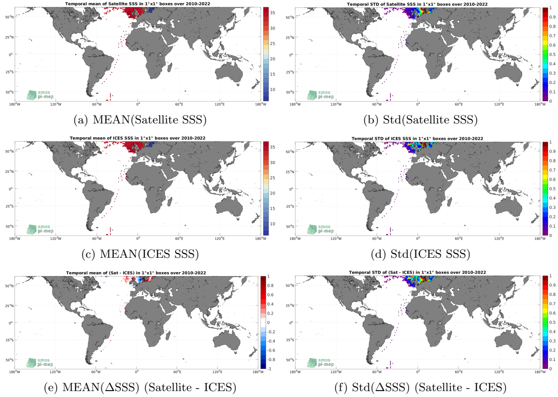
Figure 6: Temporal mean (left) and Std (right) of SSS from SMOS SSS L4 v1 - Weekly (CMEMS-CNR) (top), ICES (middle), and of \Delta SSS (Satellite - ICES). Only match-up pairs are used to generate these maps.
