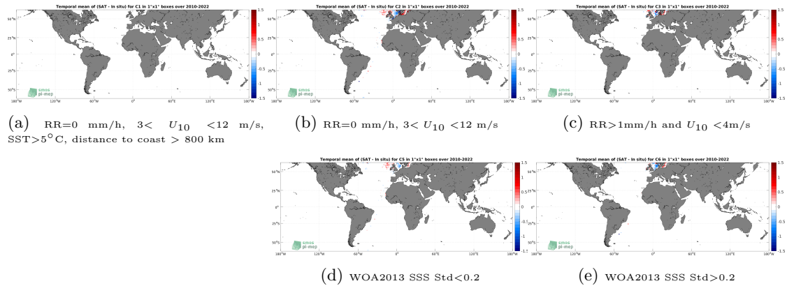
Figure 12: Temporal mean gridded over spatial boxes of size 1^\circ \times 1^\circ of \Delta\text{SSS} (SMOS SSS L4 v1 - Weekly (CMEMS-CNR) - ICES) for 5 different subdatasets corresponding to:RR=0 mm/h, 3 < U_{10} < 12 m/s, SST >5^\circ\text{C} , distance to coast > 800 km (a), RR=0 mm/h, 3 < U_{10} < 12 m/s (b), RR >1 mm/h and U_{10} < 4 m/s (c), WOA2013 SSS Std <0.2 (d), WOA2013 SSS Std >0.2 (e).
