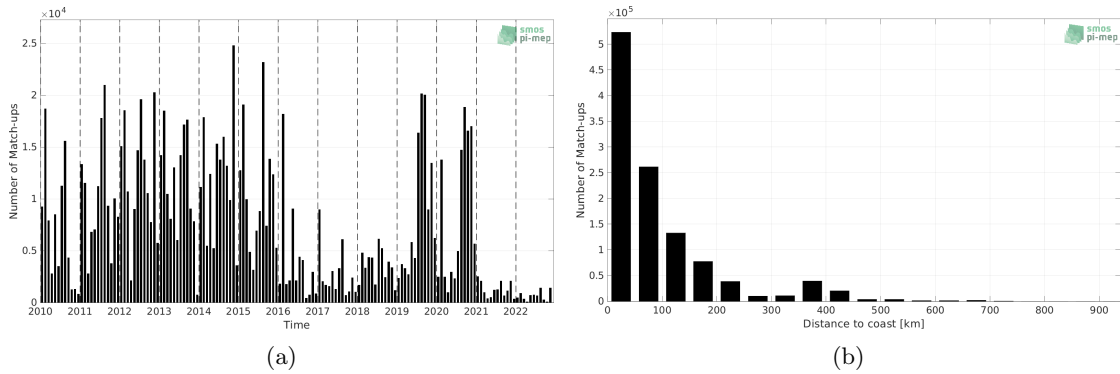
Figure 1: Number of match-ups between ICES and SMOS SSS L4 v1 - Weekly (CMEMS-CNR) SSS as a function of time (a) and as function of the distance to coast (b) over the SMOS coastal zone (<800km) 60N-60S Pi-MEP region and for the full satellite product period.
