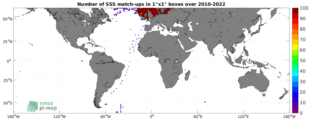
Figure 4: Number of SSS match-ups between ICES SSS and the SMOS SSS L4 v1 - Weekly (CMEMS-CNR) SSS product for the SMOS coastal zone (<800km) 60N-60S Pi-MEP region over 1^\circ \times 1^\circ boxes and for the full satellite product period.
