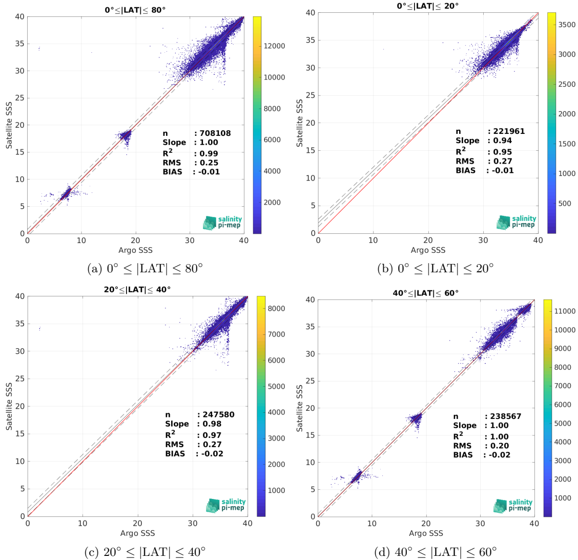
Figure 9: Contour maps of the concentration of SMOS SSS L4 v1 - Weekly (CMEMS-CNR) SSS (y-axis) versus Argo SSS (x-axis) at match-up pairs for different latitude bands. For each plot, the red line shows x=y . The black thin and dashed lines indicate a linear fit through the data cloud and the \pm 95\% confidence levels, respectively. The number match-up pairs n , the slope and R^2 coefficient of the linear fit, the root mean square (RMS) and the mean bias between satellite and in situ data are indicated for each latitude band in each plot.
