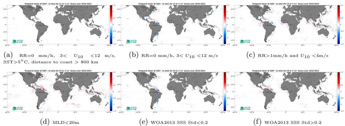
Figure 12: Temporal mean gridded over spatial boxes of size 1^\circ \times 1^\circ of \Delta SSS (SMOS SSS L4 v1 - Weekly (CMEMS-CNR) - Argo) for 6 different subdatasets corresponding to:RR=0 mm/h, 3 < U_{10} < 12 m/s, SST > 5^\circ\text{C} , distance to coast > 800 km (a), RR=0 mm/h, 3 < U_{10} < 12 m/s (b), RR > 1 mm/h and U_{10} < 4 m/s (c),MLD < 20 m (d),WOA2013 SSS Std < 0.2 (e),WOA2013 SSS Std > 0.2 (f).
