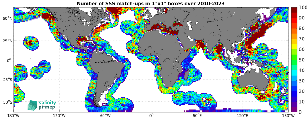
Figure 4: Number of SSS match-ups between Argo SSS and the SMOS SSS L4 v1 - Weekly (CMEMS-CNR) SSS product for the SMOS coastal zone (<800km) 60N-60S Pi-MEP region over 1^\circ \times 1^\circ boxes and for the full satellite product period.
