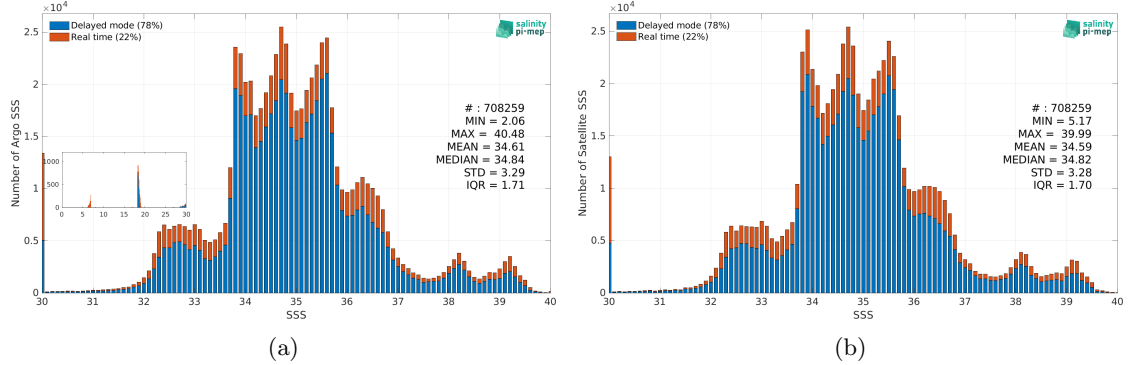
Figure 2: Histograms of SSS from Argo (a) and SMOS SSS L4 v1 - Weekly (CMEMS-CNR) (b) considering all match-up pairs per bins of 0.1 over the SMOS coastal zone (<800km) 60N-60S Pi-MEP region and for the full satellite product period.
