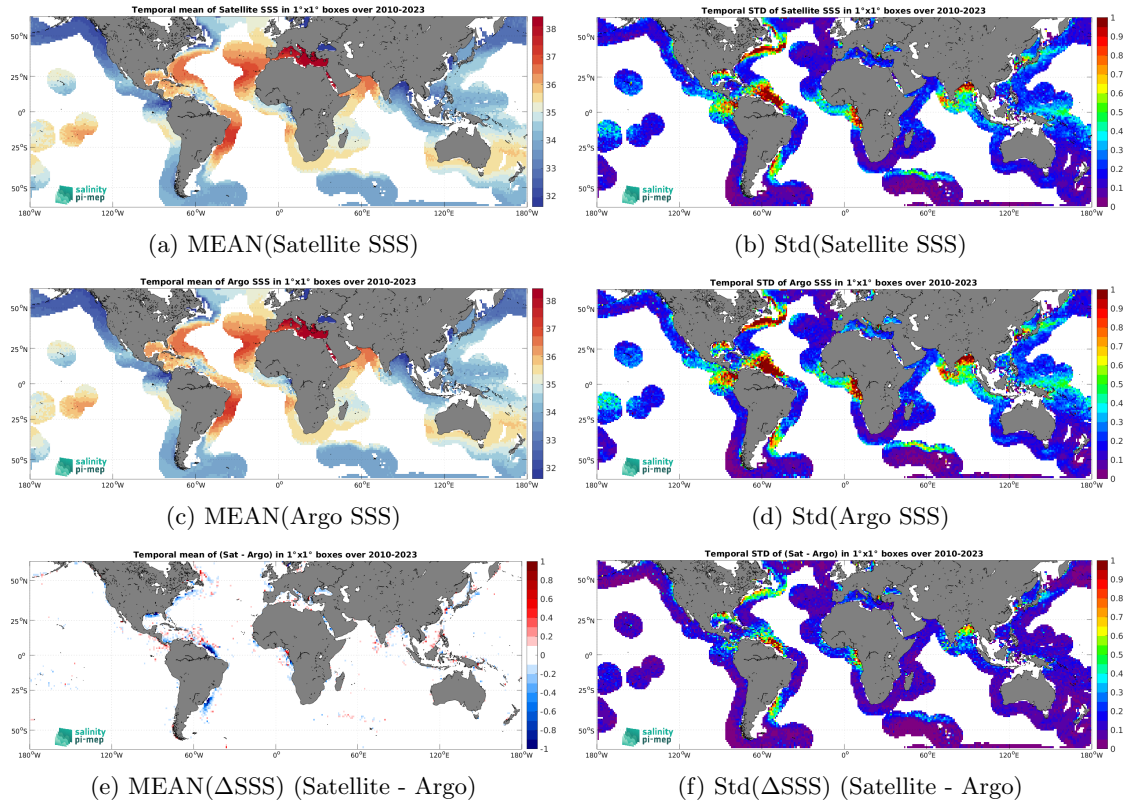
Figure 6: Temporal mean (left) and Std (right) of SSS from SMOS SSS L4 v1 - Weekly (CMEMS-CNR) (top), Argo (middle), and of \Delta SSS (Satellite - Argo). Only match-up pairs are used to generate these maps.
