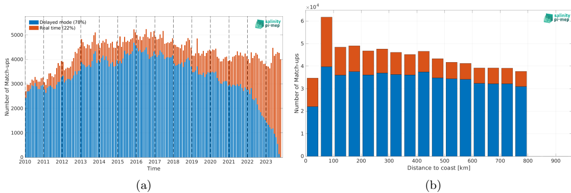
Figure 1: Number of match-ups between Argo and SMOS SSS L4 v1 - Weekly (CMEMS-CNR) SSS as a function of time (a) and as function of the distance to coast (b) over the SMOS coastal zone ( < 800\text{km} ) 60N-60S Pi-MEP region and for the full satellite product period.
