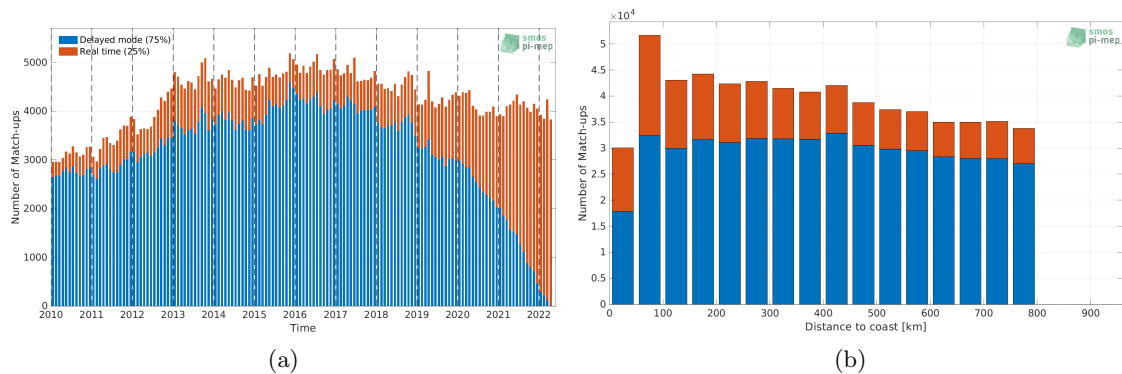
Figure 1: Number of match-ups between Argo and SMOS SSS L4 v1 - Weekly (CMEMS-CNR) SSS as a function of time (a) and as function of the distance to coast (b) over the SMOS coastal zone (<800km) 60N-60S Pi-MEP region and for the full satellite product period.
