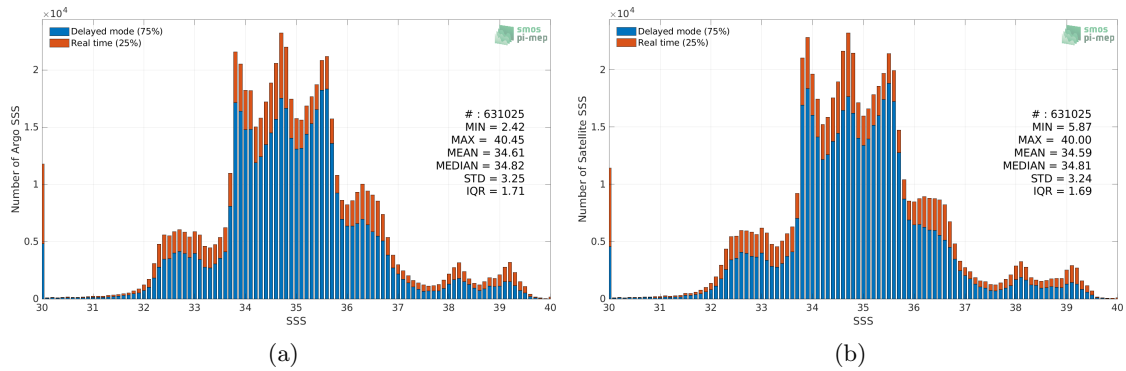
Figure 2: Histograms of SSS from Argo (a) and SMOS SSS L4 v1 - Weekly (CMEMS-CNR) (b) considering all match-up pairs per bins of 0.1 over the SMOS coastal zone (<800km) 60N-60S Pi-MEP region and for the full satellite product period.
