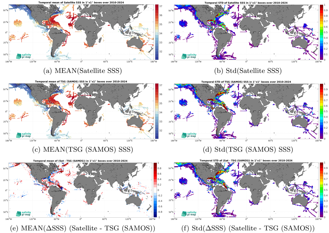
Figure 7: Temporal mean (left) and Std (right) of SSS from SMOS SSS L4 v1 - Monthly (CMEMS-CNR) (top), TSG (SAMOS) (middle), and of \Delta SSS (Satellite - TSG (SAMOS)). Only match-up pairs are used to generate these maps.
