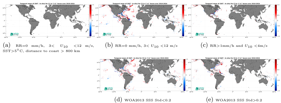
Figure 14: Temporal mean gridded over spatial boxes of size 1^\circ \times 1^\circ of \Delta SSS (SMOS SSS L4 v1 - Monthly (CMEMS-CNR) - TSG (SAMOS)) for 5 different subdatasets corresponding to:RR=0 mm/h, 3 < U_{10} < 12 m/s, SST > 5^\circ\text{C} , distance to coast > 800 km (a), RR=0 mm/h, 3 < U_{10} < 12 m/s (b), RR > 1 mm/h and U_{10} < 4 m/s (c), WOA2013 SSS Std < 0.2 (d), WOA2013 SSS Std > 0.2 (e).
