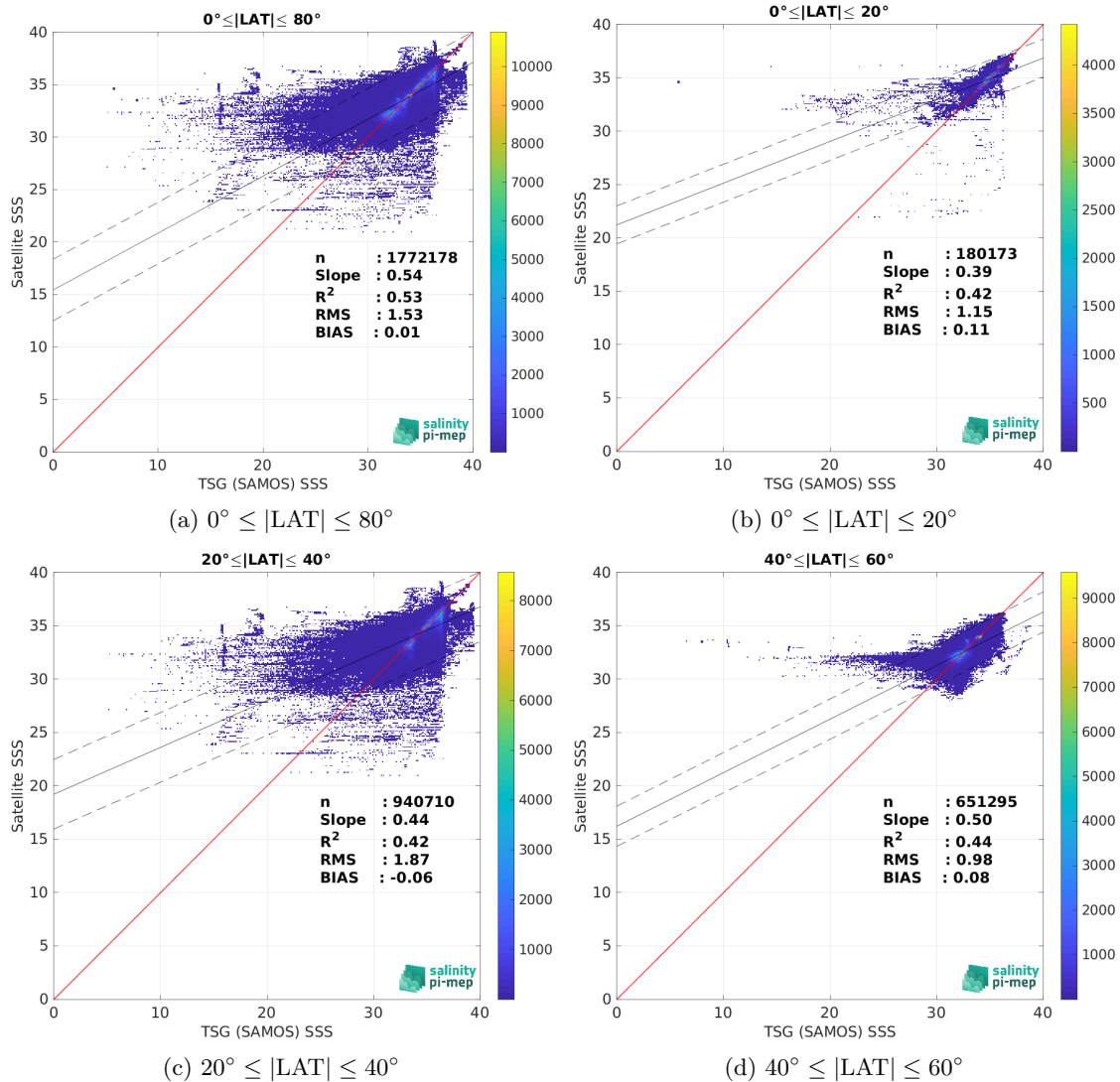
Figure 10: Contour maps of the concentration of SMOS SSS L4 v1 - Monthly (CMEMS-CNR) SSS (y-axis) versus TSG (SAMOS) SSS (x-axis) at match-up pairs for different latitude bands. For each plot, the red line shows x=y . The black thin and dashed lines indicate a linear fit through the data cloud and the \pm 95\% confidence levels, respectively. The number match-up pairs n , the slope and R^2 coefficient of the linear fit, the root mean square (RMS) and the mean bias between satellite and in situ data are indicated for each latitude band in each plot.
