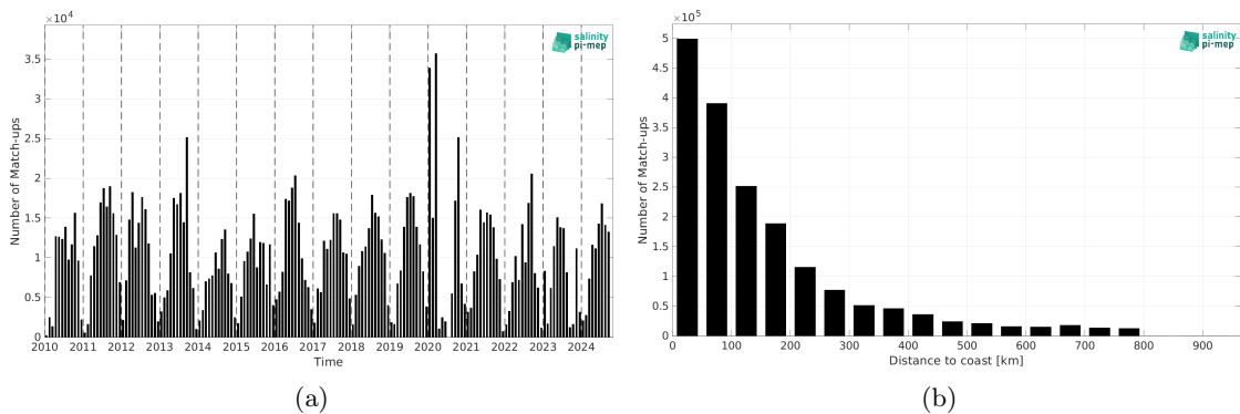
Figure 2: Number of match-ups between TSG (SAMOS) and SMOS SSS L4 v1 - Monthly (CMEMS-CNR) SSS as a function of time (a) and as function of the distance to coast (b) over the SMOS coastal zone (<800km) 60N-60S Pi-MEP region and for the full satellite product period.
