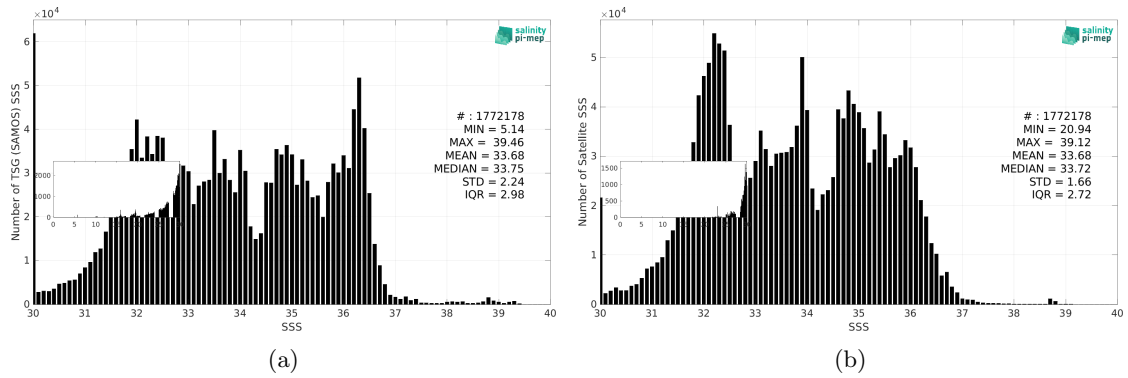
Figure 3: Histograms of SSS from TSG (SAMOS) (a) and SMOS SSS L4 v1 - Monthly (CMEMS-CNR) (b) considering all match-up pairs per bins of 0.1 over the SMOS coastal zone (<800km) 60N-60S Pi-MEP region and for the full satellite product period.
