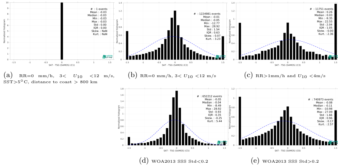
Figure 15: Normalized histogram of \Delta SSS (SMOS SSS L4 v1 - Monthly (CMEMS-CNR) - TSG (SAMOS)) for 5 different subdatasets corresponding to: RR=0 mm/h, 3 < U_{10} < 12 m/s, SST > 5°C, distance to coast > 800 km (a), RR=0 mm/h, 3 < U_{10} < 12 m/s (b), RR > 1mm/h and U_{10} < 4 m/s (c), WOA2013 SSS Std < 0.2 (d), WOA2013 SSS Std > 0.2 (e).
