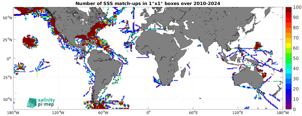
Figure 5: Number of SSS match-ups between TSG (SAMOS) SSS and the SMOS SSS L4 v1 - Monthly (CMEMS-CNR) SSS product for the SMOS coastal zone (<800km) 60N-60S Pi-MEP region over 1^{\circ} \times 1^{\circ} boxes and for the full satellite product period.
