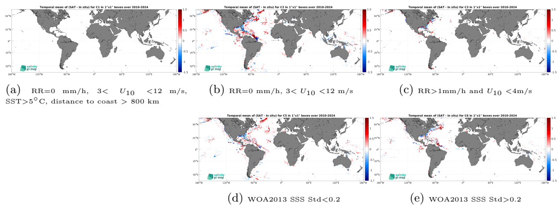
Figure 14: Temporal mean gridded over spatial boxes of size 1^\circ \times 1^\circ of \Delta\text{SSS} (SMOS SSS L4 v1 - Monthly (CMEMS-CNR) - TSG (SAMOS)) for 5 different subdatasets corresponding to:RR=0 mm/h, 3 < U_{10} < 12 m/s, SST >5^\circ\text{C} , distance to coast > 800 km (a), RR=0 mm/h, 3 < U_{10} < 12 m/s (b), RR >1 mm/h and U_{10} < 4 m/s (c), WOA2013 SSS Std <0.2 (d), WOA2013 SSS Std >0.2 (e).
