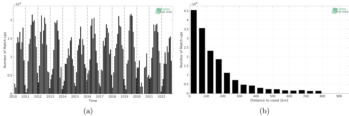
Figure 1: Number of match-ups between TSG (SAMOS) and SMOS SSS L4 v1 - Monthly (CMEMS-CNR) SSS as a function of time (a) and as function of the distance to coast (b) over the SMOS coastal zone (<800km) 60N-60S Pi-MEP region and for the full satellite product period.
