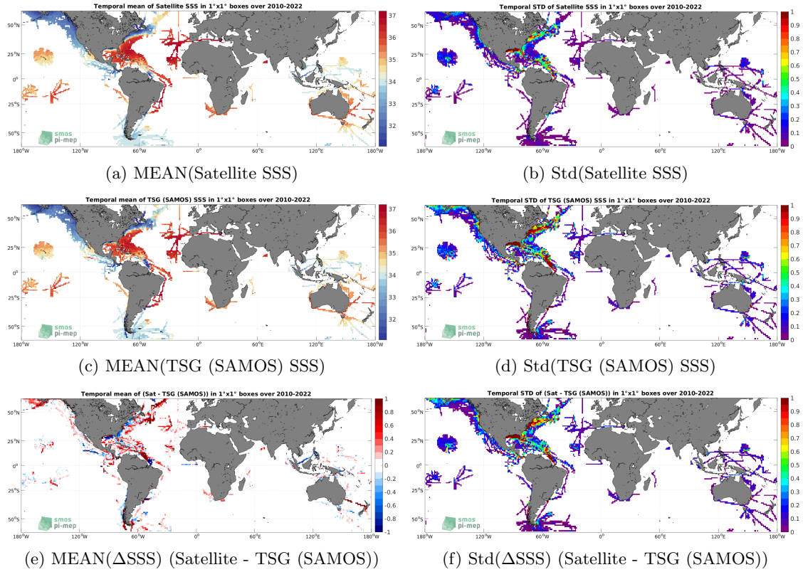
Figure 6: Temporal mean (left) and Std (right) of SSS from SMOS SSS L4 v1 - Monthly (CMEMS-CNR) (top), TSG (SAMOS) (middle), and of \Delta SSS (Satellite - TSG (SAMOS)). Only match-up pairs are used to generate these maps.
