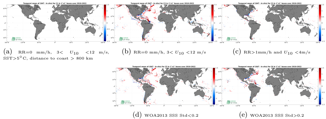
Figure 12: Temporal mean gridded over spatial boxes of size 1^\circ \times 1^\circ of \Delta SSS (SMOS SSS L4 v1 - Monthly (CMEMS-CNR) - TSG (SAMOS)) for 5 different subdatasets corresponding to:RR=0 mm/h, 3 < U_{10} < 12 m/s, SST >5^\circ C, distance to coast > 800 km (a), RR=0 mm/h, 3 < U_{10} < 12 m/s (b), RR >1 mm/h and U_{10} < 4 m/s (c), WOA2013 SSS Std <0.2 (d), WOA2013 SSS Std >0.2 (e).
