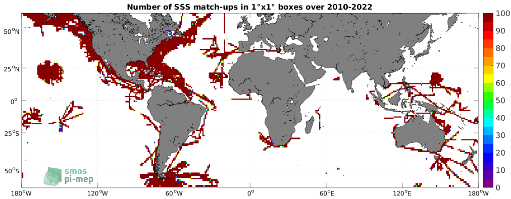
Figure 4: Number of SSS match-ups between TSG (SAMOS) SSS and the SMOS SSS L4 v1 - Monthly (CMEMS-CNR) SSS product for the SMOS coastal zone (<800km) 60N-60S Pi-MEP region over 1^{\circ} \times 1^{\circ} boxes and for the full satellite product period.
