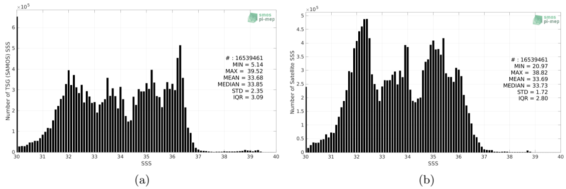
Figure 2: Histograms of SSS from TSG (SAMOS) (a) and SMOS SSS L4 v1 - Monthly (CMEMS-CNR) (b) considering all match-up pairs per bins of 0.1 over the SMOS coastal zone (<800km) 60N-60S Pi-MEP region and for the full satellite product period.
