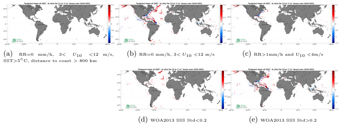
Figure 12: Temporal mean gridded over spatial boxes of size 1^\circ \times 1^\circ of \Delta\text{SSS} (SMOS SSS L4 v1 - Monthly (CMEMS-CNR) - TSG (SAMOS)) for 5 different subdatasets corresponding to:RR=0 mm/h, 3 < U_{10} < 12 m/s, SST >5^\circ\text{C} , distance to coast > 800 km (a), RR=0 mm/h, 3 < U_{10} < 12 m/s (b), RR >1 mm/h and U_{10} < 4 m/s (c), WOA2013 SSS Std <0.2 (d), WOA2013 SSS Std >0.2 (e).
