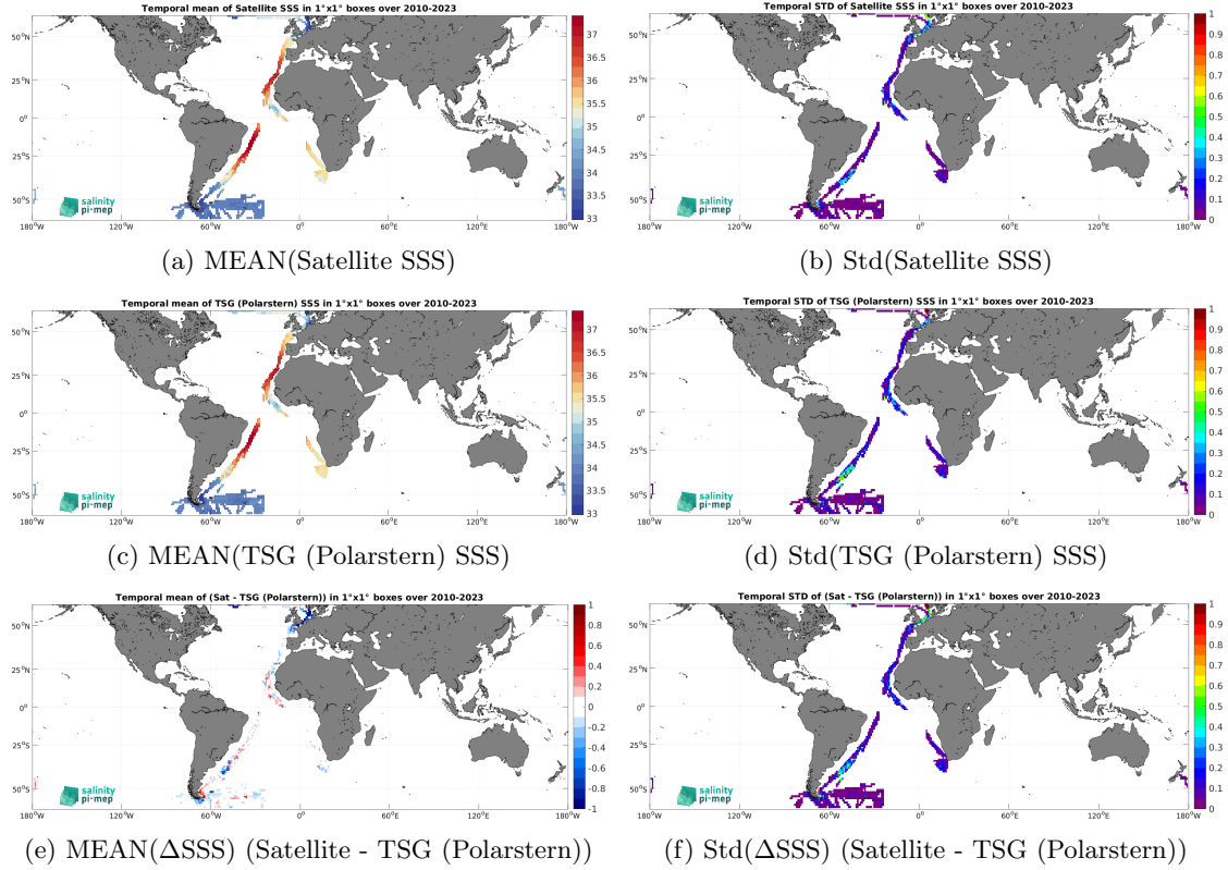
Figure 7: Temporal mean (left) and Std (right) of SSS from SMOS SSS L4 v1 - Monthly (CMEMS-CNR) (top), TSG (Polarstern) (middle), and of \Delta SSS (Satellite - TSG (Polarstern)). Only match-up pairs are used to generate these maps.
