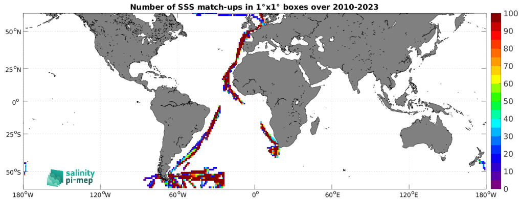
Figure 5: Number of SSS match-ups between TSG (Polarstern) SSS and the SMOS SSS L4 v1 - Monthly (CMEMS-CNR) SSS product for the SMOS coastal zone (<800km) 60N-60S Pi-MEP region over 1^{\circ} \times 1^{\circ} boxes and for the full satellite product period.
