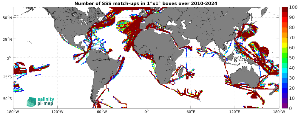
Figure 5: Number of SSS match-ups between TSG (LEGOS-DM) SSS and the SMOS SSS L4 v1 - Monthly (CMEMS-CNR) SSS product for the SMOS coastal zone (<800km) 60N-60S Pi-MEP region over 1^{\circ} \times 1^{\circ} boxes and for the full satellite product period.
