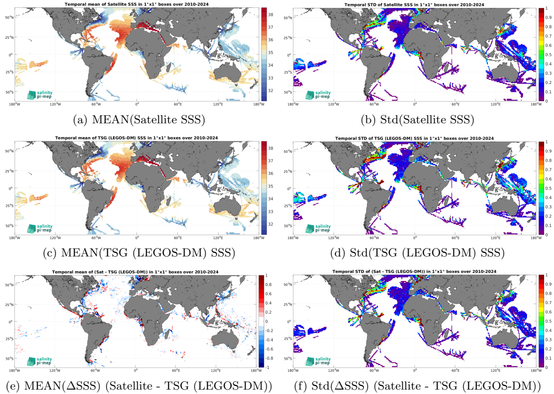
Figure 7: Temporal mean (left) and Std (right) of SSS from SMOS SSS L4 v1 - Monthly (CMEMS-CNR) (top), TSG (LEGOS-DM) (middle), and of \Delta SSS (Satellite - TSG (LEGOS-DM)). Only match-up pairs are used to generate these maps.
