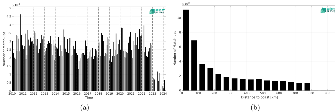
Figure 2: Number of match-ups between TSG (LEGOS-DM) and SMOS SSS L4 v1 - Monthly (CMEMS-CNR) SSS as a function of time (a) and as function of the distance to coast (b) over the SMOS coastal zone (<800km) 60N-60S Pi-MEP region and for the full satellite product period.
