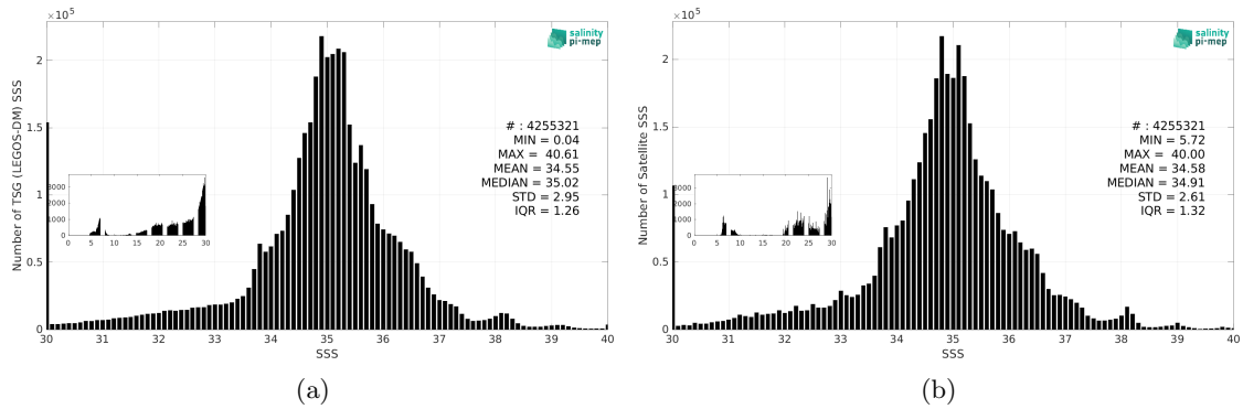
Figure 3: Histograms of SSS from TSG (LEGOS-DM) (a) and SMOS SSS L4 v1 - Monthly (CMEMS-CNR) (b) considering all match-up pairs per bins of 0.1 over the SMOS coastal zone (<800km) 60N-60S Pi-MEP region and for the full satellite product period.
