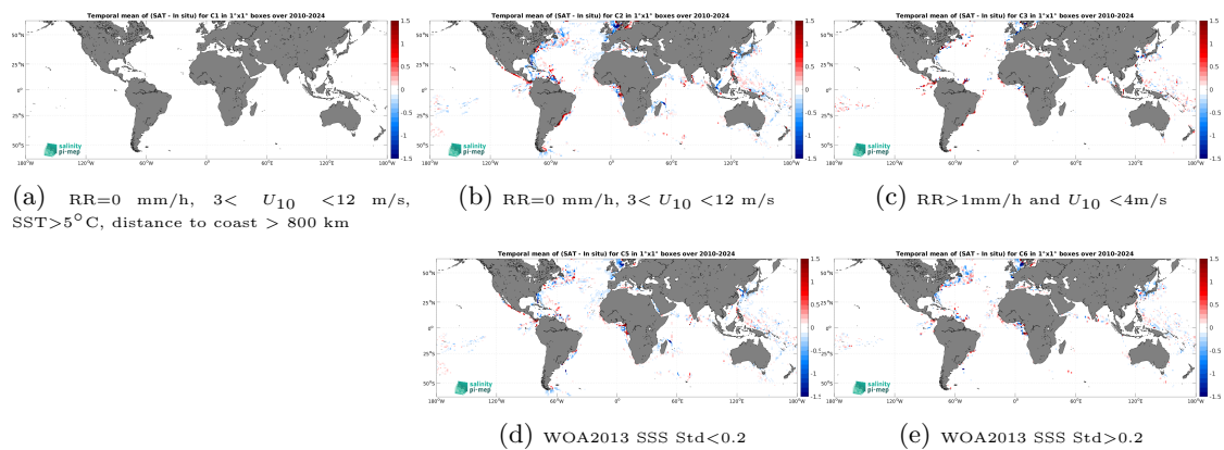
Figure 14: Temporal mean gridded over spatial boxes of size 1^\circ \times 1^\circ of \Delta SSS (SMOS SSS L4 v1 - Monthly (CMEMS-CNR) - TSG (LEGOS-DM)) for 5 different subdatasets corresponding to:RR=0 mm/h, 3 < U_{10} < 12 m/s, SST >5^\circ C, distance to coast > 800 km (a), RR=0 mm/h, 3 < U_{10} < 12 m/s (b), RR >1 mm/h and U_{10} < 4 m/s (c), WOA2013 SSS Std <0.2 (d), WOA2013 SSS Std >0.2 (e).
