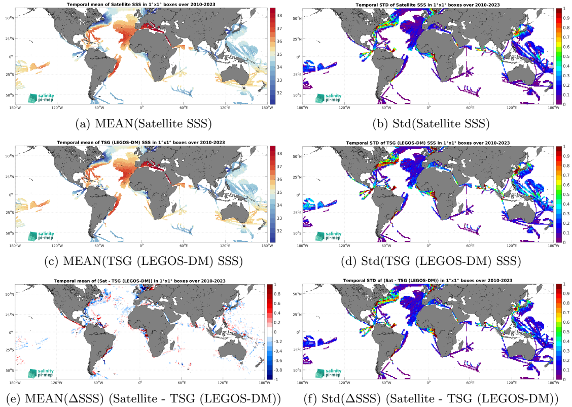
Figure 6: Temporal mean (left) and Std (right) of SSS from SMOS SSS L4 v1 - Monthly (CMEMS-CNR) (top), TSG (LEGOS-DM) (middle), and of \Delta SSS (Satellite - TSG (LEGOS-DM)). Only match-up pairs are used to generate these maps.
