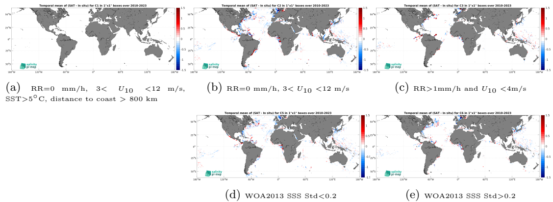
Figure 12: Temporal mean gridded over spatial boxes of size 1^\circ \times 1^\circ of \Delta SSS (SMOS SSS L4 v1 - Monthly (CMEMS-CNR) - TSG (LEGOS-DM)) for 5 different subdatasets corresponding to:RR=0 mm/h, 3 < U_{10} < 12 m/s, SST >5^\circ C, distance to coast > 800 km (a), RR=0 mm/h, 3 < U_{10} < 12 m/s (b), RR >1 mm/h and U_{10} < 4 m/s (c), WOA2013 SSS Std <0.2 (d), WOA2013 SSS Std >0.2 (e).
