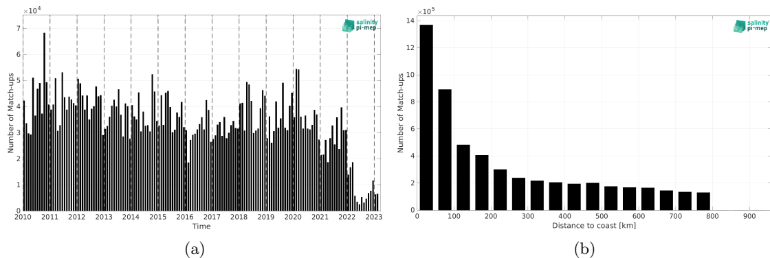
Figure 1: Number of match-ups between TSG (LEGOS-DM) and SMOS SSS L4 v1 - Monthly (CMEMS-CNR) SSS as a function of time (a) and as function of the distance to coast (b) over the SMOS coastal zone (<800km) 60N-60S Pi-MEP region and for the full satellite product period.
