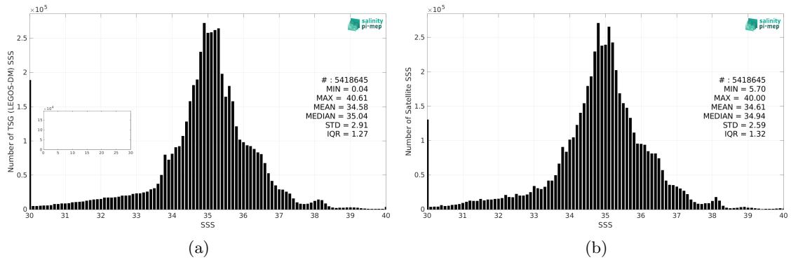
Figure 2: Histograms of SSS from TSG (LEGOS-DM) (a) and SMOS SSS L4 v1 - Monthly (CMEMS-CNR) (b) considering all match-up pairs per bins of 0.1 over the SMOS coastal zone (<800km) 60N-60S Pi-MEP region and for the full satellite product period.
