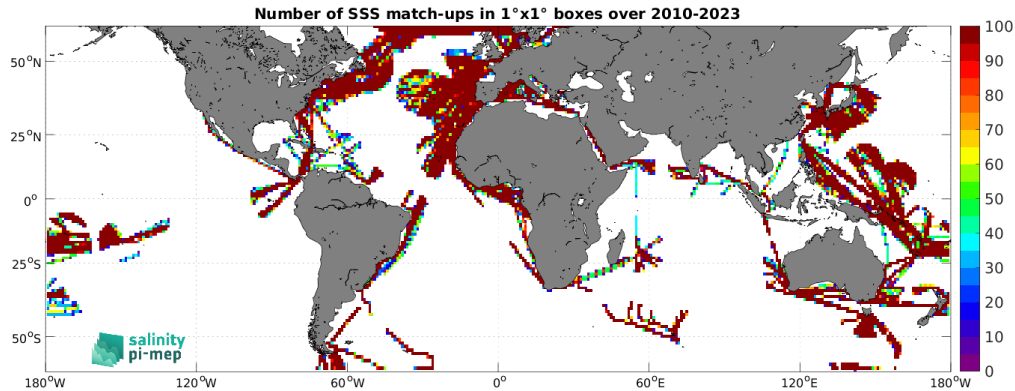
Figure 4: Number of SSS match-ups between TSG (LEGOS-DM) SSS and the SMOS SSS L4 v1 - Monthly (CMEMS-CNR) SSS product for the SMOS coastal zone (<800km) 60N-60S Pi-MEP region over 1^\circ \times 1^\circ boxes and for the full satellite product period.
