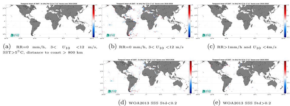
Figure 14: Temporal mean gridded over spatial boxes of size 1^\circ \times 1^\circ of \Delta SSS (SMOS SSS L4 v1 - Monthly (CMEMS-CNR) - TSG (GOSUD-Sailing-ship)) for 5 different subdatasets corresponding to:RR=0 mm/h, 3 < U_{10} < 12 m/s, SST >5^\circ\text{C} , distance to coast > 800 km (a), RR=0 mm/h, 3 < U_{10} < 12 m/s (b), RR >1 mm/h and U_{10} < 4 m/s (c), WOA2013 SSS Std <0.2 (d), WOA2013 SSS Std >0.2 (e).
