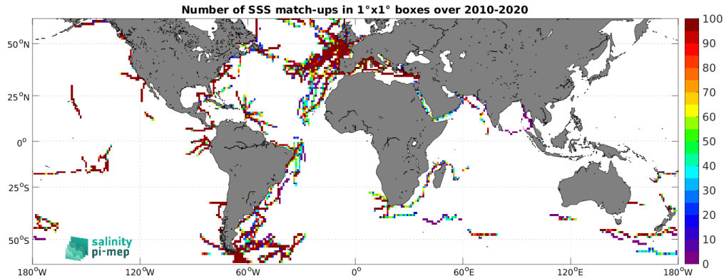
Figure 5: Number of SSS match-ups between TSG (GOSUD-Sailing-ship) SSS and the SMOS SSS L4 v1 - Monthly (CMEMS-CNR) SSS product for the SMOS coastal zone (<800km) 60N-60S Pi-MEP region over 1^{\circ} \times 1^{\circ} boxes and for the full satellite product period.
