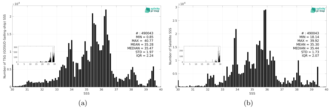
Figure 3: Histograms of SSS from TSG (GOSUD-Sailing-ship) (a) and SMOS SSS L4 v1 - Monthly (CMEMS-CNR) (b) considering all match-up pairs per bins of 0.1 over the SMOS coastal zone (<800km) 60N-60S Pi-MEP region and for the full satellite product period.
