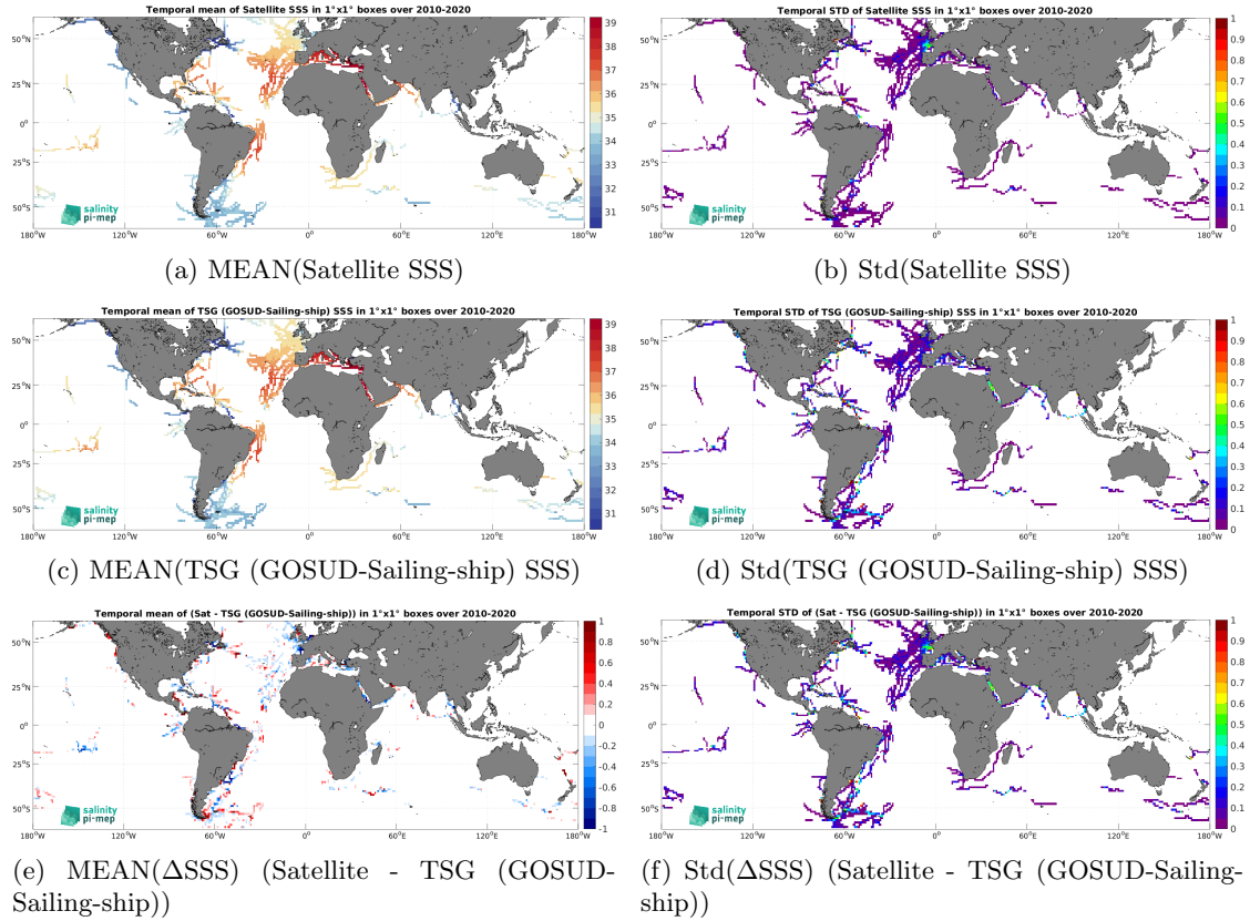
Figure 7: Temporal mean (left) and Std (right) of SSS from SMOS SSS L4 v1 - Monthly (CMEMS-CNR) (top), TSG (GOSUD-Sailing-ship) (middle), and of \Delta SSS (Satellite - TSG (GOSUD-Sailing-ship)). Only match-up pairs are used to generate these maps.
