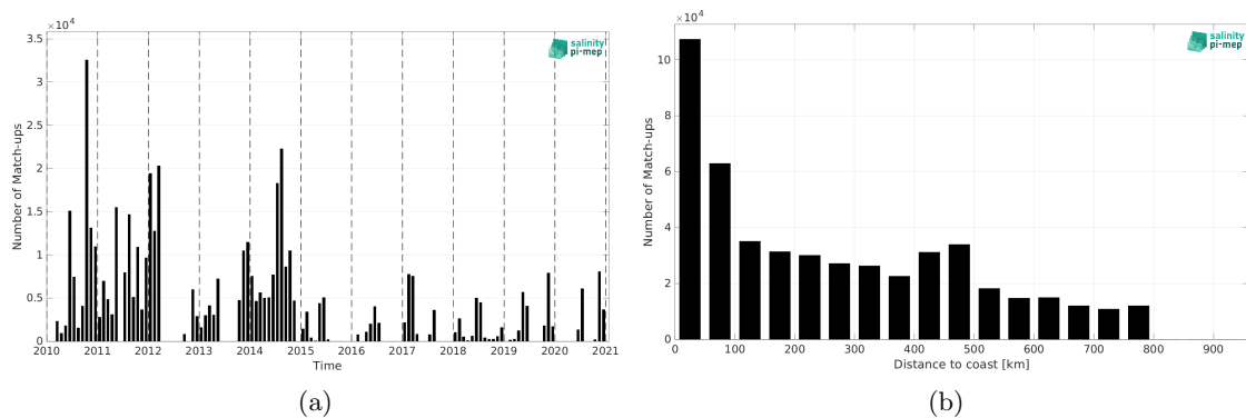
Figure 2: Number of match-ups between TSG (GOSUD-Sailing-ship) and SMOS SSS L4 v1 - Monthly (CMEMS-CNR) SSS as a function of time (a) and as function of the distance to coast (b) over the SMOS coastal zone (<800km) 60N-60S Pi-MEP region and for the full satellite product period.
