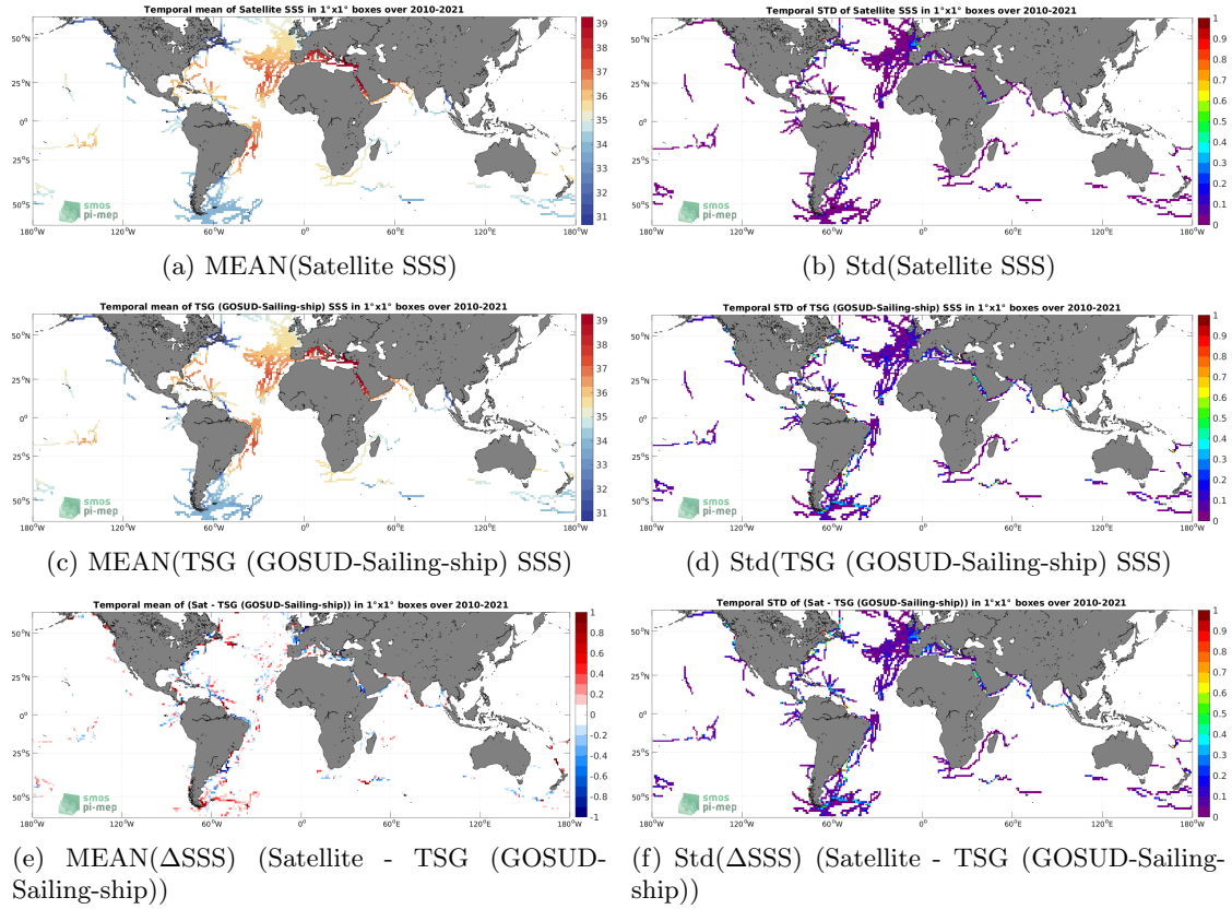
Figure 6: Temporal mean (left) and Std (right) of SSS from SMOS SSS L4 v1 - Monthly (CMEMS-CNR) (top), TSG (GOSUD-Sailing-ship) (middle), and of \Delta SSS (Satellite - TSG (GOSUD-Sailing-ship)). Only match-up pairs are used to generate these maps.
