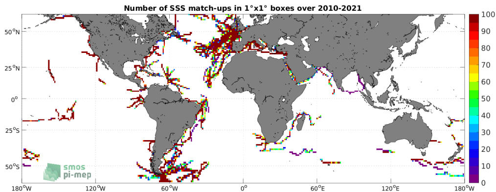
Figure 4: Number of SSS match-ups between TSG (GOSUD-Sailing-ship) SSS and the SMOS SSS L4 v1 - Monthly (CMEMS-CNR) SSS product for the SMOS coastal zone (<800km) 60N-60S Pi-MEP region over 1^\circ \times 1^\circ boxes and for the full satellite product period.
