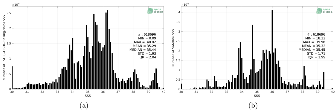
Figure 2: Histograms of SSS from TSG (GOSUD-Sailing-ship) (a) and SMOS SSS L4 v1 - Monthly (CMEMS-CNR) (b) considering all match-up pairs per bins of 0.1 over the SMOS coastal zone (<800km) 60N-60S Pi-MEP region and for the full satellite product period.
