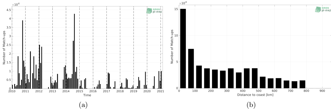
Figure 1: Number of match-ups between TSG (GOSUD-Sailing-ship) and SMOS SSS L4 v1 - Monthly (CMEMS-CNR) SSS as a function of time (a) and as function of the distance to coast (b) over the SMOS coastal zone (<800km) 60N-60S Pi-MEP region and for the full satellite product period.
