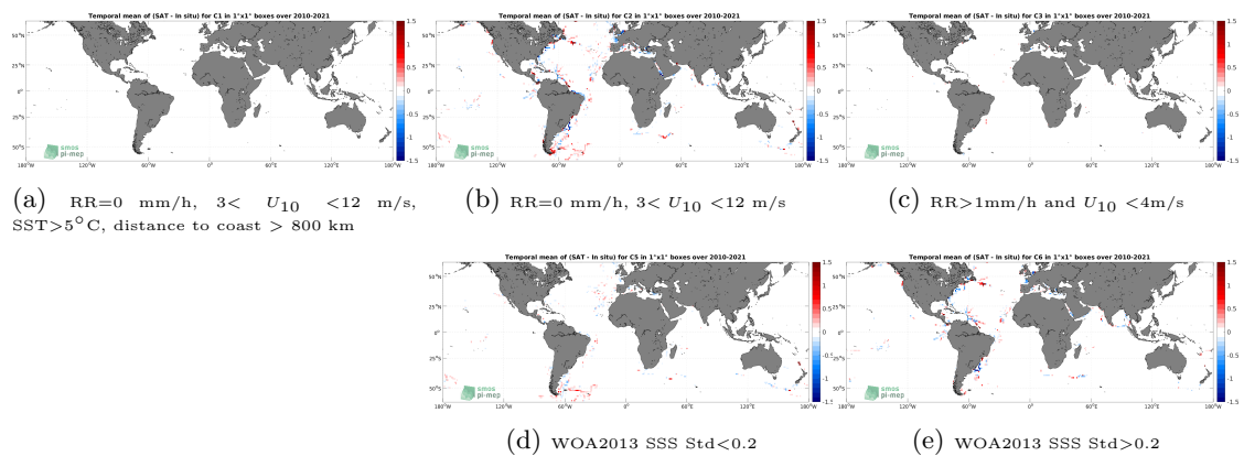
Figure 12: Temporal mean gridded over spatial boxes of size 1^\circ \times 1^\circ of \Delta SSS (SMOS SSS L4 v1 - Monthly (CMEMS-CNR) - TSG (GOSUD-Sailing-ship)) for 5 different subdatasets corresponding to:RR=0 mm/h, 3 < U_{10} < 12 m/s, SST >5^\circ C, distance to coast > 800 km (a), RR=0 mm/h, 3 < U_{10} < 12 m/s (b), RR >1 mm/h and U_{10} < 4 m/s (c), WOA2013 SSS Std <0.2 (d), WOA2013 SSS Std >0.2 (e).
