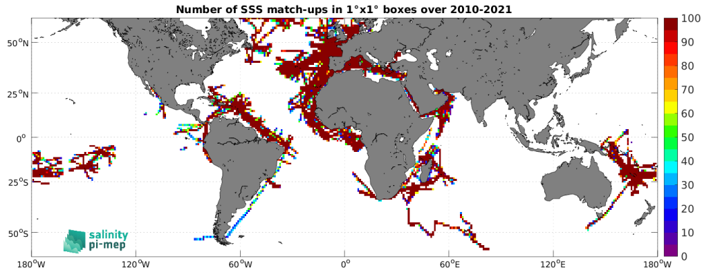
Figure 5: Number of SSS match-ups between TSG (GOSUD-Research-vessel) SSS and the SMOS SSS L4 v1 - Monthly (CMEMS-CNR) SSS product for the SMOS coastal zone (<800km) 60N-60S Pi-MEP region over 1^{\circ} \times 1^{\circ} boxes and for the full satellite product period.
