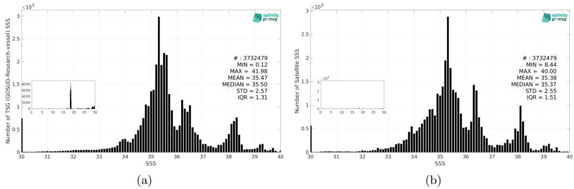
Figure 3: Histograms of SSS from TSG (GOSUD-Research-vessel) (a) and SMOS SSS L4 v1 - Monthly (CMEMS-CNR) (b) considering all match-up pairs per bins of 0.1 over the SMOS coastal zone (<800km) 60N-60S Pi-MEP region and for the full satellite product period.
