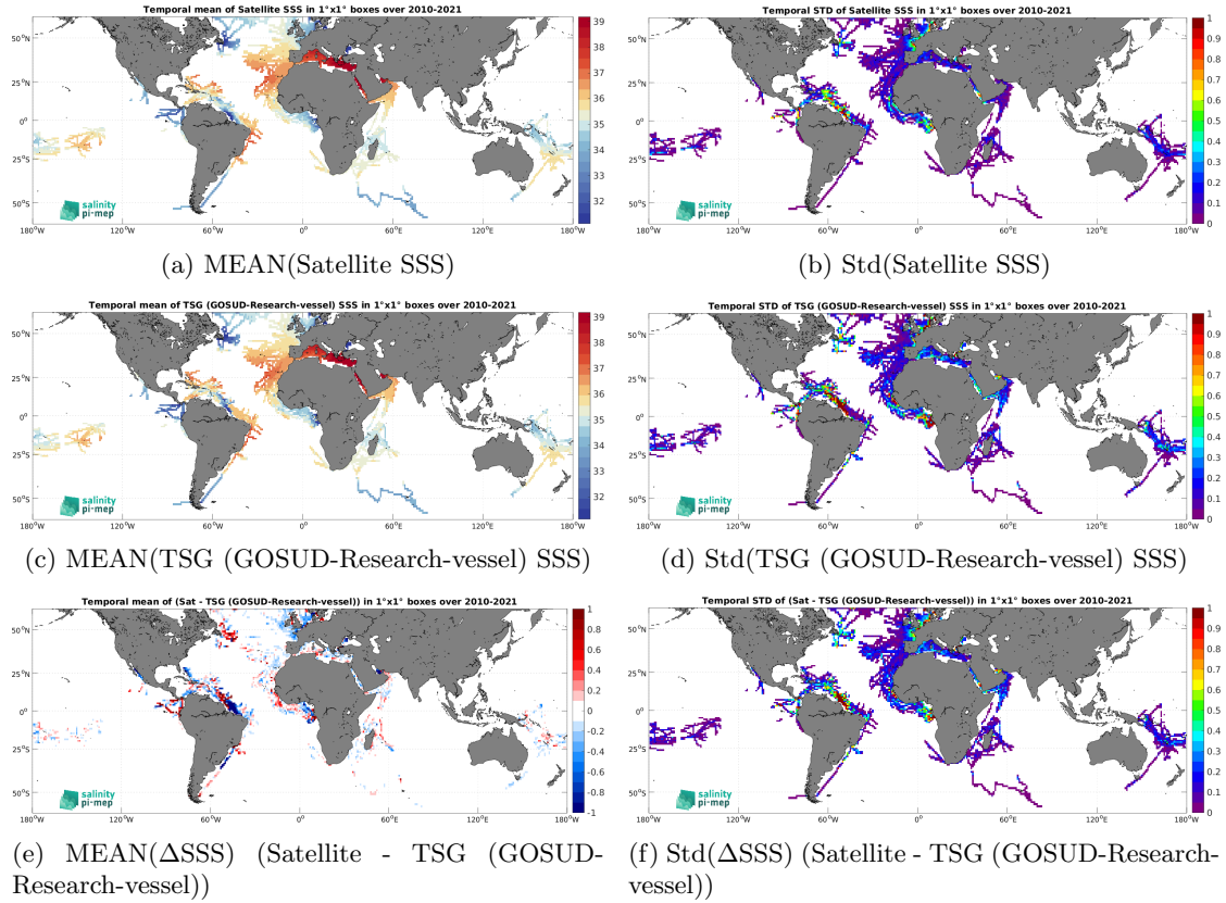
Figure 7: Temporal mean (left) and Std (right) of SSS from SMOS SSS L4 v1 - Monthly (CMEMS-CNR) (top), TSG (GOSUD-Research-vessel) (middle), and of \Delta SSS (Satellite - TSG (GOSUD-Research-vessel)). Only match-up pairs are used to generate these maps.
