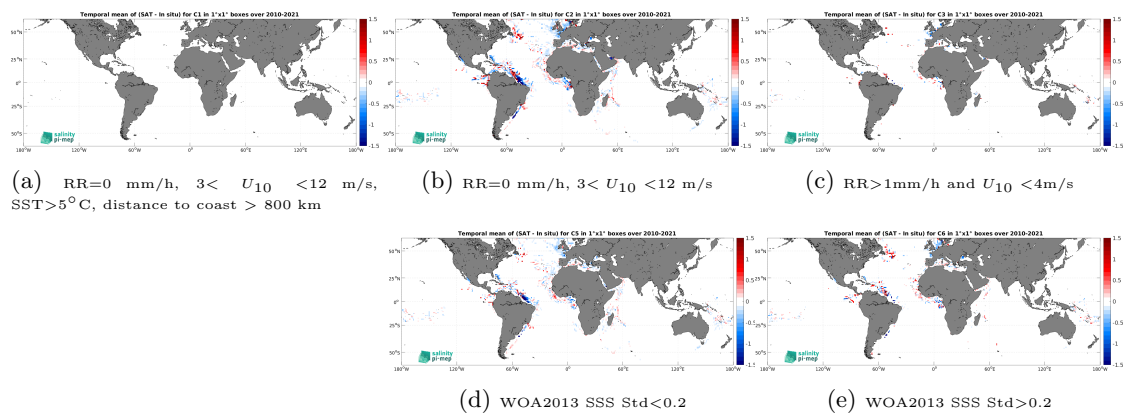
Figure 14: Temporal mean gridded over spatial boxes of size 1^\circ \times 1^\circ of \Delta SSS (SMOS SSS L4 v1 - Monthly (CMEMS-CNR) - TSG (GOSUD-Research-vessel)) for 5 different subdatasets corresponding to:RR=0 mm/h, 3 < U_{10} < 12 m/s, SST >5^\circ C, distance to coast > 800 km (a), RR=0 mm/h, 3 < U_{10} < 12 m/s (b), RR >1 mm/h and U_{10} < 4 m/s (c), WOA2013 SSS Std <0.2 (d), WOA2013 SSS Std >0.2 (e).
