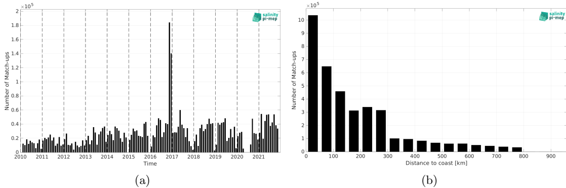
Figure 2: Number of match-ups between TSG (GOSUD-Research-vessel) and SMOS SSS L4 v1 - Monthly (CMEMS-CNR) SSS as a function of time (a) and as function of the distance to coast (b) over the SMOS coastal zone (<800km) 60N-60S Pi-MEP region and for the full satellite product period.
