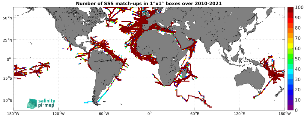
Figure 4: Number of SSS match-ups between TSG (GOSUD-Research-vessel) SSS and the SMOS SSS L4 v1 - Monthly (CMEMS-CNR) SSS product for the SMOS coastal zone (<800km) 60N-60S Pi-MEP region over 1^\circ \times 1^\circ boxes and for the full satellite product period.
