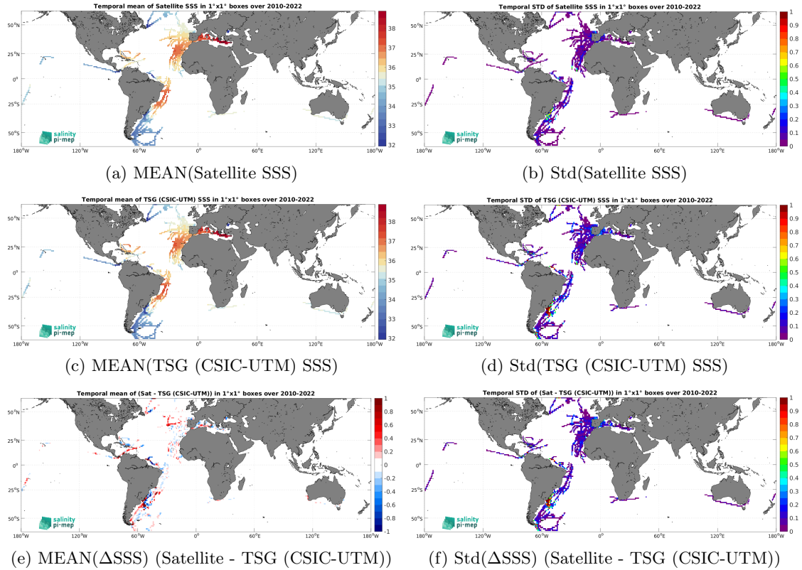
Figure 7: Temporal mean (left) and Std (right) of SSS from SMOS SSS L4 v1 - Monthly (CMEMS-CNR) (top), TSG (CSIC-UTM) (middle), and of \Delta SSS (Satellite - TSG (CSIC-UTM)). Only match-up pairs are used to generate these maps.
