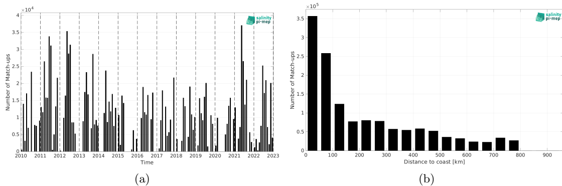
Figure 2: Number of match-ups between TSG (CSIC-UTM) and SMOS SSS L4 v1 - Monthly (CMEMS-CNR) SSS as a function of time (a) and as function of the distance to coast (b) over the SMOS coastal zone (<800km) 60N-60S Pi-MEP region and for the full satellite product period.
