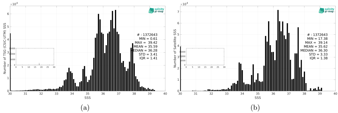
Figure 3: Histograms of SSS from TSG (CSIC-UTM) (a) and SMOS SSS L4 v1 - Monthly (CMEMS-CNR) (b) considering all match-up pairs per bins of 0.1 over the SMOS coastal zone (<800km) 60N-60S Pi-MEP region and for the full satellite product period.
