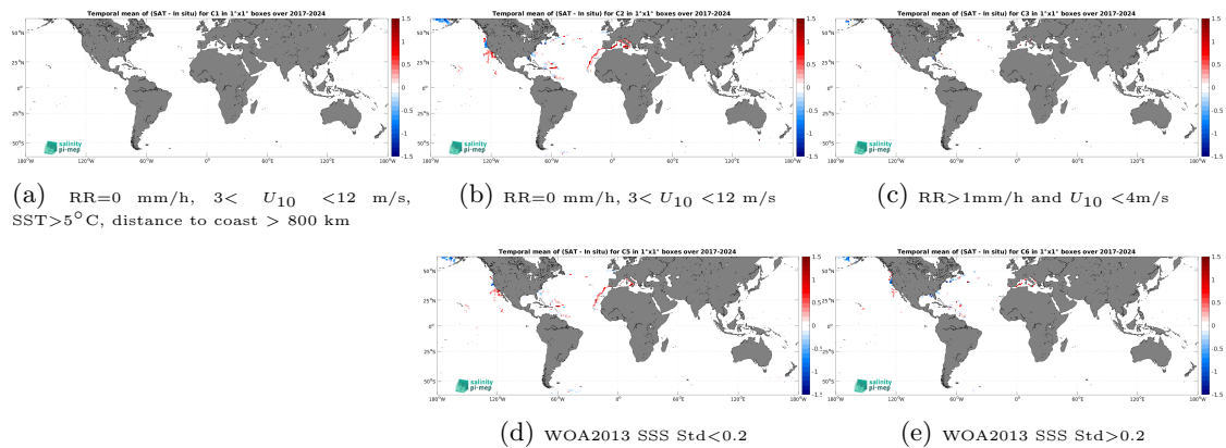
Figure 14: Temporal mean gridded over spatial boxes of size 1^\circ \times 1^\circ of \Delta\text{SSS} (SMOS SSS L4 v1 - Monthly (CMEMS-CNR) - Saildrone) for 5 different subdatasets corresponding to:RR=0 mm/h, 3 < U_{10} < 12 m/s, SST >5^\circ\text{C} , distance to coast > 800 km (a), RR=0 mm/h, 3 < U_{10} < 12 m/s (b), RR >1 mm/h and U_{10} < 4 m/s (c), WOA2013 SSS Std <0.2 (d), WOA2013 SSS Std >0.2 (e).
