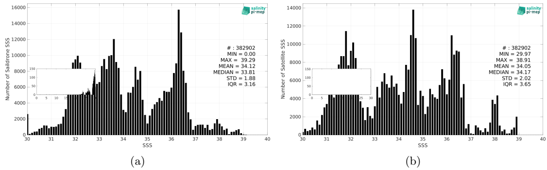
Figure 3: Histograms of SSS from Sairdrone (a) and SMOS SSS L4 v1 - Monthly (CMEMS-CNR) (b) considering all match-up pairs per bins of 0.1 over the SMOS coastal zone (<800km) 60N-60S Pi-MEP region and for the full satellite product period.
