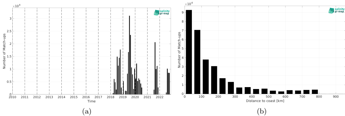
Figure 2: Number of match-ups between Saildrone and SMOS SSS L4 v1 - Monthly (CMEMS-CNR) SSS as a function of time (a) and as function of the distance to coast (b) over the SMOS coastal zone ( < 800\text{km} ) 60N-60S Pi-MEP region and for the full satellite product period.
