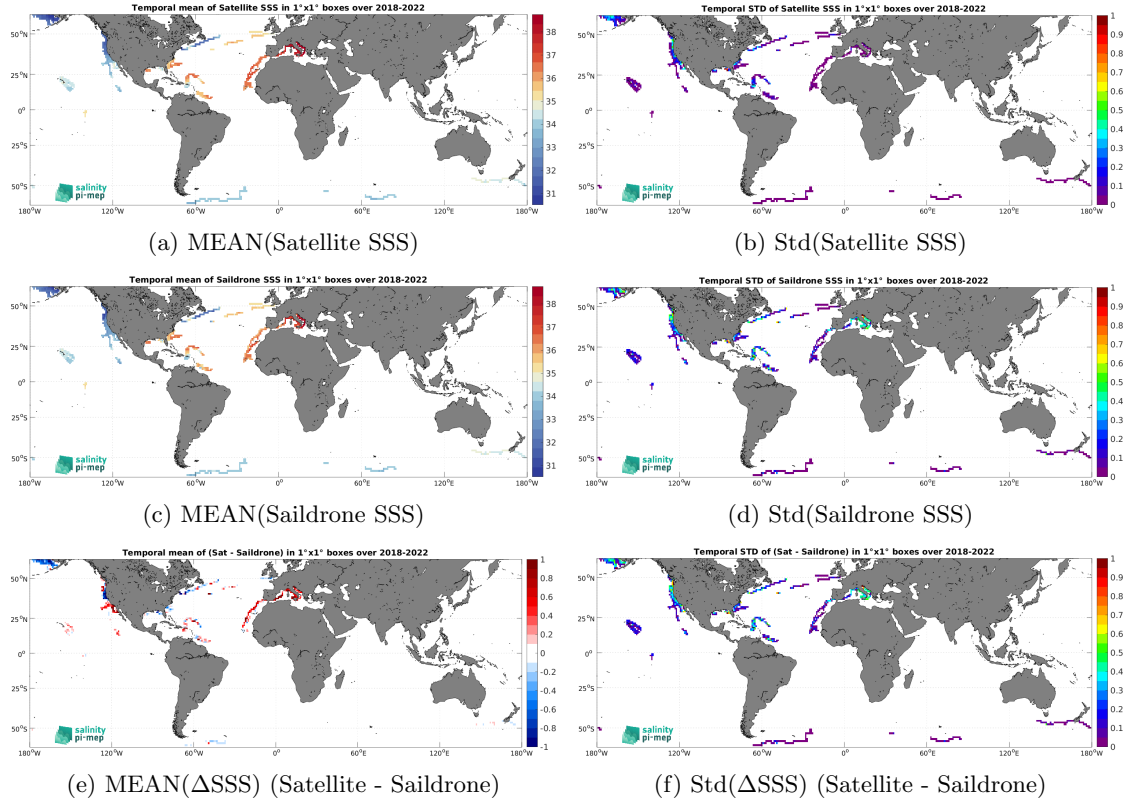
Figure 7: Temporal mean (left) and Std (right) of SSS from SMOS SSS L4 v1 - Monthly (CMEMS-CNR) (top), Saildrone (middle), and of \Delta SSS (Satellite - Saildrone). Only match-up pairs are used to generate these maps.
