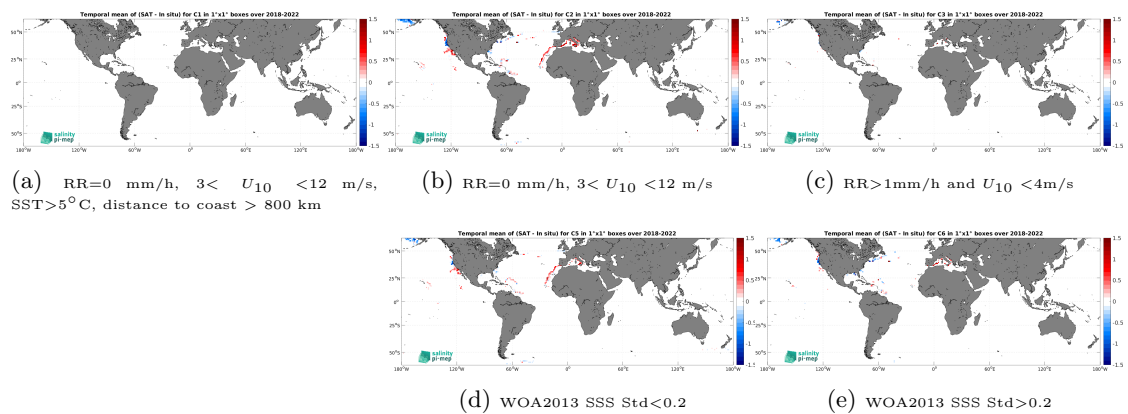
Figure 14: Temporal mean gridded over spatial boxes of size 1^\circ \times 1^\circ of \Delta SSS (SMOS SSS L4 v1 - Monthly (CMEMS-CNR) - Saildrone) for 5 different subdatasets corresponding to:RR=0 mm/h, 3 < U_{10} < 12 m/s, SST >5^\circ\text{C} , distance to coast > 800 km (a), RR=0 mm/h, 3 < U_{10} < 12 m/s (b), RR >1 mm/h and U_{10} < 4 m/s (c), WOA2013 SSS Std <0.2 (d), WOA2013 SSS Std >0.2 (e).
