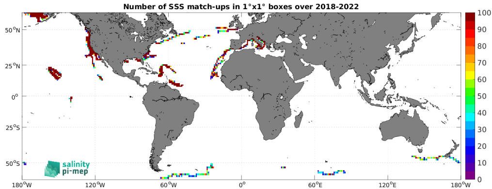
Figure 5: Number of SSS match-ups between Saildrone SSS and the SMOS SSS L4 v1 - Monthly (CMEMS-CNR) SSS product for the SMOS coastal zone (<800km) 60N-60S Pi-MEP region over 1^\circ \times 1^\circ boxes and for the full satellite product period.
