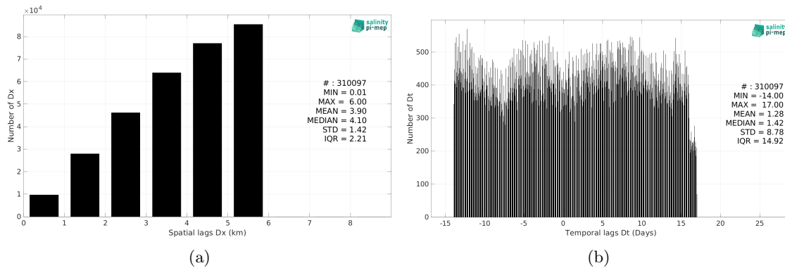
Figure 6: Histograms of the spatial (a) and temporal (b) lags between the location/time of the Saildrone measurement and the date of the corresponding SMOS SSS L4 v1 - Monthly (CMEMS-CNR) SSS pixel.
