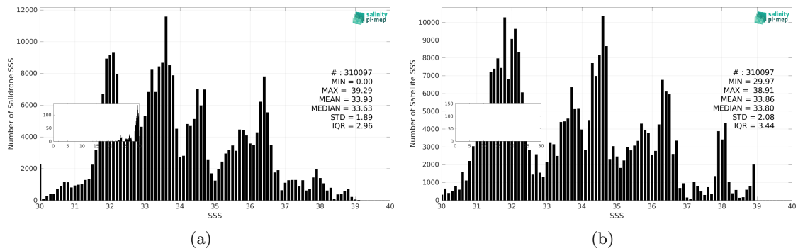
Figure 3: Histograms of SSS from Saildrone (a) and SMOS SSS L4 v1 - Monthly (CMEMS-CNR) (b) considering all match-up pairs per bins of 0.1 over the SMOS coastal zone (<800km) 60N-60S Pi-MEP region and for the full satellite product period.
