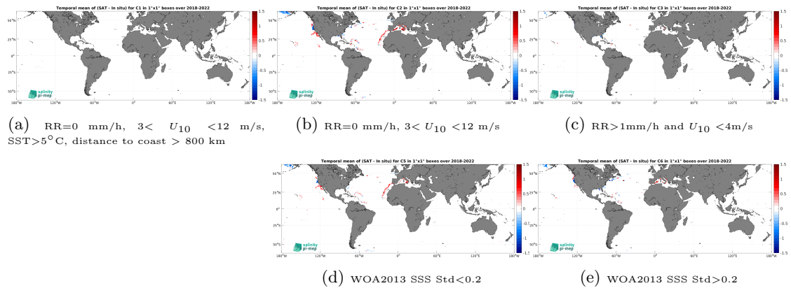
Figure 12: Temporal mean gridded over spatial boxes of size 1^\circ \times 1^\circ of \Delta SSS (SMOS SSS L4 v1 - Monthly (CMEMS-CNR) - Saildrone) for 5 different subdatasets corresponding to:RR=0 mm/h, 3 < U_{10} < 12 m/s, SST >5^\circ C, distance to coast > 800 km (a), RR=0 mm/h, 3 < U_{10} < 12 m/s (b), RR >1 mm/h and U_{10} < 4 m/s (c), WOA2013 SSS Std <0.2 (d), WOA2013 SSS Std >0.2 (e).
