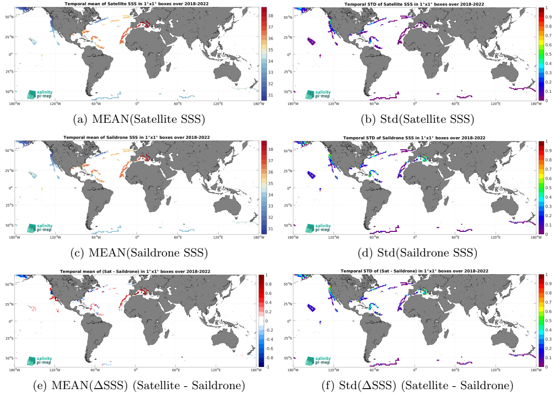
Figure 6: Temporal mean (left) and Std (right) of SSS from SMOS SSS L4 v1 - Monthly (CMEMS-CNR) (top), Saildrone (middle), and of \Delta SSS (Satellite - Saildrone). Only match-up pairs are used to generate these maps.
