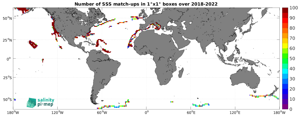
Figure 4: Number of SSS match-ups between Saildrone SSS and the SMOS SSS L4 v1 - Monthly (CMEMS-CNR) SSS product for the SMOS coastal zone (<800km) 60N-60S Pi-MEP region over 1^\circ \times 1^\circ boxes and for the full satellite product period.
