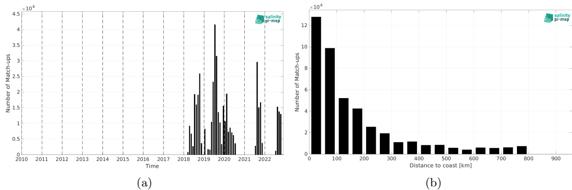
Figure 1: Number of match-ups between Saildrone and SMOS SSS L4 v1 - Monthly (CMEMS-CNR) SSS as a function of time (a) and as function of the distance to coast (b) over the SMOS coastal zone (<800km) 60N-60S Pi-MEP region and for the full satellite product period.
