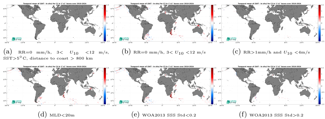
Figure 14: Temporal mean gridded over spatial boxes of size 1^\circ \times 1^\circ of \Delta SSS (SMOS SSS L4 v1 - Monthly (CMEMS-CNR) - Marine mammals) for 6 different subdatasets corresponding to:RR=0 mm/h, 3 < U_{10} < 12 m/s, SST >5^\circ C, distance to coast > 800 km (a), RR=0 mm/h, 3 < U_{10} < 12 m/s (b), RR >1 mm/h and U_{10} < 4 m/s (c),MLD <20 m (d),WOA2013 SSS Std <0.2 (e),WOA2013 SSS Std >0.2 (f).
