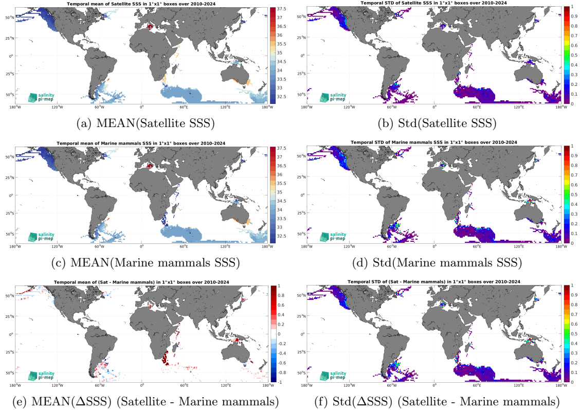
Figure 7: Temporal mean (left) and Std (right) of SSS from SMOS SSS L4 v1 - Monthly (CMEMS-CNR) (top), Marine mammals (middle), and of \Delta SSS (Satellite - Marine mammals). Only match-up pairs are used to generate these maps.
