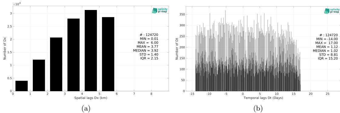
Figure 6: Histograms of the spatial (a) and temporal (b) lags between the location/time of the Marine mammals measurement and the date of the corresponding SMOS SSS L4 v1 - Monthly (CMEMS-CNR) SSS pixel.
