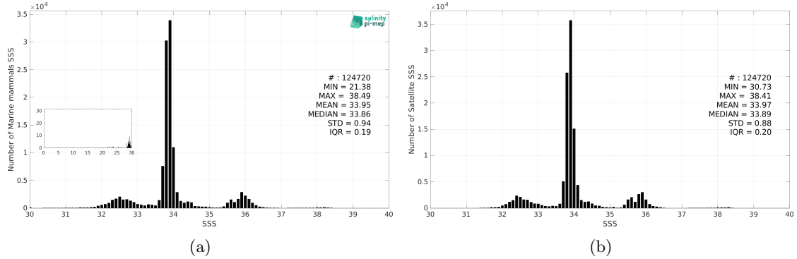
Figure 3: Histograms of SSS from Marine mammals (a) and SMOS SSS L4 v1 - Monthly (CMEMS-CNR) (b) considering all match-up pairs per bins of 0.1 over the SMOS coastal zone (<800km) 60N-60S Pi-MEP region and for the full satellite product period.
