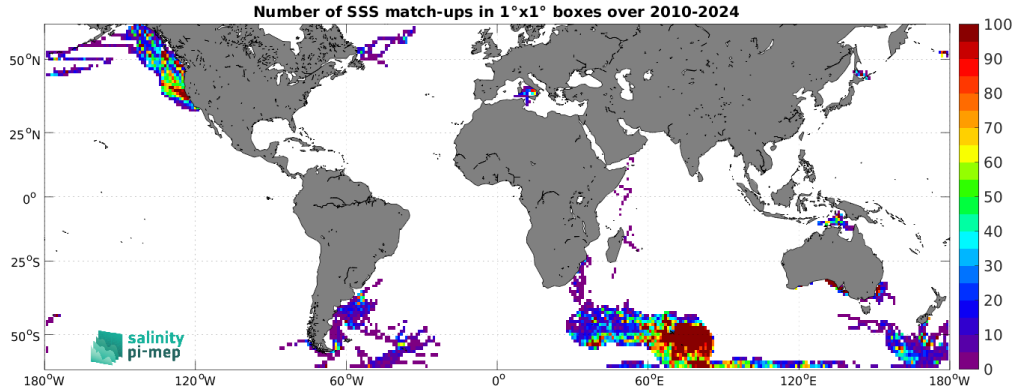
Figure 5: Number of SSS match-ups between Marine mammals SSS and the SMOS SSS L4 v1 - Monthly (CMEMS-CNR) SSS product for the SMOS coastal zone (<800km) 60N-60S Pi-MEP region over 1^{\circ} \times 1^{\circ} boxes and for the full satellite product period.
