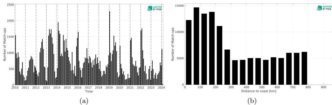
Figure 2: Number of match-ups between Marine mammals and SMOS SSS L4 v1 - Monthly (CMEMS-CNR) SSS as a function of time (a) and as function of the distance to coast (b) over the SMOS coastal zone (<800km) 60N-60S Pi-MEP region and for the full satellite product period.
