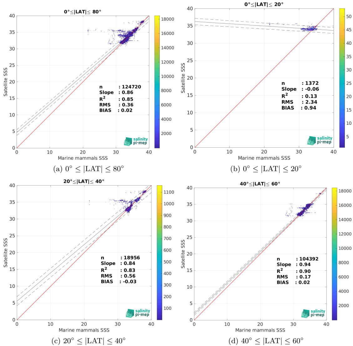
Figure 10: Contour maps of the concentration of SMOS SSS L4 v1 - Monthly (CMEMS-CNR) SSS (y-axis) versus Marine mammals SSS (x-axis) at match-up pairs for different latitude bands. For each plot, the red line shows x=y . The black thin and dashed lines indicate a linear fit through the data cloud and the \pm 95\% confidence levels, respectively. The number match-up pairs n , the slope and R^2 coefficient of the linear fit, the root mean square (RMS) and the mean bias between satellite and in situ data are indicated for each latitude band in each plots.
