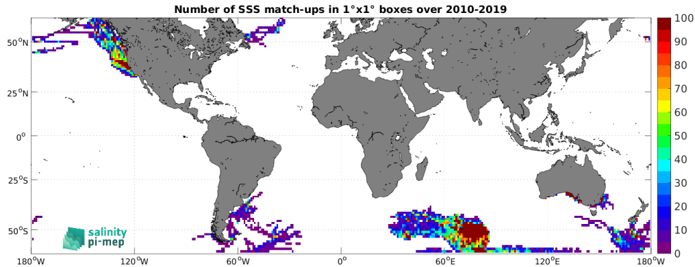
Figure 4: Number of SSS match-ups between Marine mammals SSS and the SMOS SSS L4 v1 - Monthly (CMEMS-CNR) SSS product for the SMOS coastal zone (<800km) 60N-60S Pi-MEP region over 1^{\circ} \times 1^{\circ} boxes and for the full satellite product period.
