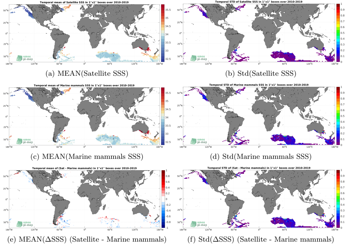
Figure 6: Temporal mean (left) and Std (right) of SSS from SMOS SSS L4 v1 - Monthly (CMEMS-CNR) (top), Marine mammals (middle), and of \Delta SSS (Satellite - Marine mammals). Only match-up pairs are used to generate these maps.
