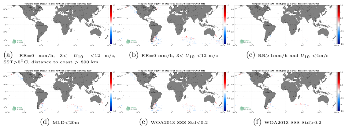
Figure 12: Temporal mean gridded over spatial boxes of size 1^\circ \times 1^\circ of \Delta SSS (SMOS SSS L4 v1 - Monthly (CMEMS-CNR) - Marine mammals) for 6 different subdatasets corresponding to:RR=0 mm/h, 3 < U_{10} < 12 m/s, SST >5^\circ C, distance to coast > 800 km (a), RR=0 mm/h, 3 < U_{10} < 12 m/s (b), RR >1 mm/h and U_{10} < 4 m/s (c),MLD <20 m (d),WOA2013 SSS Std <0.2 (e),WOA2013 SSS Std >0.2 (f).
