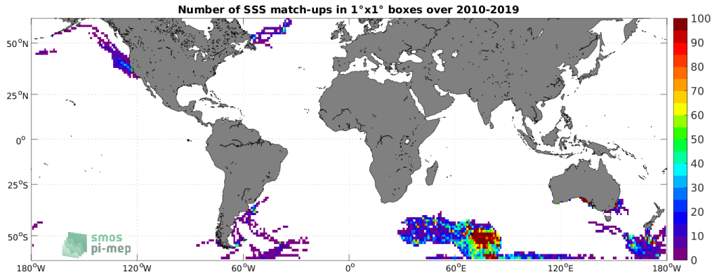
Figure 4: Number of SSS match-ups between Marine mammals SSS and the SMOS SSS L4 v1 - Monthly (CMEMS-CNR) SSS product for the SMOS coastal zone (<800km) 60N-60S Pi-MEP region over 1^\circ \times 1^\circ boxes and for the full satellite product period.
