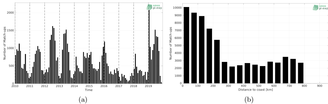
Figure 1: Number of match-ups between Marine mammals and SMOS SSS L4 v1 - Monthly (CMEMS-CNR) SSS as a function of time (a) and as function of the distance to coast (b) over the SMOS coastal zone (<800km) 60N-60S Pi-MEP region and for the full satellite product period.
