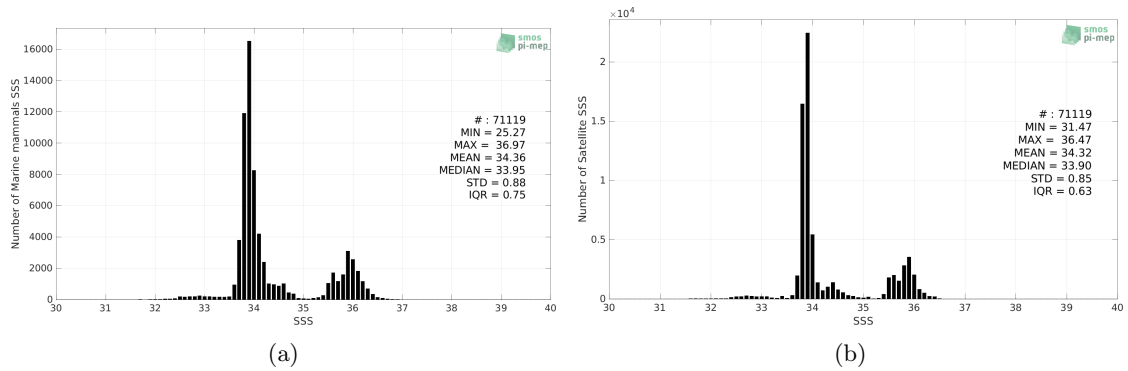
Figure 2: Histograms of SSS from Marine mammals (a) and SMOS SSS L4 v1 - Monthly (CMEMS-CNR) (b) considering all match-up pairs per bins of 0.1 over the SMOS coastal zone (<800km) 60N-60S Pi-MEP region and for the full satellite product period.
