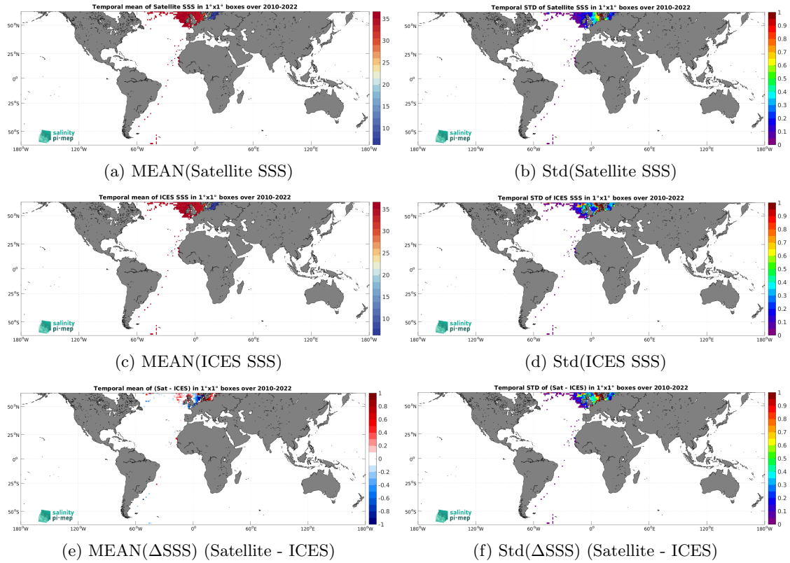
Figure 7: Temporal mean (left) and Std (right) of SSS from SMOS SSS L4 v1 - Monthly (CMEMS-CNR) (top), ICES (middle), and of \Delta SSS (Satellite - ICES). Only match-up pairs are used to generate these maps.
