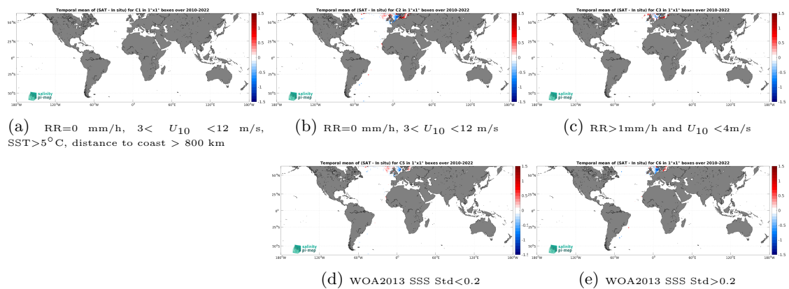
Figure 14: Temporal mean gridded over spatial boxes of size 1^\circ \times 1^\circ of \Delta\text{SSS} (SMOS SSS L4 v1 - Monthly (CMEMS-CNR) - ICES) for 5 different subdatasets corresponding to:RR=0 mm/h, 3 < U_{10} < 12 m/s, SST >5^\circ\text{C} , distance to coast > 800 km (a), RR=0 mm/h, 3 < U_{10} < 12 m/s (b), RR >1 mm/h and U_{10} < 4 m/s (c), WOA2013 SSS Std <0.2 (d), WOA2013 SSS Std >0.2 (e).
