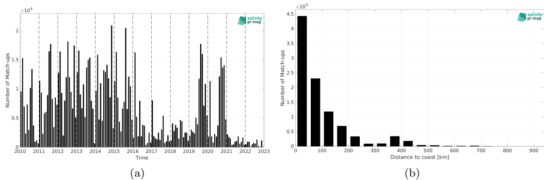
Figure 2: Number of match-ups between ICES and SMOS SSS L4 v1 - Monthly (CMEMS-CNR) SSS as a function of time (a) and as function of the distance to coast (b) over the SMOS coastal zone (<800km) 60N-60S Pi-MEP region and for the full satellite product period.
