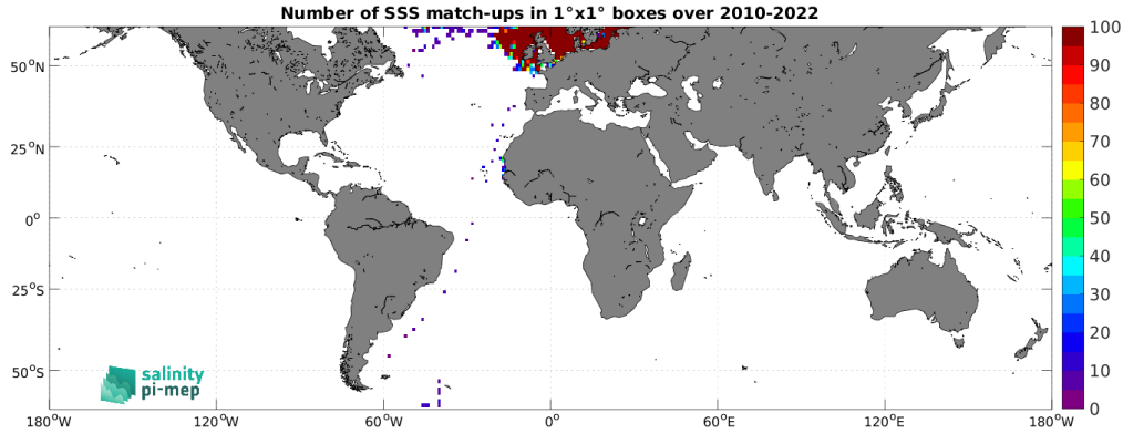
Figure 5: Number of SSS match-ups between ICES SSS and the SMOS SSS L4 v1 - Monthly (CMEMS-CNR) SSS product for the SMOS coastal zone (<800km) 60N-60S Pi-MEP region over 1^\circ \times 1^\circ boxes and for the full satellite product period.
