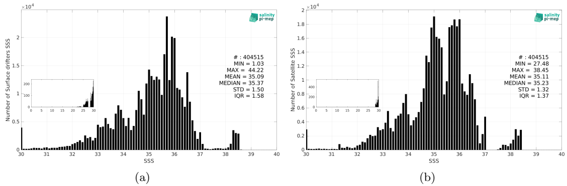
Figure 3: Histograms of SSS from Surface drifters (a) and SMOS SSS L4 v1 - Monthly (CMEMS-CNR) (b) considering all match-up pairs per bins of 0.1 over the SMOS coastal zone (<800km) 60N-60S Pi-MEP region and for the full satellite product period.
