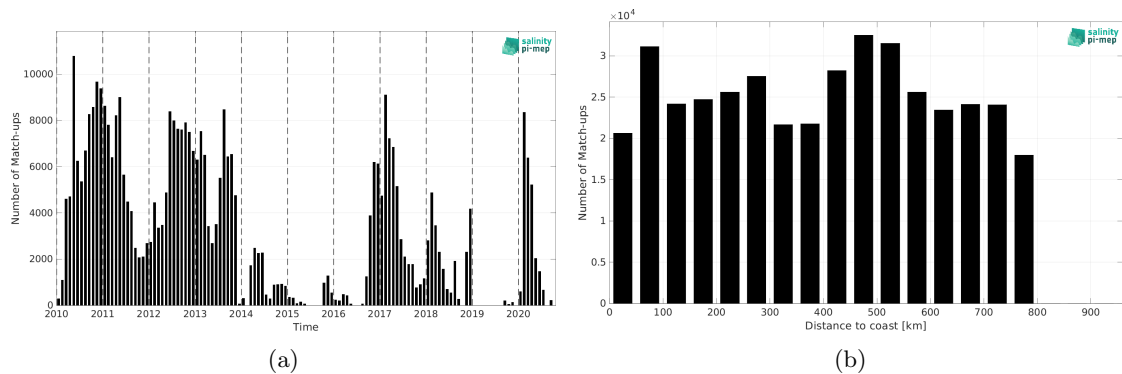
Figure 2: Number of match-ups between Surface drifters and SMOS SSS L4 v1 - Monthly (CMEMS-CNR) SSS as a function of time (a) and as function of the distance to coast (b) over the SMOS coastal zone (<800km) 60N-60S Pi-MEP region and for the full satellite product period.
