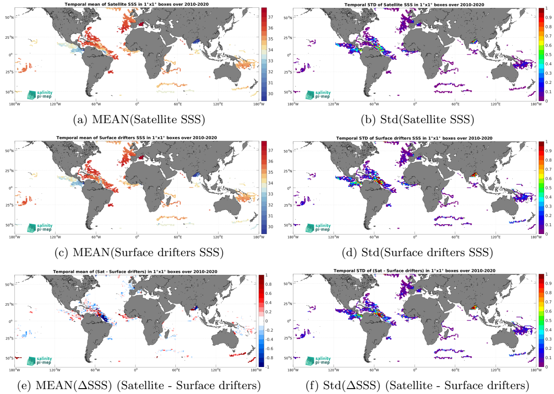
Figure 6: Temporal mean (left) and Std (right) of SSS from SMOS SSS L4 v1 - Monthly (CMEMS-CNR) (top), Surface drifters (middle), and of \Delta SSS (Satellite - Surface drifters). Only match-up pairs are used to generate these maps.
