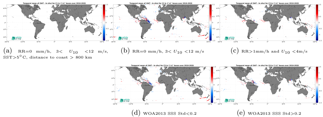
Figure 13: Temporal mean gridded over spatial boxes of size 1^\circ \times 1^\circ of \Delta SSS (SMOS SSS L4 v1 - Monthly (CMEMS-CNR) - Surface drifters) for 5 different subdatasets corresponding to:RR=0 mm/h, 3 < U_{10} < 12 m/s, SST >5^\circ C, distance to coast > 800 km (a), RR=0 mm/h, 3 < U_{10} < 12 m/s (b), RR >1 mm/h and U_{10} < 4 m/s (c), WOA2013 SSS Std <0.2 (d), WOA2013 SSS Std >0.2 (e).
