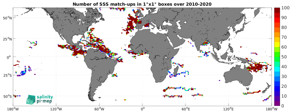
Figure 4: Number of SSS match-ups between Surface drifters SSS and the SMOS SSS L4 v1 - Monthly (CMEMS-CNR) SSS product for the SMOS coastal zone (<800km) 60N-60S Pi-MEP region over 1^\circ \times 1^\circ boxes and for the full satellite product period.
