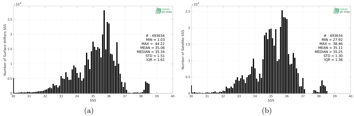
Figure 2: Histograms of SSS from Surface drifters (a) and SMOS SSS L4 v1 - Monthly (CMEMS-CNR) (b) considering all match-up pairs per bins of 0.1 over the SMOS coastal zone (<800km) 60N-60S Pi-MEP region and for the full satellite product period.
