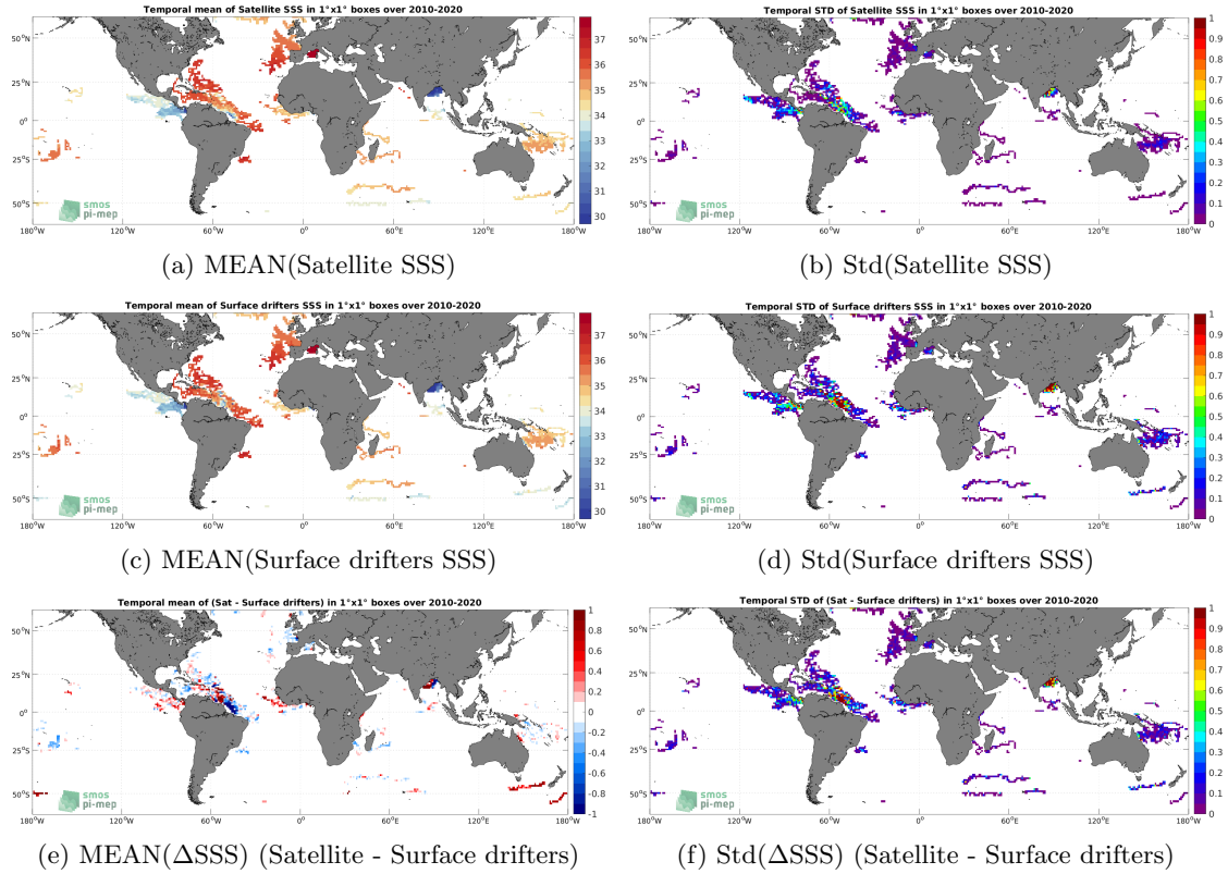
Figure 5: Temporal mean (left) and Std (right) of SSS from SMOS SSS L4 v1 - Monthly (CMEMS-CNR) (top), Surface drifters (middle), and of \Delta SSS (Satellite - Surface drifters). Only match-up pairs are used to generate these maps.
