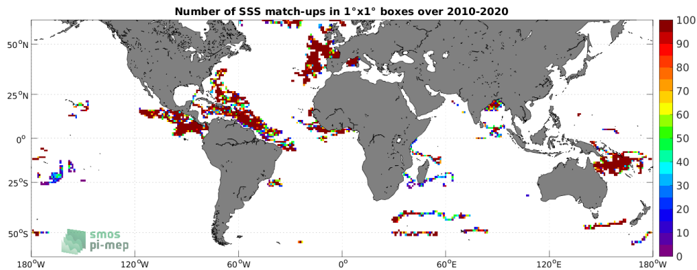
Figure 3: Number of SSS match-ups between Surface drifters SSS and the SMOS SSS L4 v1 - Monthly (CMEMS-CNR) SSS product for the SMOS coastal zone (<800km) 60N-60S Pi-MEP region over 1^\circ \times 1^\circ boxes and for the full satellite product period.
