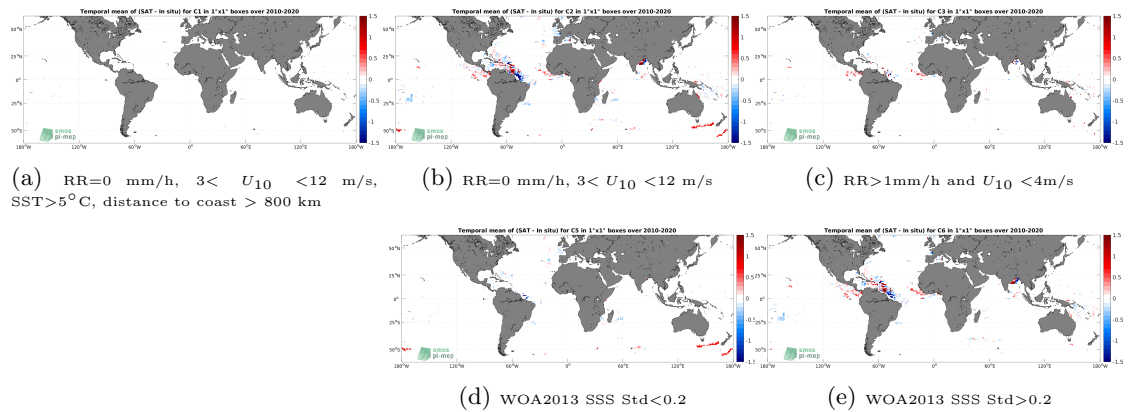
Figure 11: Temporal mean gridded over spatial boxes of size 1^\circ \times 1^\circ of \Delta SSS (SMOS SSS L4 v1 - Monthly (CMEMS-CNR) - Surface drifters) for 5 different subdatasets corresponding to:RR=0 mm/h, 3 < U_{10} < 12 m/s, SST >5^\circ C, distance to coast > 800 km (a), RR=0 mm/h, 3 < U_{10} < 12 m/s (b), RR >1 mm/h and U_{10} < 4 m/s (c), WOA2013 SSS Std <0.2 (d), WOA2013 SSS Std >0.2 (e).
