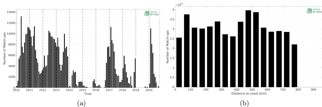
Figure 1: Number of match-ups between Surface drifters and SMOS SSS L4 v1 - Monthly (CMEMS-CNR) SSS as a function of time (a) and as function of the distance to coast (b) over the SMOS coastal zone (<800km) 60N-60S Pi-MEP region and for the full satellite product period.
