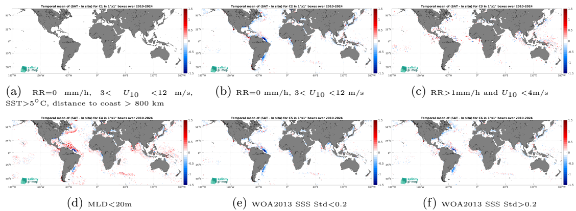
Figure 14: Temporal mean gridded over spatial boxes of size 1^\circ \times 1^\circ of \Delta SSS (SMOS SSS L4 v1 - Monthly (CMEMS-CNR) - Argo) for 6 different subdatasets corresponding to:RR=0 mm/h, 3 < U_{10} < 12 m/s, SST>5°C, distance to coast > 800 km (a), RR=0 mm/h, 3 < U_{10} < 12 m/s (b), RR>1mm/h and U_{10} < 4 m/s (c),MLD<20m (d),WOA2013 SSS Std<0.2 (e),WOA2013 SSS Std>0.2 (f).
