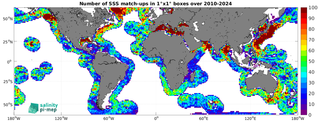
Figure 5: Number of SSS match-ups between Argo SSS and the SMOS SSS L4 v1 - Monthly (CMEMS-CNR) SSS product for the SMOS coastal zone (<800km) 60N-60S Pi-MEP region over 1^{\circ} \times 1^{\circ} boxes and for the full satellite product period.
