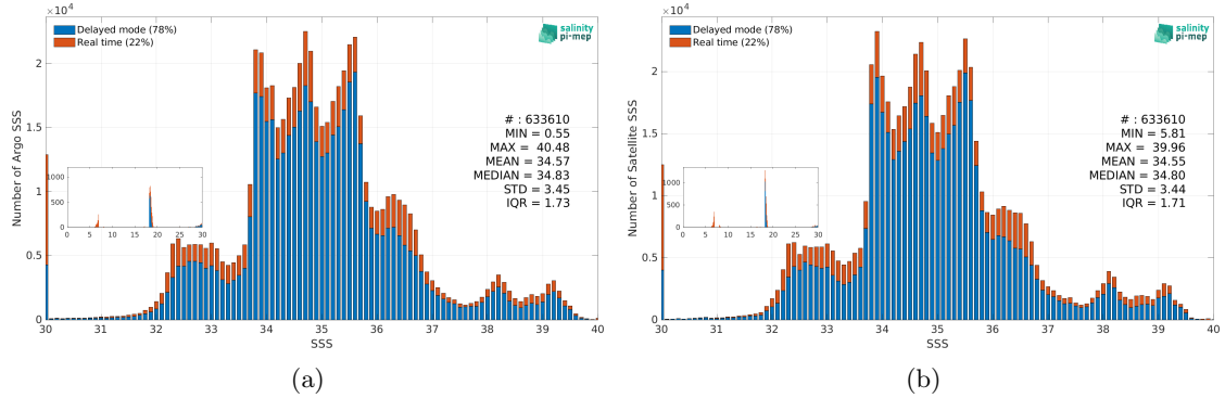
Figure 3: Histograms of SSS from Argo (a) and SMOS SSS L4 v1 - Monthly (CMEMS-CNR) (b) considering all match-up pairs per bins of 0.1 over the SMOS coastal zone (<800km) 60N-60S Pi-MEP region and for the full satellite product period.
