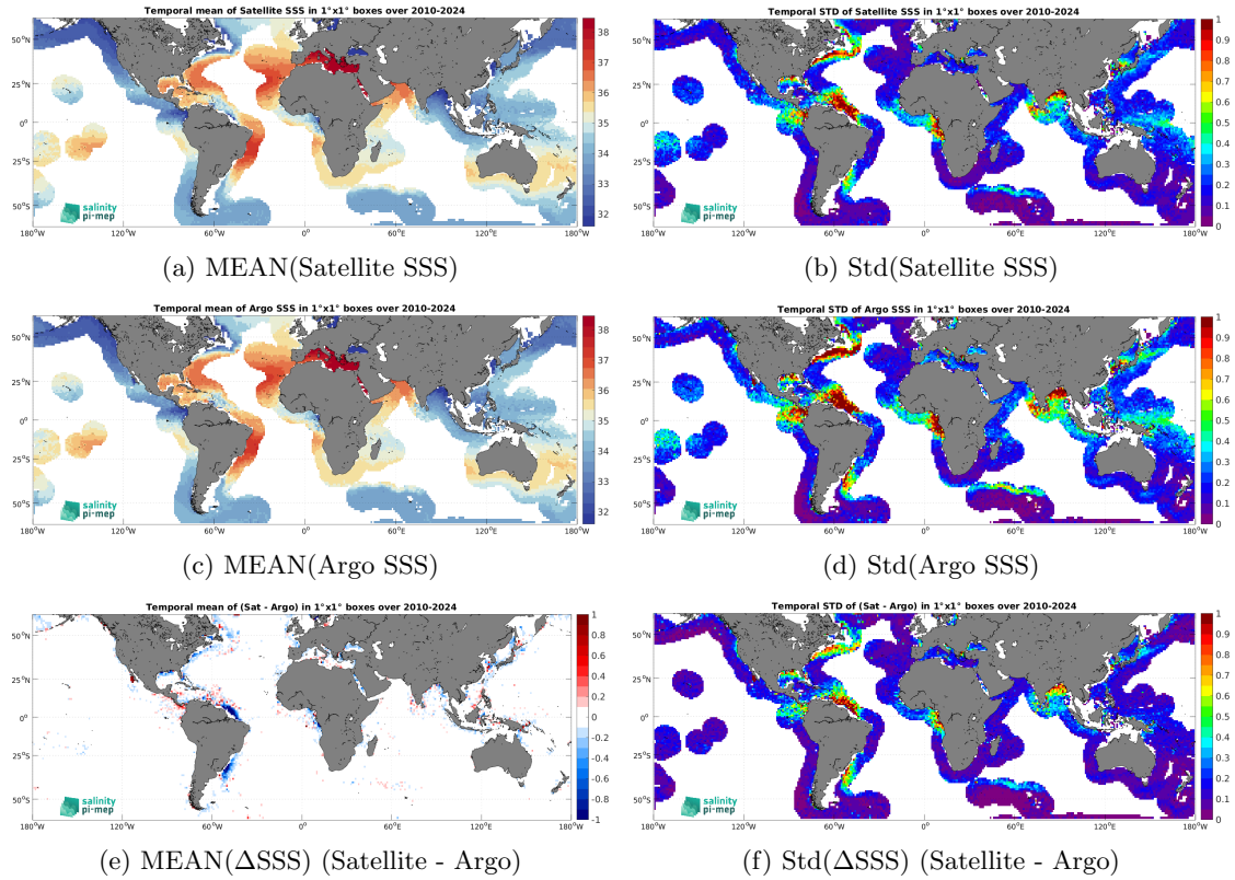
Figure 7: Temporal mean (left) and Std (right) of SSS from SMOS SSS L4 v1 - Monthly (CMEMS-CNR) (top), Argo (middle), and of \Delta SSS (Satellite - Argo). Only match-up pairs are used to generate these maps.
