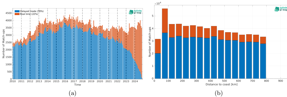
Figure 2: Number of match-ups between Argo and SMOS SSS L4 v1 - Monthly (CMEMS-CNR) SSS as a function of time (a) and as function of the distance to coast (b) over the SMOS coastal zone ( < 800\text{km} ) 60N-60S Pi-MEP region and for the full satellite product period.
