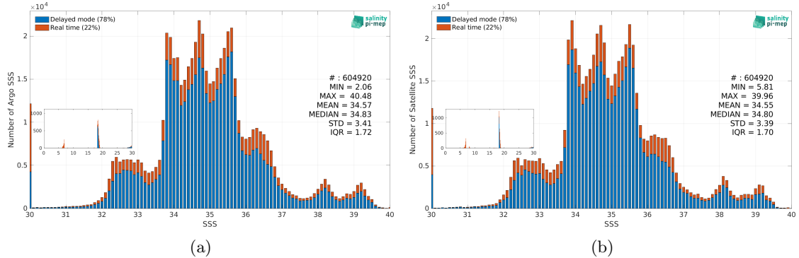
Figure 3: Histograms of SSS from Argo (a) and SMOS SSS L4 v1 - Monthly (CMEMS-CNR) (b) considering all match-up pairs per bins of 0.1 over the SMOS coastal zone (<800km) 60N-60S Pi-MEP region and for the full satellite product period.
