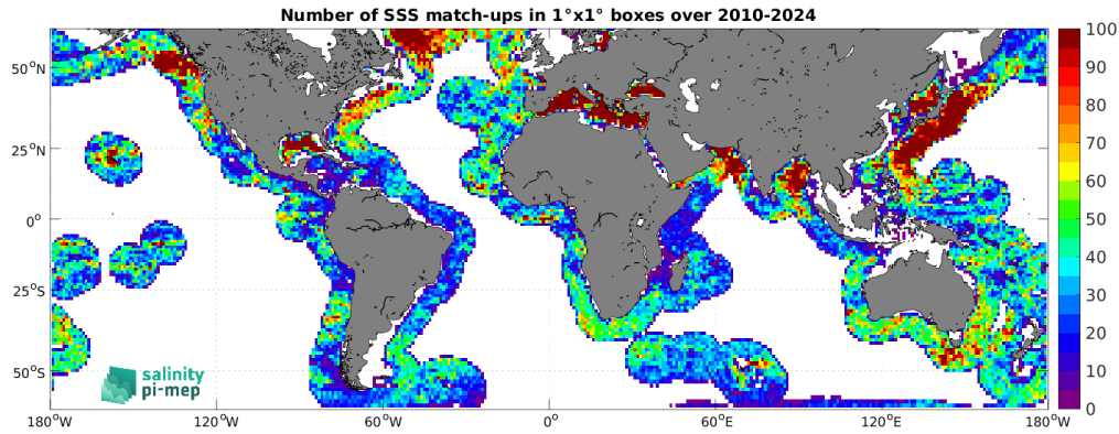
Figure 5: Number of SSS match-ups between Argo SSS and the SMOS SSS L4 v1 - Monthly (CMEMS-CNR) SSS product for the SMOS coastal zone (<800km) 60N-60S Pi-MEP region over 1^\circ \times 1^\circ boxes and for the full satellite product period.
