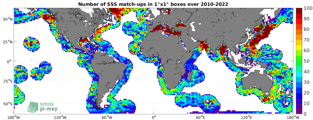
Figure 4: Number of SSS match-ups between Argo SSS and the SMOS SSS L4 v1 - Monthly (CMEMS-CNR) SSS product for the SMOS coastal zone (<800km) 60N-60S Pi-MEP region over 1^\circ \times 1^\circ boxes and for the full satellite product period.
