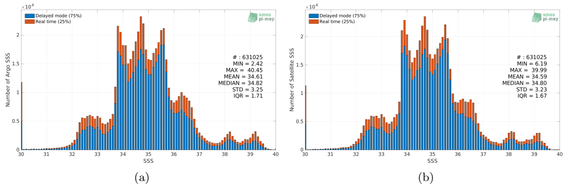
Figure 2: Histograms of SSS from Argo (a) and SMOS SSS L4 v1 - Monthly (CMEMS-CNR) (b) considering all match-up pairs per bins of 0.1 over the SMOS coastal zone (<800km) 60N-60S Pi-MEP region and for the full satellite product period.
