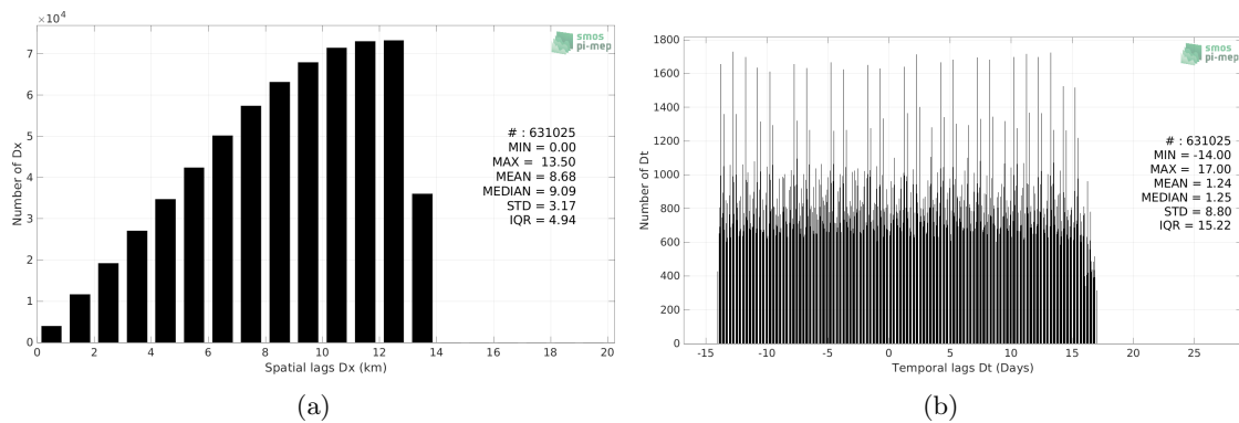
Figure 5: Histograms of the spatial (a) and temporal (b) lags between the location/time of the Argo measurement and the date of the corresponding SMOS SSS L4 v1 - Monthly (CMEMS-CNR) SSS pixel.
