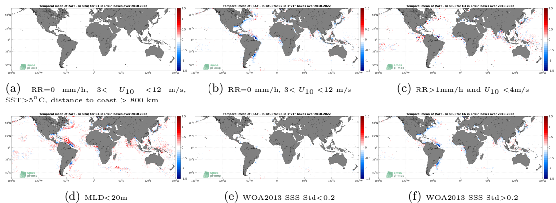
Figure 12: Temporal mean gridded over spatial boxes of size 1^\circ \times 1^\circ of \Delta SSS (SMOS SSS L4 v1 - Monthly (CMEMS-CNR) - Argo) for 6 different subdatasets corresponding to:RR=0 mm/h, 3 < U_{10} < 12 m/s, SST > 5^\circ\text{C} , distance to coast > 800 km (a), RR=0 mm/h, 3 < U_{10} < 12 m/s (b), RR > 1 mm/h and U_{10} < 4 m/s (c),MLD < 20 m (d),WOA2013 SSS Std < 0.2 (e),WOA2013 SSS Std > 0.2 (f).
