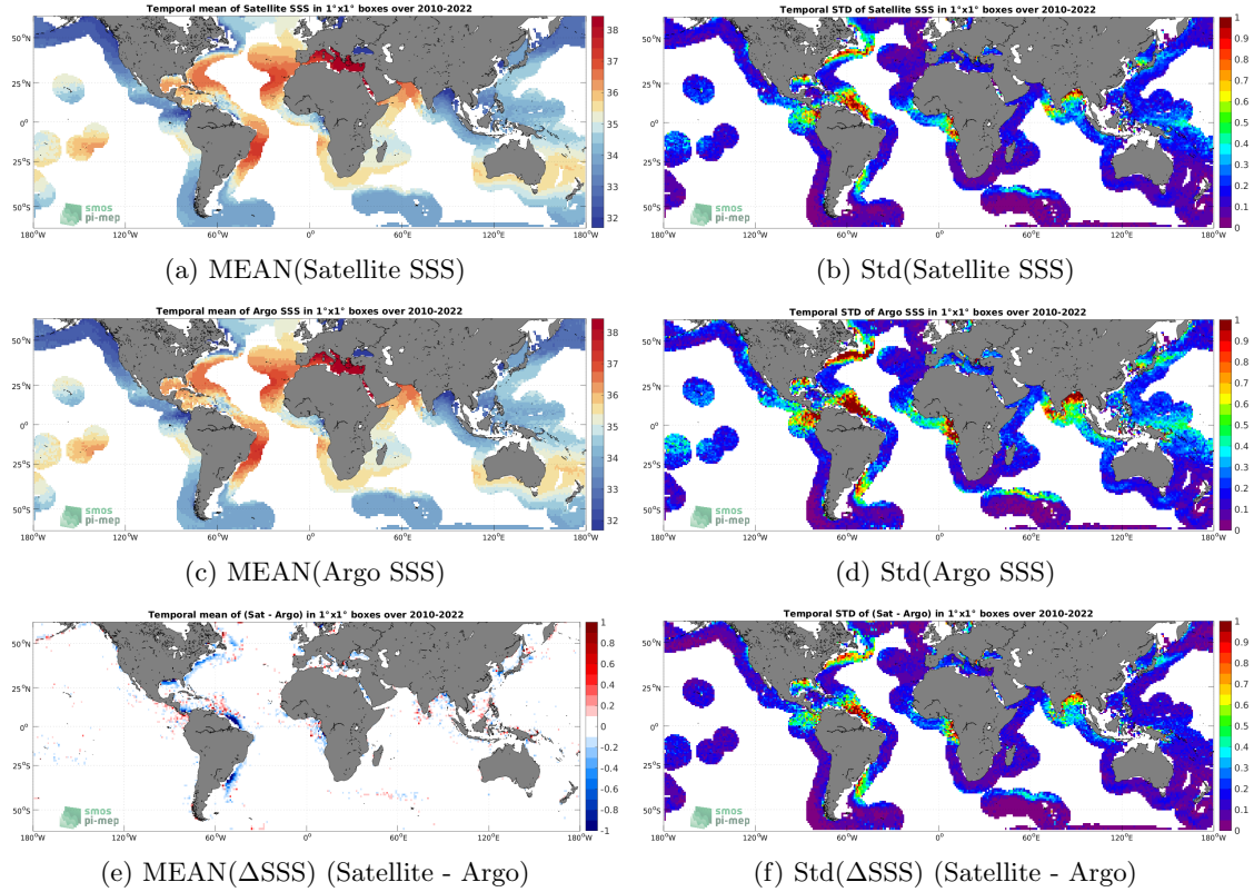
Figure 6: Temporal mean (left) and Std (right) of SSS from SMOS SSS L4 v1 - Monthly (CMEMS-CNR) (top), Argo (middle), and of \Delta SSS (Satellite - Argo). Only match-up pairs are used to generate these maps.
