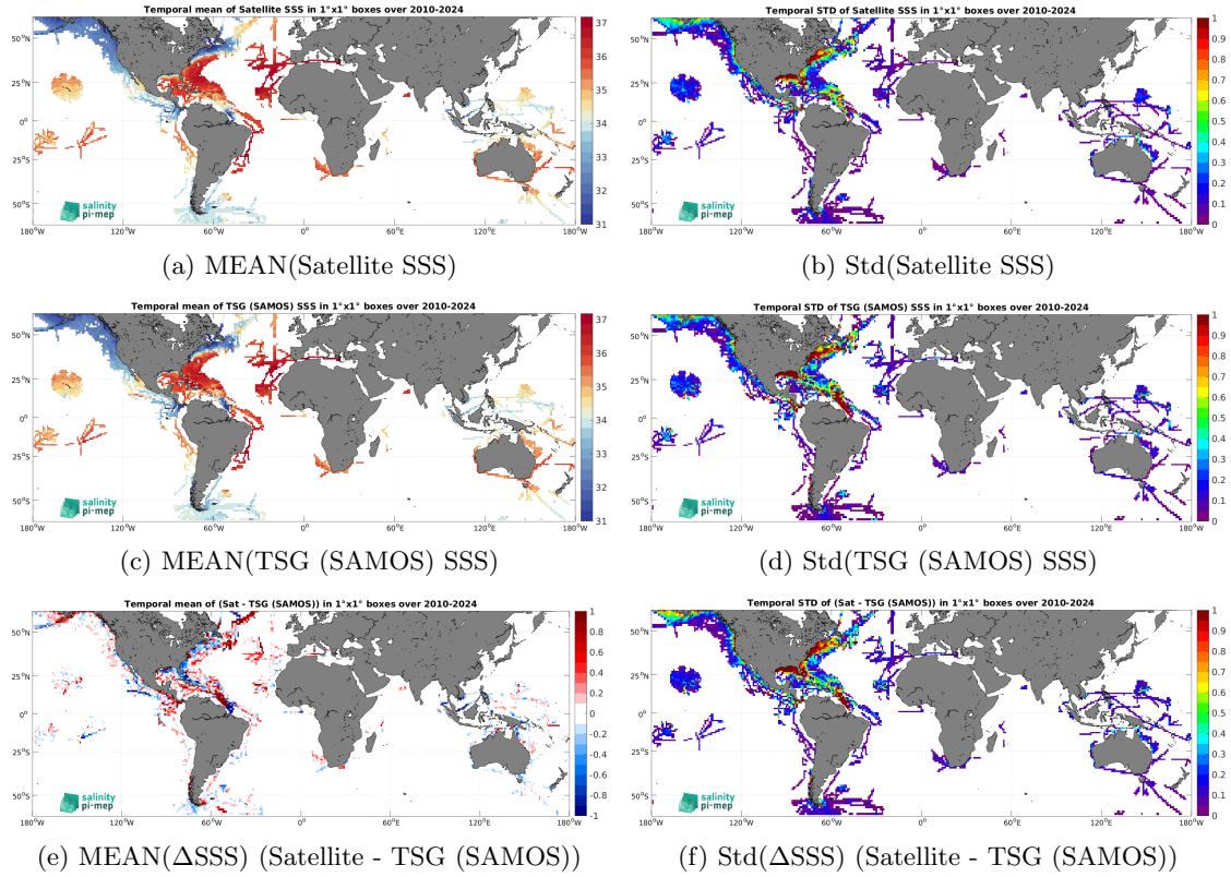
Figure 7: Temporal mean (left) and Std (right) of SSS from SMOS SSS L4 v1 - Daily (CMEMS-CNR) (top), TSG (SAMOS) (middle), and of \Delta SSS (Satellite - TSG (SAMOS)). Only match-up pairs are used to generate these maps.
