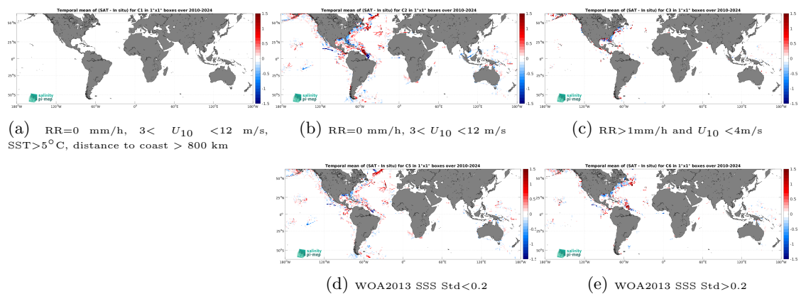
Figure 14: Temporal mean gridded over spatial boxes of size 1^\circ \times 1^\circ of \Delta SSS (SMOS SSS L4 v1 - Daily (CMEMS-CNR) - TSG (SAMOS)) for 5 different subdatasets corresponding to:RR=0 mm/h, 3 < U_{10} < 12 m/s, SST >5^\circ\text{C} , distance to coast > 800 km (a), RR=0 mm/h, 3 < U_{10} < 12 m/s (b), RR >1 mm/h and U_{10} < 4 m/s (c), WOA2013 SSS Std <0.2 (d), WOA2013 SSS Std >0.2 (e).
