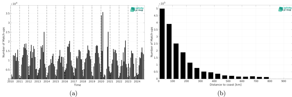
Figure 2: Number of match-ups between TSG (SAMOS) and SMOS SSS L4 v1 - Daily (CMEMS-CNR) SSS as a function of time (a) and as function of the distance to coast (b) over the SMOS coastal zone (<800km) 60N-60S Pi-MEP region and for the full satellite product period.
