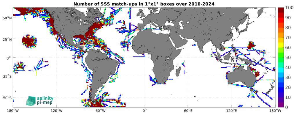
Figure 5: Number of SSS match-ups between TSG (SAMOS) SSS and the SMOS SSS L4 v1 - Daily (CMEMS-CNR) SSS product for the SMOS coastal zone (<800km) 60N-60S Pi-MEP region over 1^{\circ} \times 1^{\circ} boxes and for the full satellite product period.
