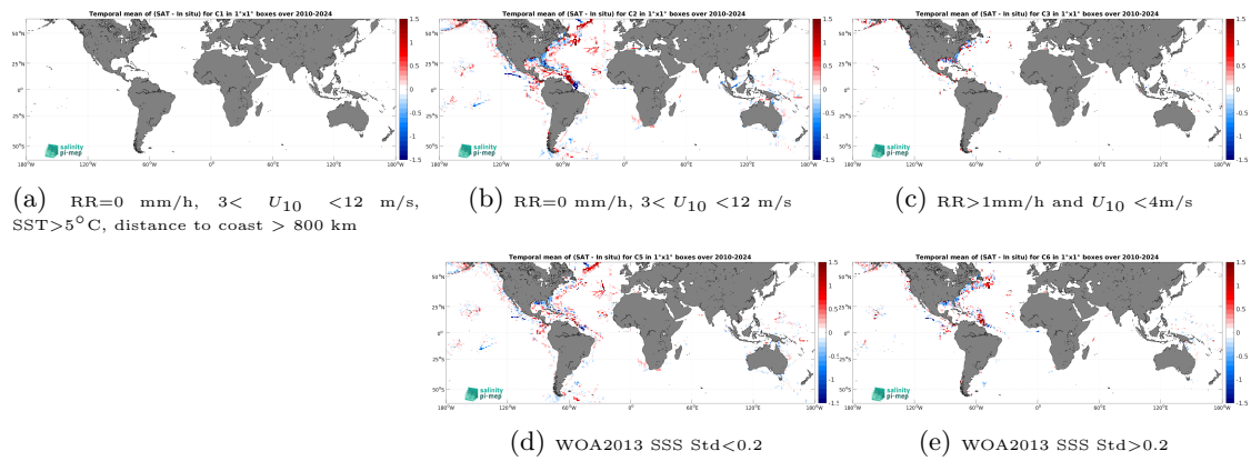
Figure 14: Temporal mean gridded over spatial boxes of size 1^\circ \times 1^\circ of \Delta\text{SSS} (SMOS SSS L4 v1 - Daily (CMEMS-CNR) - TSG (SAMOS)) for 5 different subdatasets corresponding to: RR=0 mm/h, 3 < U_{10} < 12 m/s, SST > 5°C, distance to coast > 800 km (a), RR=0 mm/h, 3 < U_{10} < 12 m/s (b), RR > 1mm/h and U_{10} < 4 m/s (c), WOA2013 SSS Std < 0.2 (d), WOA2013 SSS Std > 0.2 (e).
