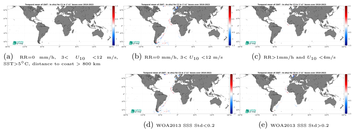
Figure 14: Temporal mean gridded over spatial boxes of size 1^\circ \times 1^\circ of \Delta SSS (SMOS SSS L4 v1 - Daily (CMEMS-CNR) - TSG (Polarstern)) for 5 different subdatasets corresponding to:RR=0 mm/h, 3 < U_{10} < 12 m/s, SST >5^\circ\text{C} , distance to coast > 800 km (a), RR=0 mm/h, 3 < U_{10} < 12 m/s (b), RR >1 mm/h and U_{10} < 4 m/s (c), WOA2013 SSS Std <0.2 (d), WOA2013 SSS Std >0.2 (e).
