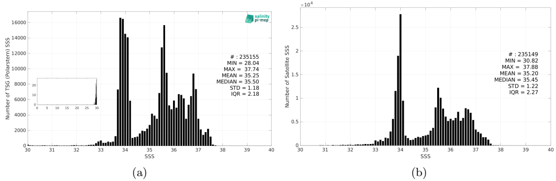
Figure 3: Histograms of SSS from TSG (Polarstern) (a) and SMOS SSS L4 v1 - Daily (CMEMS-CNR) (b) considering all match-up pairs per bins of 0.1 over the SMOS coastal zone (<800km) 60N-60S Pi-MEP region and for the full satellite product period.
