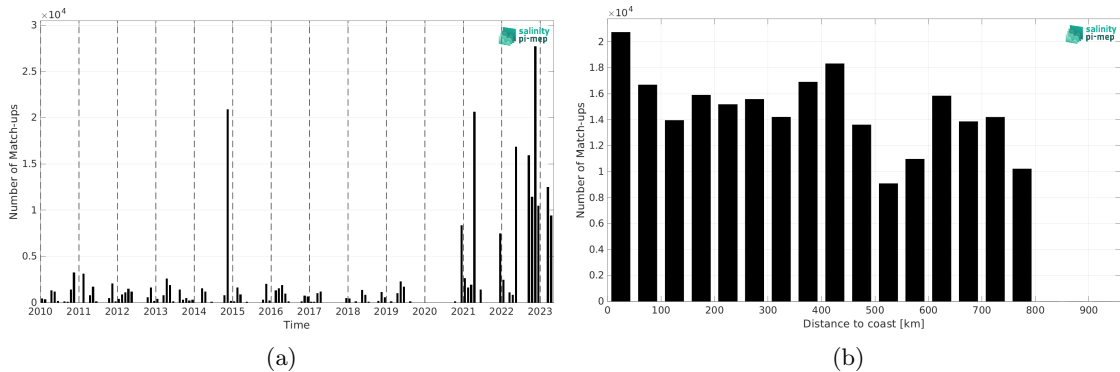
Figure 2: Number of match-ups between TSG (Polarstern) and SMOS SSS L4 v1 - Daily (CMEMS-CNR) SSS as a function of time (a) and as function of the distance to coast (b) over the SMOS coastal zone (<800km) 60N-60S Pi-MEP region and for the full satellite product period.
