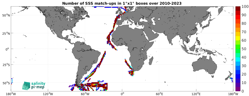
Figure 5: Number of SSS match-ups between TSG (Polarstern) SSS and the SMOS SSS L4 v1 - Daily (CMEMS-CNR) SSS product for the SMOS coastal zone (<800km) 60N-60S Pi-MEP region over 1^{\circ} \times 1^{\circ} boxes and for the full satellite product period.
