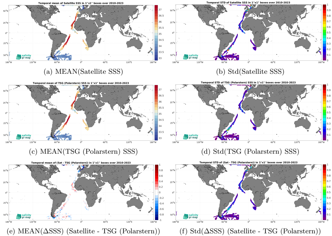
Figure 7: Temporal mean (left) and Std (right) of SSS from SMOS SSS L4 v1 - Daily (CMEMS-CNR) (top), TSG (Polarstern) (middle), and of \Delta SSS (Satellite - TSG (Polarstern)). Only match-up pairs are used to generate these maps.
