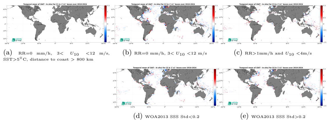
Figure 14: Temporal mean gridded over spatial boxes of size 1^\circ \times 1^\circ of \Delta\text{SSS} (SMOS SSS L4 v1 - Daily (CMEMS-CNR) - TSG (LEGOS-DM)) for 5 different subdatasets corresponding to:RR=0 mm/h, 3 < U_{10} < 12 m/s, SST >5^\circ\text{C} , distance to coast > 800 km (a), RR=0 mm/h, 3 < U_{10} < 12 m/s (b), RR >1 mm/h and U_{10} < 4 m/s (c), WOA2013 SSS Std <0.2 (d), WOA2013 SSS Std >0.2 (e).
