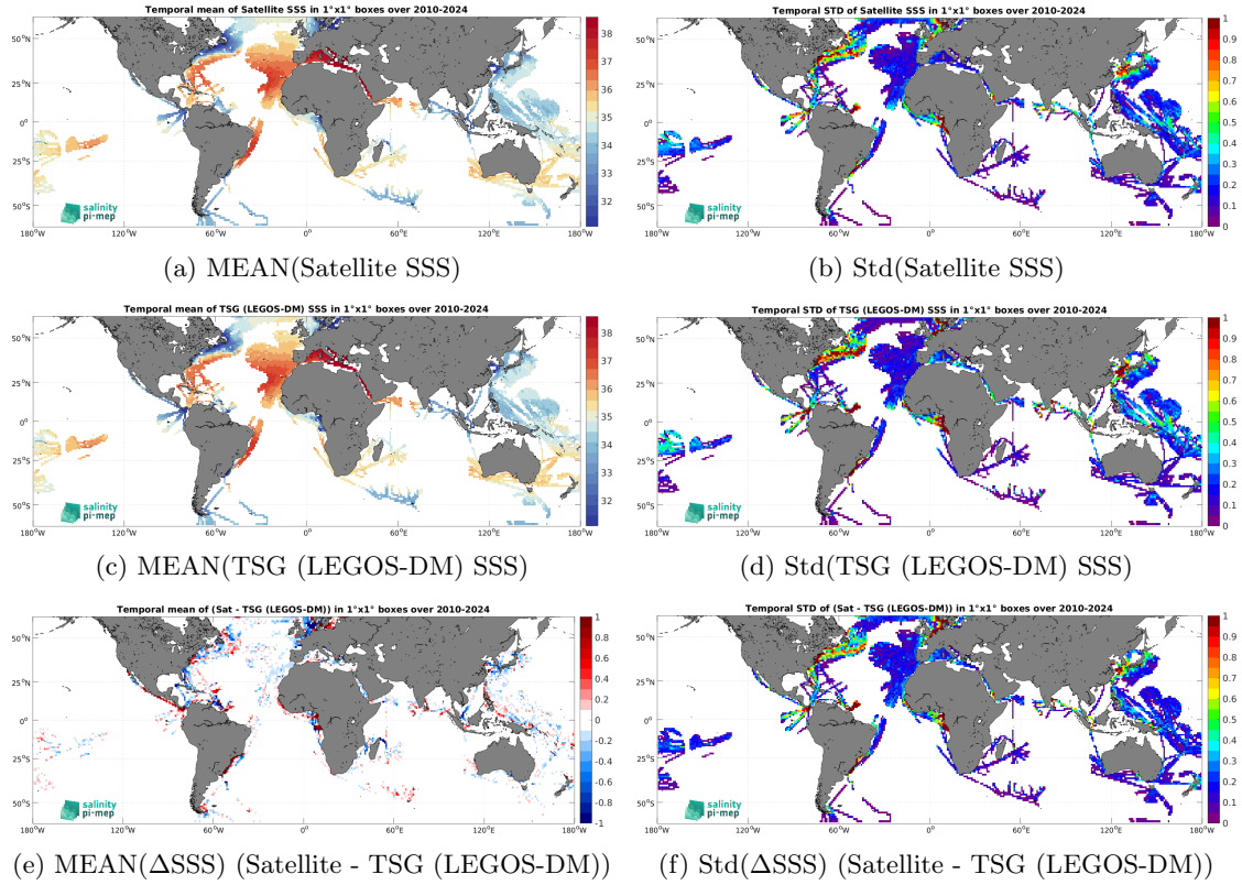
Figure 7: Temporal mean (left) and Std (right) of SSS from SMOS SSS L4 v1 - Daily (CMEMS-CNR) (top), TSG (LEGOS-DM) (middle), and of \Delta SSS (Satellite - TSG (LEGOS-DM)). Only match-up pairs are used to generate these maps.
