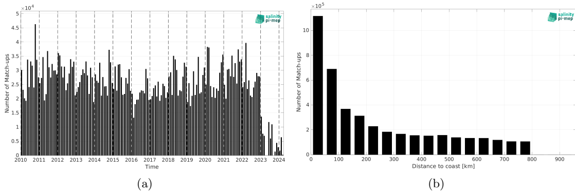
Figure 2: Number of match-ups between TSG (LEGOS-DM) and SMOS SSS L4 v1 - Daily (CMEMS-CNR) SSS as a function of time (a) and as function of the distance to coast (b) over the SMOS coastal zone (<800km) 60N-60S Pi-MEP region and for the full satellite product period.
