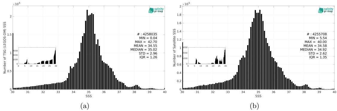
Figure 3: Histograms of SSS from TSG (LEGOS-DM) (a) and SMOS SSS L4 v1 - Daily (CMEMS-CNR) (b) considering all match-up pairs per bins of 0.1 over the SMOS coastal zone (<800km) 60N-60S Pi-MEP region and for the full satellite product period.
