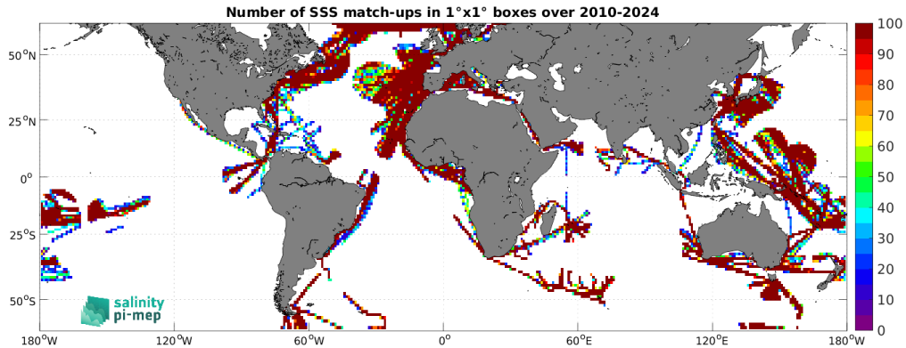
Figure 5: Number of SSS match-ups between TSG (LEGOS-DM) SSS and the SMOS SSS L4 v1 - Daily (CMEMS-CNR) SSS product for the SMOS coastal zone (<800km) 60N-60S Pi-MEP region over 1^\circ \times 1^\circ boxes and for the full satellite product period.
