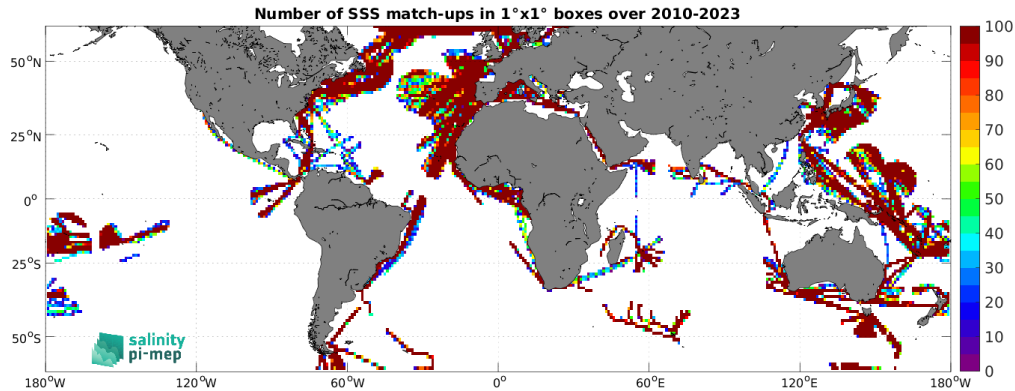
Figure 5: Number of SSS match-ups between TSG (LEGOS-DM) SSS and the SMOS SSS L4 v1 - Daily (CMEMS-CNR) SSS product for the SMOS coastal zone (<800km) 60N-60S Pi-MEP region over 1^{\circ} \times 1^{\circ} boxes and for the full satellite product period.
