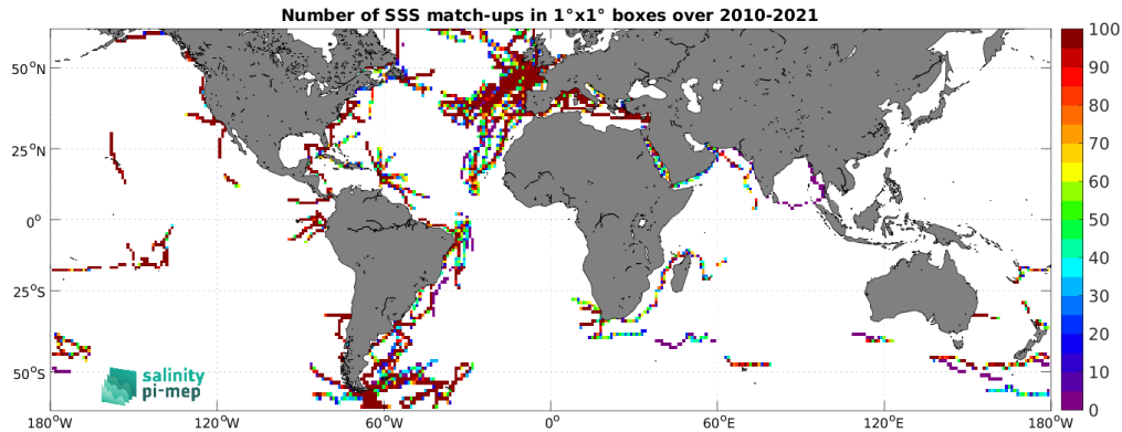
Figure 5: Number of SSS match-ups between TSG (GOSUD-Sailing-ship) SSS and the SMOS SSS L4 v1 - Daily (CMEMS-CNR) SSS product for the SMOS coastal zone (<800km) 60N-60S Pi-MEP region over 1^{\circ} \times 1^{\circ} boxes and for the full satellite product period.
