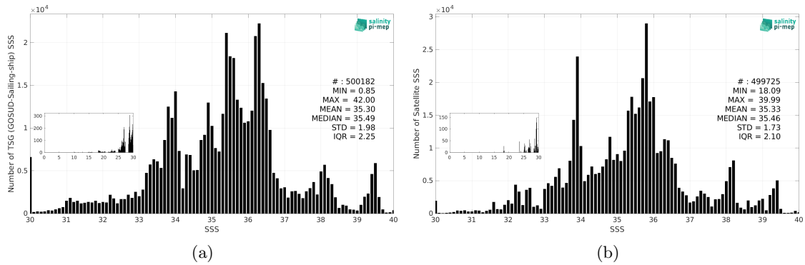
Figure 3: Histograms of SSS from TSG (GOSUD-Sailing-ship) (a) and SMOS SSS L4 v1 - Daily (CMEMS-CNR) (b) considering all match-up pairs per bins of 0.1 over the SMOS coastal zone (<800km) 60N-60S Pi-MEP region and for the full satellite product period.
