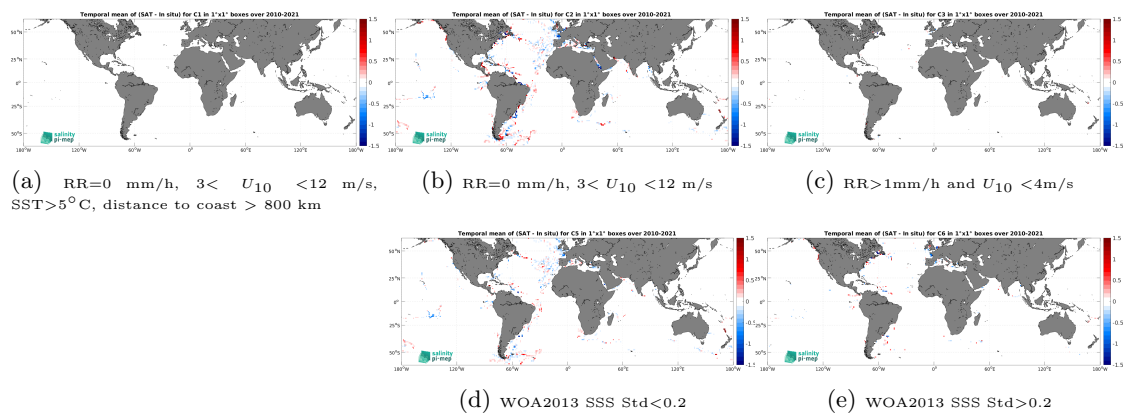
Figure 14: Temporal mean gridded over spatial boxes of size 1^\circ \times 1^\circ of \Delta SSS (SMOS SSS L4 v1 - Daily (CMEMS-CNR) - TSG (GOSUD-Sailing-ship)) for 5 different subdatasets corresponding to:RR=0 mm/h, 3 < U_{10} < 12 m/s, SST >5^\circ\text{C} , distance to coast > 800 km (a), RR=0 mm/h, 3 < U_{10} < 12 m/s (b), RR >1 mm/h and U_{10} < 4 m/s (c), WOA2013 SSS Std <0.2 (d), WOA2013 SSS Std >0.2 (e).
