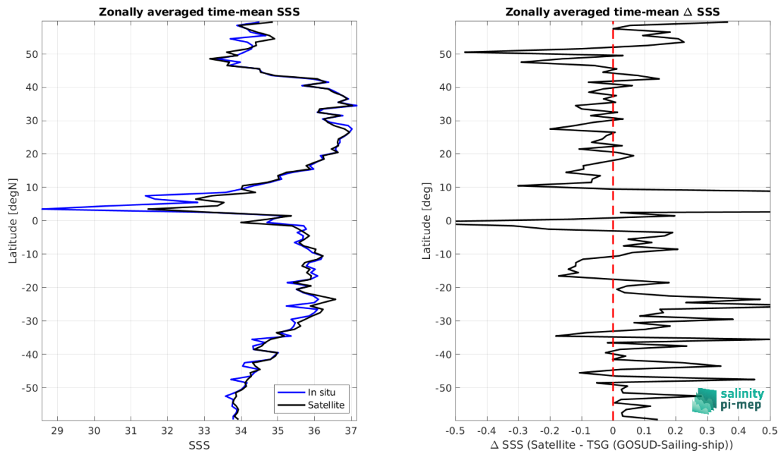
Figure 9: Left panel: Zonal mean SSS from SMOS SSS L4 v1 - Daily (CMEMS-CNR) satellite product (black) and from TSG (GOSUD-Sailing-ship) (blue). Right panel: Zonal mean of \Delta SSS (Satellite - TSG (GOSUD-Sailing-ship)) for all the collected Pi-MEP match-up pairs estimated over the full satellite product period.
