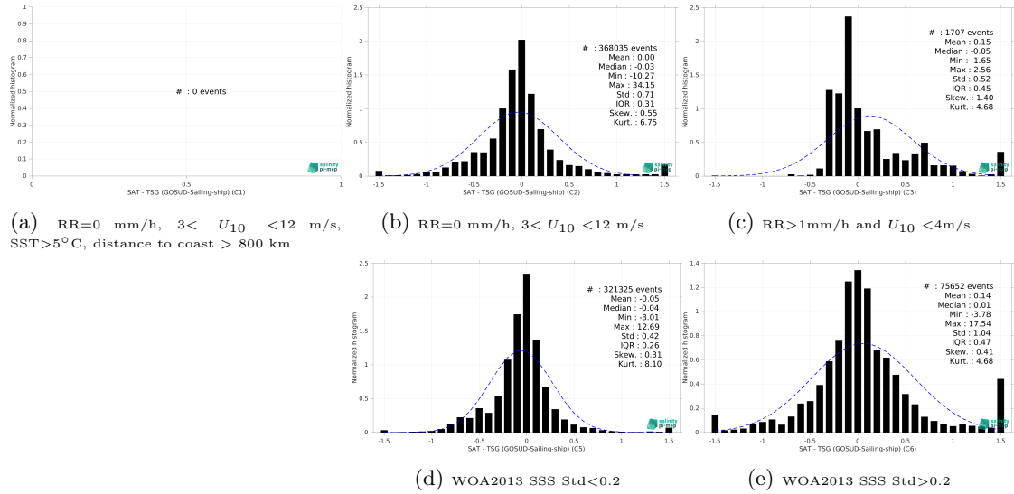
Figure 15: Normalized histogram of \Delta SSS (SMOS SSS L4 v1 - Daily (CMEMS-CNR) - TSG (GOSUD-Sailing-ship)) for 5 different subdatasets corresponding to: RR=0 mm/h, 3 < U_{10} < 12 m/s, SST>5°C, distance to coast > 800 km (a), RR=0 mm/h, 3 < U_{10} < 12 m/s (b), RR>1mm/h and U_{10} < 4 m/s (c), WOA2013 SSS Std<0.2 (d), WOA2013 SSS Std>0.2 (e).
