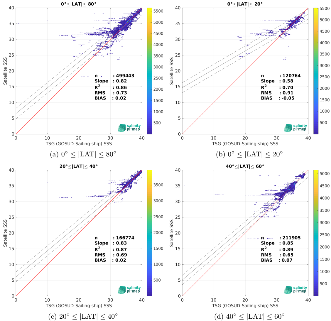
Figure 10: Contour maps of the concentration of SMOS SSS L4 v1 - Daily (CMEMS-CNR) SSS (y-axis) versus TSG (GOSUD-Sailing-ship) SSS (x-axis) at match-up pairs for different latitude bands. For each plot, the red line shows x=y . The black thin and dashed lines indicate a linear fit through the data cloud and the \pm 95\% confidence levels, respectively. The number match-up pairs n , the slope and R^2 coefficient of the linear fit, the root mean square (RMS) and the mean bias between satellite and in situ data are indicated for each latitude band in each plots.
