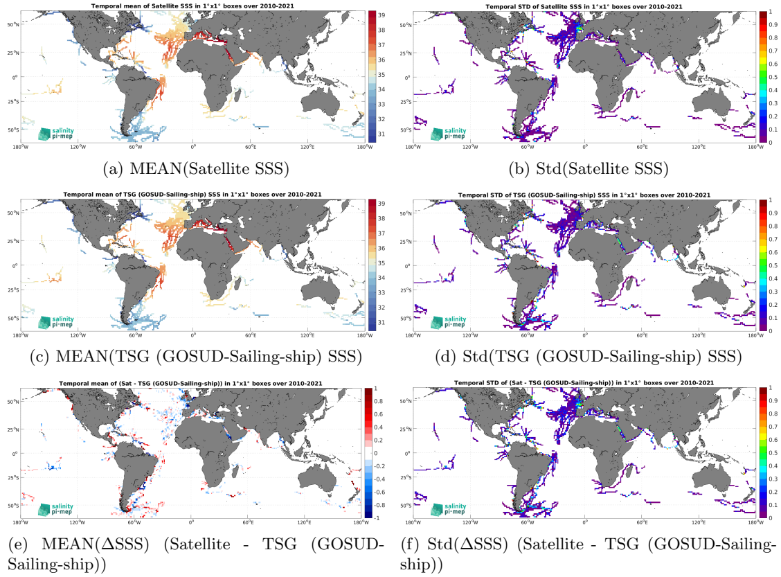
Figure 7: Temporal mean (left) and Std (right) of SSS from SMOS SSS L4 v1 - Daily (CMEMS-CNR) (top), TSG (GOSUD-Sailing-ship) (middle), and of \Delta SSS (Satellite - TSG (GOSUD-Sailing-ship)). Only match-up pairs are used to generate these maps.
