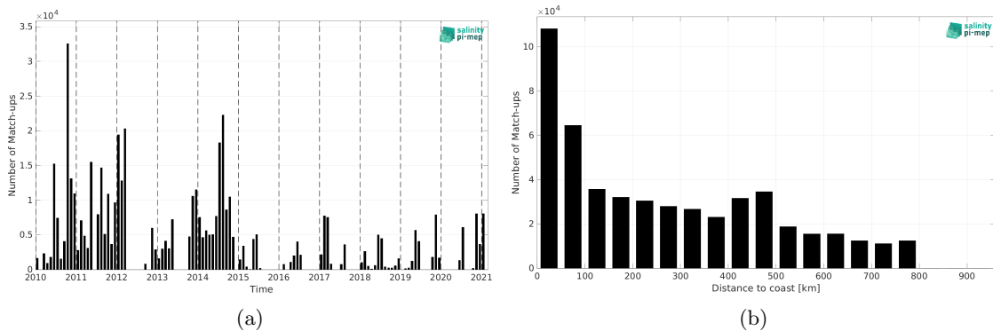
Figure 2: Number of match-ups between TSG (GOSUD-Sailing-ship) and SMOS SSS L4 v1 - Daily (CMEMS-CNR) SSS as a function of time (a) and as function of the distance to coast (b) over the SMOS coastal zone ( < 800\text{km} ) 60\text{N}-60\text{S} Pi-MEP region and for the full satellite product period.
