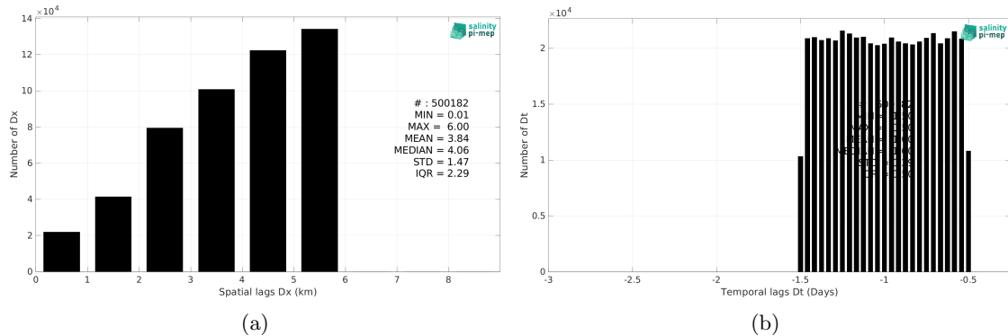
Figure 6: Histograms of the spatial (a) and temporal (b) lags between the location/time of the TSG (GOSUD-Sailing-ship) measurement and the date of the corresponding SMOS SSS L4 v1 - Daily (CMEMS-CNR) SSS pixel.
