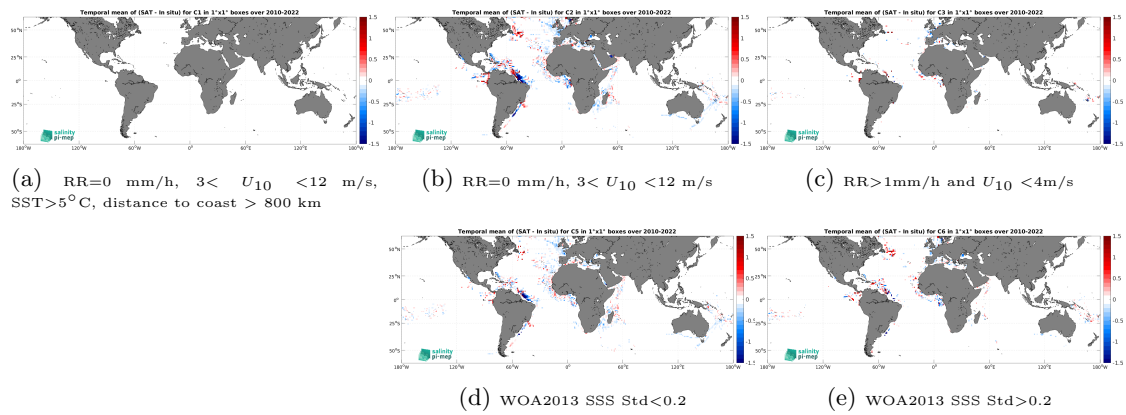
Figure 14: Temporal mean gridded over spatial boxes of size 1^\circ \times 1^\circ of \Delta\text{SSS} (SMOS SSS L4 v1 - Daily (CMEMS-CNR) - TSG (GOSUD-Research-vessel)) for 5 different subdatasets corresponding to: RR=0 mm/h, 3 < U_{10} < 12 m/s, SST > 5°C, distance to coast > 800 km (a), RR=0 mm/h, 3 < U_{10} < 12 m/s (b), RR > 1mm/h and U_{10} < 4 m/s (c), WOA2013 SSS Std < 0.2 (d), WOA2013 SSS Std > 0.2 (e).
