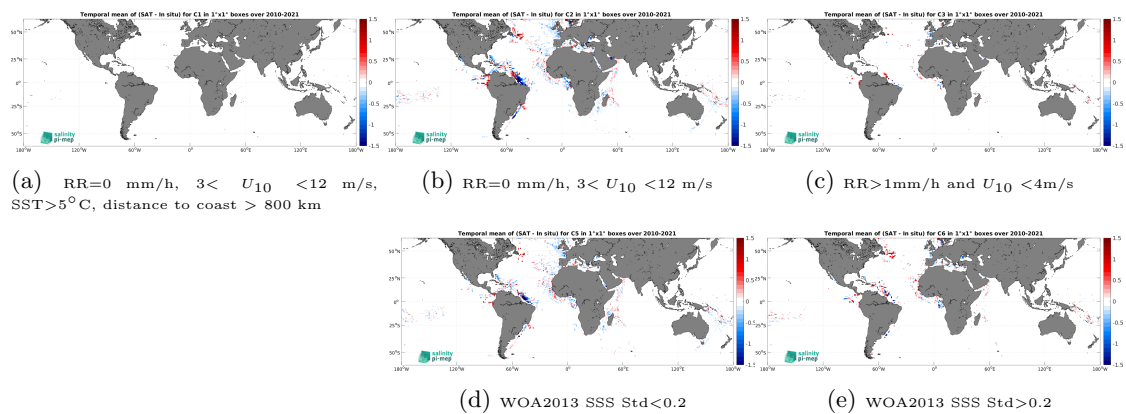
Figure 14: Temporal mean gridded over spatial boxes of size 1^\circ \times 1^\circ of \Delta SSS (SMOS SSS L4 v1 - Daily (CMEMS-CNR) - TSG (GOSUD-Research-vessel)) for 5 different subdatasets corresponding to:RR=0 mm/h, 3 < U_{10} < 12 m/s, SST >5^\circ\text{C} , distance to coast > 800 km (a), RR=0 mm/h, 3 < U_{10} < 12 m/s (b), RR >1 mm/h and U_{10} < 4 m/s (c), WOA2013 SSS Std <0.2 (d), WOA2013 SSS Std >0.2 (e).
