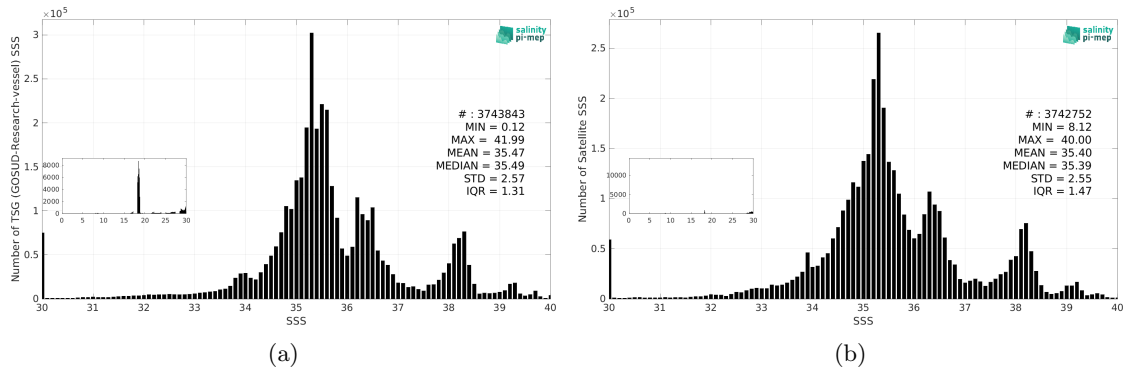
Figure 3: Histograms of SSS from TSG (GOSUD-Research-vessel) (a) and SMOS SSS L4 v1 - Daily (CMEMS-CNR) (b) considering all match-up pairs per bins of 0.1 over the SMOS coastal zone (<800km) 60N-60S Pi-MEP region and for the full satellite product period.
