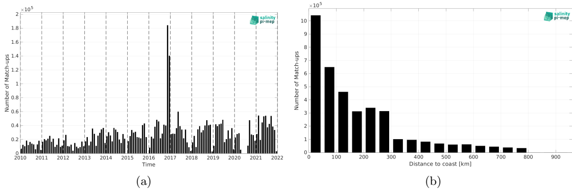
Figure 2: Number of match-ups between TSG (GOSUD-Research-vessel) and SMOS SSS L4 v1 - Daily (CMEMS-CNR) SSS as a function of time (a) and as function of the distance to coast (b) over the SMOS coastal zone (<800km) 60N-60S Pi-MEP region and for the full satellite product period.
