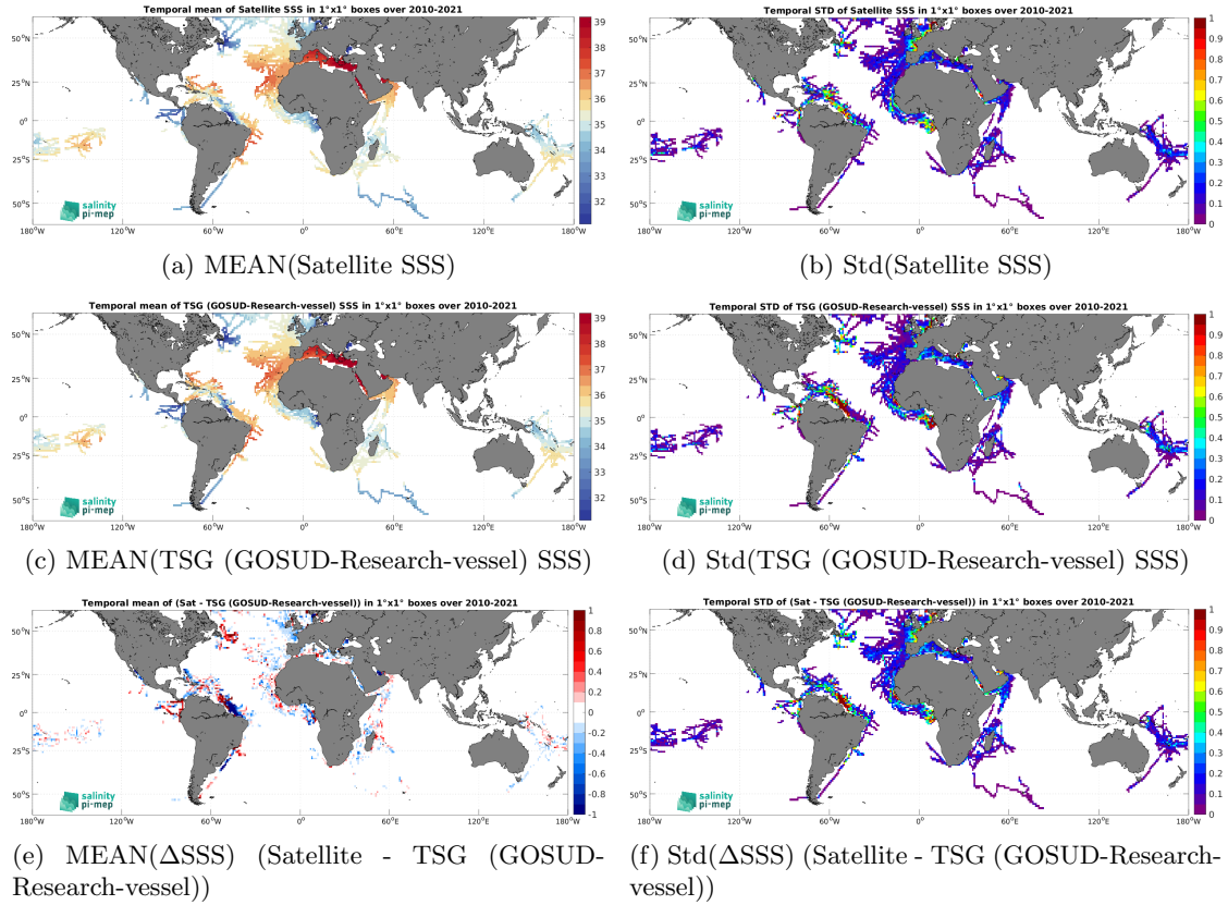
Figure 7: Temporal mean (left) and Std (right) of SSS from SMOS SSS L4 v1 - Daily (CMEMS-CNR) (top), TSG (GOSUD-Research-vessel) (middle), and of \Delta SSS (Satellite - TSG (GOSUD-Research-vessel)). Only match-up pairs are used to generate these maps.
