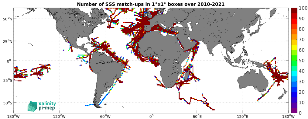
Figure 5: Number of SSS match-ups between TSG (GOSUD-Research-vessel) SSS and the SMOS SSS L4 v1 - Daily (CMEMS-CNR) SSS product for the SMOS coastal zone (<800km) 60N-60S Pi-MEP region over 1^{\circ} \times 1^{\circ} boxes and for the full satellite product period.
