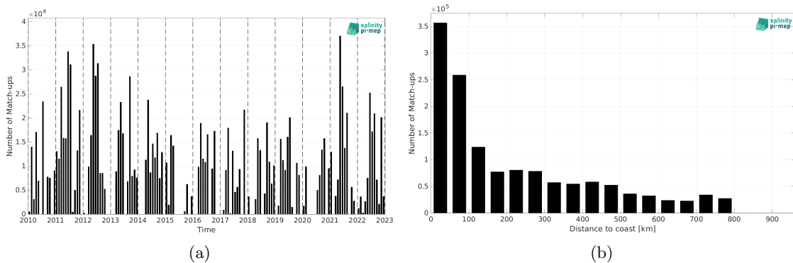
Figure 2: Number of match-ups between TSG (CSIC-UTM) and SMOS SSS L4 v1 - Daily (CMEMS-CNR) SSS as a function of time (a) and as function of the distance to coast (b) over the SMOS coastal zone (<800km) 60N-60S Pi-MEP region and for the full satellite product period.
