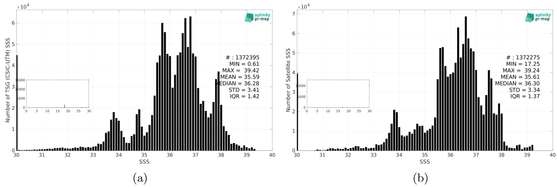
Figure 3: Histograms of SSS from TSG (CSIC-UTM) (a) and SMOS SSS L4 v1 - Daily (CMEMS-CNR) (b) considering all match-up pairs per bins of 0.1 over the SMOS coastal zone (<800km) 60N-60S Pi-MEP region and for the full satellite product period.
