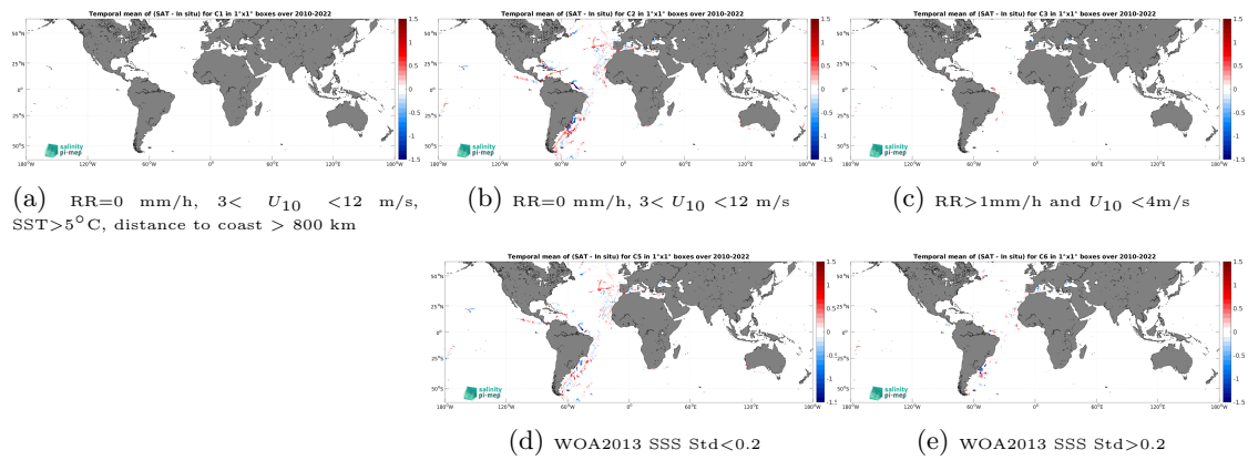
Figure 14: Temporal mean gridded over spatial boxes of size 1^\circ \times 1^\circ of \Delta SSS (SMOS SSS L4 v1 - Daily (CMEMS-CNR) - TSG (CSIC-UTM)) for 5 different subdatasets corresponding to:RR=0 mm/h, 3 < U_{10} < 12 m/s, SST >5^\circ\text{C} , distance to coast > 800 km (a), RR=0 mm/h, 3 < U_{10} < 12 m/s (b), RR >1 mm/h and U_{10} < 4 m/s (c), WOA2013 SSS Std <0.2 (d), WOA2013 SSS Std >0.2 (e).
