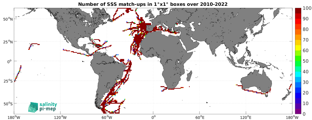
Figure 5: Number of SSS match-ups between TSG (CSIC-UTM) SSS and the SMOS SSS L4 v1 - Daily (CMEMS-CNR) SSS product for the SMOS coastal zone (<800km) 60N-60S Pi-MEP region over 1^{\circ} \times 1^{\circ} boxes and for the full satellite product period.
