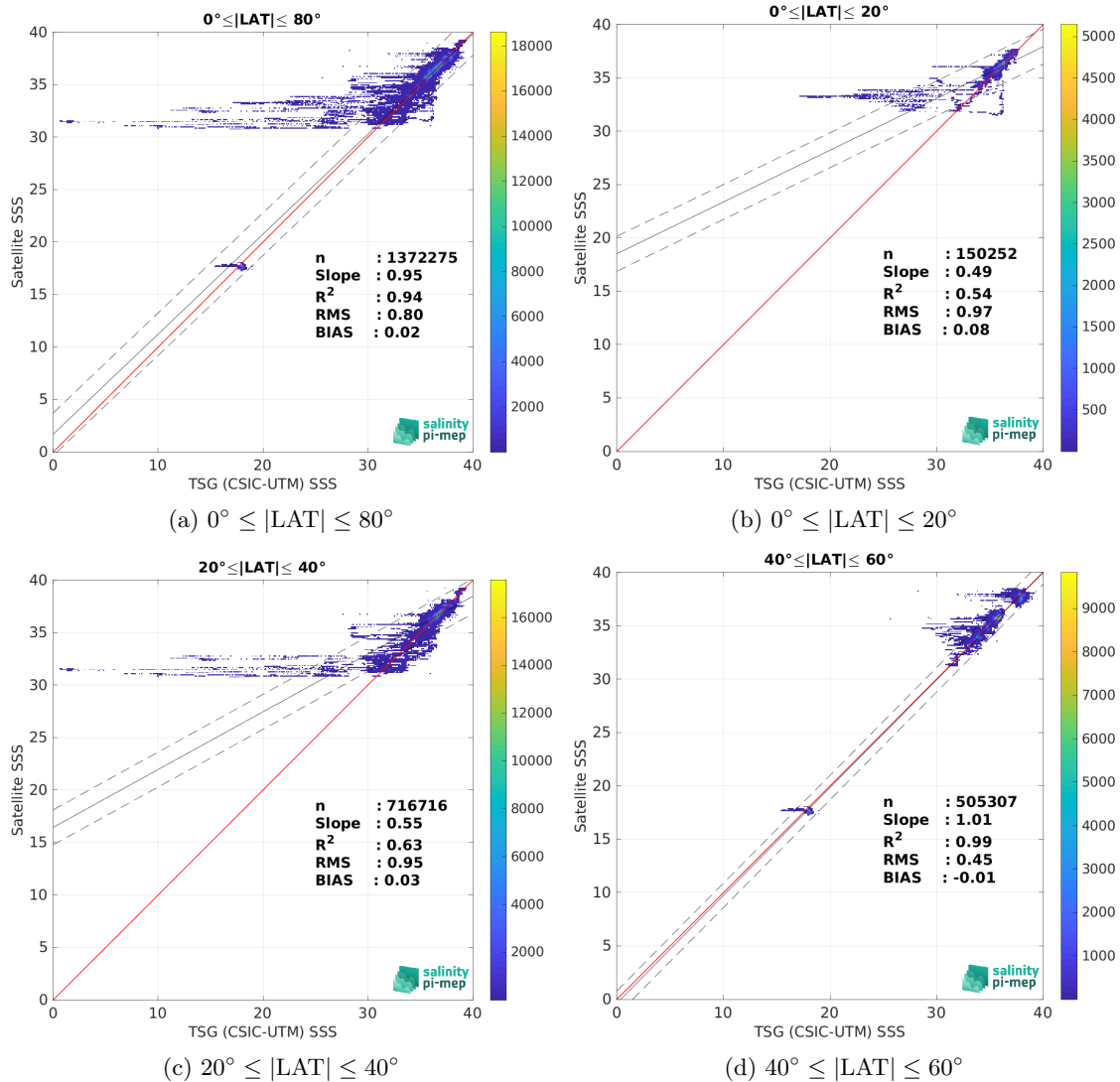
Figure 10: Contour maps of the concentration of SMOS SSS L4 v1 - Daily (CMEMS-CNR) SSS (y-axis) versus TSG (CSIC-UTM) SSS (x-axis) at match-up pairs for different latitude bands. For each plot, the red line shows x=y . The black thin and dashed lines indicate a linear fit through the data cloud and the \pm 95\% confidence levels, respectively. The number match-up pairs n , the slope and R^2 coefficient of the linear fit, the root mean square (RMS) and the mean bias between satellite and in situ data are indicated for each latitude band in each plots.
