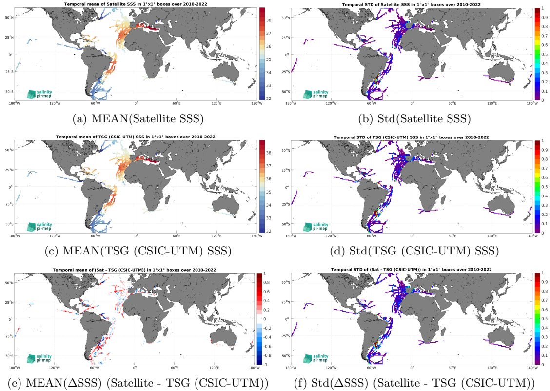
Figure 7: Temporal mean (left) and Std (right) of SSS from SMOS SSS L4 v1 - Daily (CMEMS-CNR) (top), TSG (CSIC-UTM) (middle), and of \Delta SSS (Satellite - TSG (CSIC-UTM)). Only match-up pairs are used to generate these maps.
