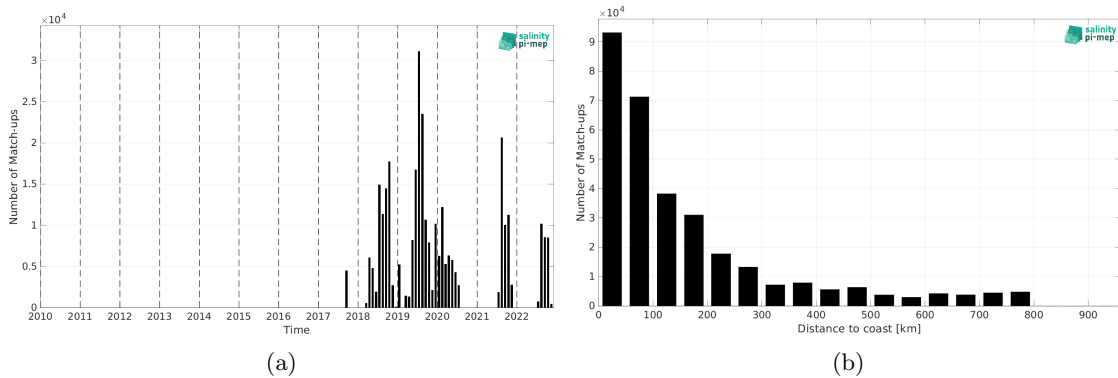
Figure 2: Number of match-ups between Saildrone and SMOS SSS L4 v1 - Daily (CMEMS-CNR) SSS as a function of time (a) and as function of the distance to coast (b) over the SMOS coastal zone (<800km) 60N-60S Pi-MEP region and for the full satellite product period.
