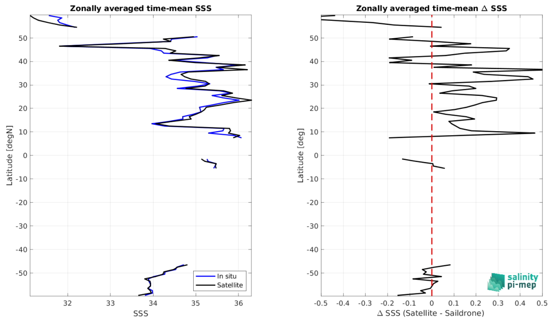
Figure 9: Left panel: Zonal mean SSS from SMOS SSS L4 v1 - Daily (CMEMS-CNR) satellite product (black) and from Sailldrone (blue). Right panel: Zonal mean of \Delta SSS (Satellite - Sailldrone) for all the collected Pi-MEP match-up pairs estimated over the full satellite product period.
