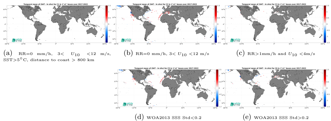
Figure 14: Temporal mean gridded over spatial boxes of size 1^\circ \times 1^\circ of \Delta SSS (SMOS SSS L4 v1 - Daily (CMEMS-CNR) - Sailydrone) for 5 different subdatasets corresponding to:RR=0 mm/h, 3 < U_{10} < 12 m/s, SST >5^\circ\text{C} , distance to coast > 800 km (a), RR=0 mm/h, 3 < U_{10} < 12 m/s (b), RR >1 mm/h and U_{10} < 4 m/s (c), WOA2013 SSS Std <0.2 (d), WOA2013 SSS Std >0.2 (e).
