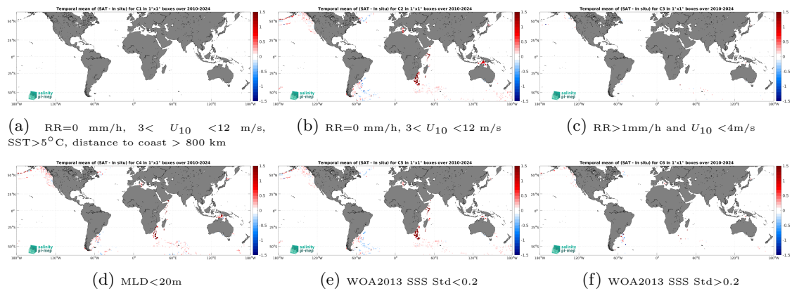
Figure 14: Temporal mean gridded over spatial boxes of size 1^\circ \times 1^\circ of \Delta SSS (SMOS SSS L4 v1 - Daily (CMEMS-CNR) - Marine mammals) for 6 different subdatasets corresponding to:RR=0 mm/h, 3 < U_{10} < 12 m/s, SST >5^\circ C, distance to coast > 800 km (a), RR=0 mm/h, 3 < U_{10} < 12 m/s (b), RR >1 mm/h and U_{10} < 4 m/s (c),MLD <20 m (d),WOA2013 SSS Std <0.2 (e),WOA2013 SSS Std >0.2 (f).
