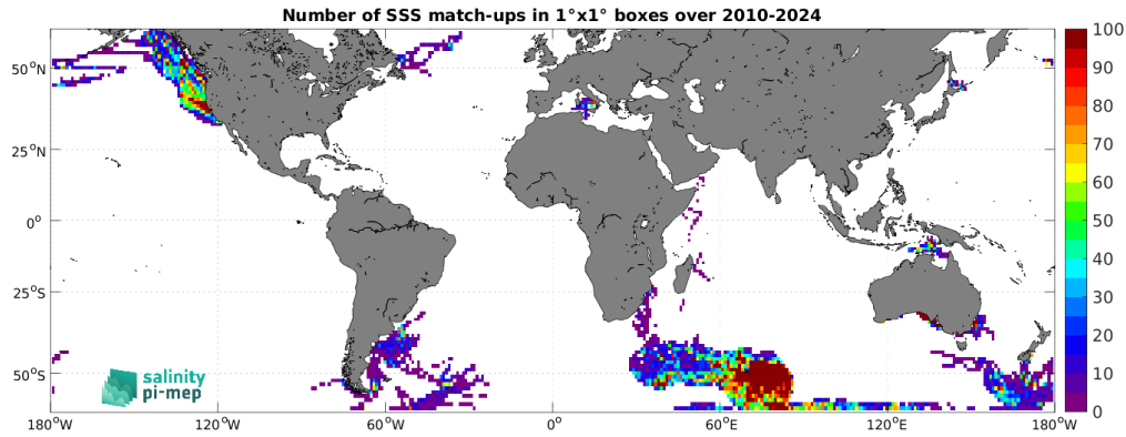
Figure 5: Number of SSS match-ups between Marine mammals SSS and the SMOS SSS L4 v1 - Daily (CMEMS-CNR) SSS product for the SMOS coastal zone (<800km) 60N-60S Pi-MEP region over 1^{\circ} \times 1^{\circ} boxes and for the full satellite product period.
