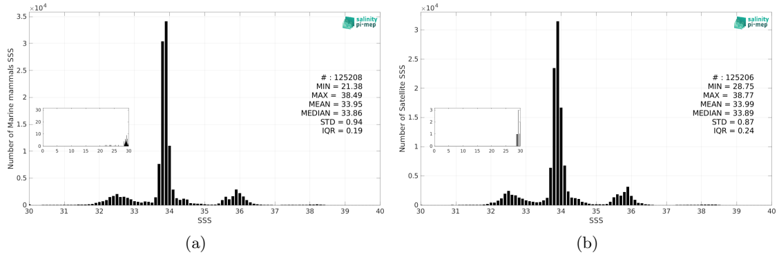
Figure 3: Histograms of SSS from Marine mammals (a) and SMOS SSS L4 v1 - Daily (CMEMS-CNR) (b) considering all match-up pairs per bins of 0.1 over the SMOS coastal zone (<800km) 60N-60S Pi-MEP region and for the full satellite product period.
