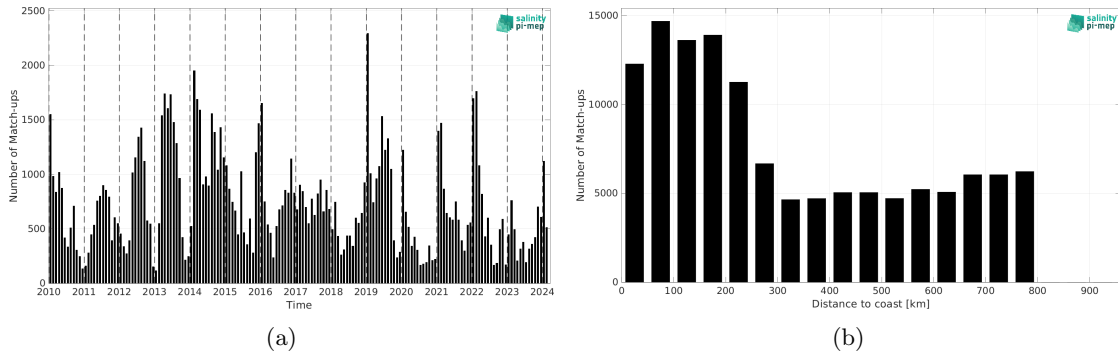
Figure 2: Number of match-ups between Marine mammals and SMOS SSS L4 v1 - Daily (CMEMS-CNR) SSS as a function of time (a) and as function of the distance to coast (b) over the SMOS coastal zone (<800km) 60N-60S Pi-MEP region and for the full satellite product period.
