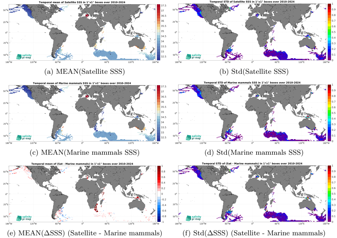
Figure 7: Temporal mean (left) and Std (right) of SSS from SMOS SSS L4 v1 - Daily (CMEMS-CNR) (top), Marine mammals (middle), and of \Delta SSS (Satellite - Marine mammals). Only match-up pairs are used to generate these maps.
