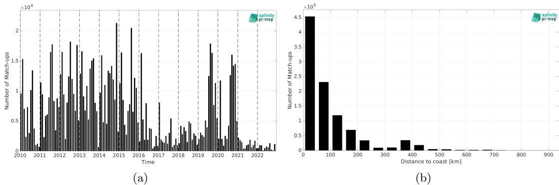
Figure 2: Number of match-ups between ICES and SMOS SSS L4 v1 - Daily (CMEMS-CNR) SSS as a function of time (a) and as function of the distance to coast (b) over the SMOS coastal zone (<800km) 60N-60S Pi-MEP region and for the full satellite product period.
