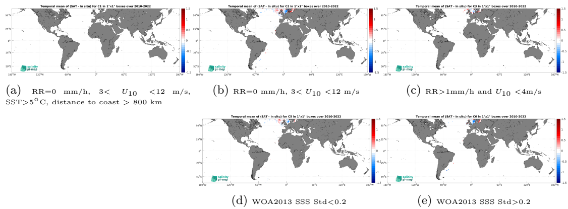
Figure 14: Temporal mean gridded over spatial boxes of size 1^\circ \times 1^\circ of \Delta SSS (SMOS SSS L4 v1 - Daily (CMEMS-CNR) - ICES) for 5 different subdatasets corresponding to:RR=0 mm/h, 3 < U_{10} < 12 m/s, SST >5^\circ\text{C} , distance to coast > 800 km (a), RR=0 mm/h, 3 < U_{10} < 12 m/s (b), RR >1 mm/h and U_{10} < 4 m/s (c), WOA2013 SSS Std <0.2 (d), WOA2013 SSS Std >0.2 (e).
