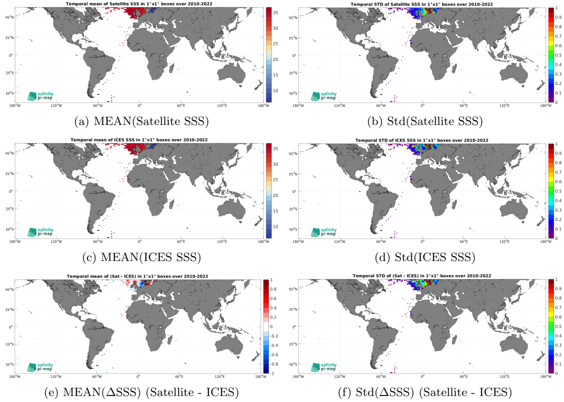
Figure 7: Temporal mean (left) and Std (right) of SSS from SMOS SSS L4 v1 - Daily (CMEMS-CNR) (top), ICES (middle), and of \Delta SSS (Satellite - ICES). Only match-up pairs are used to generate these maps.
