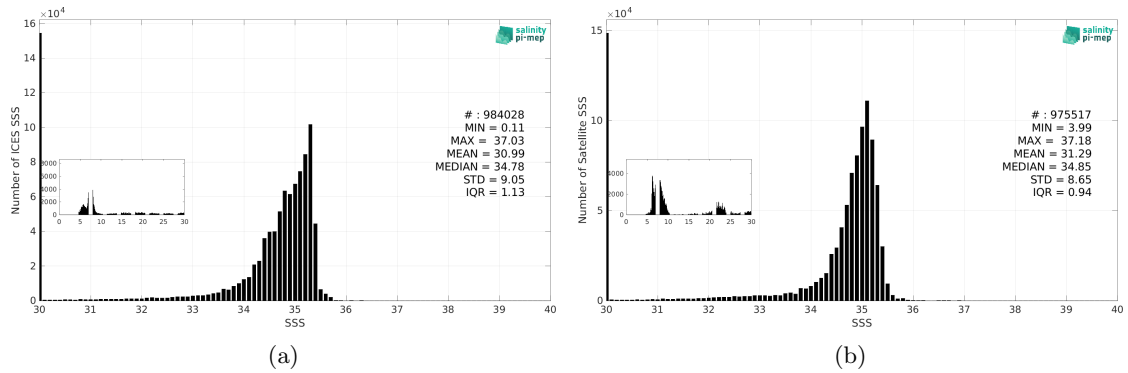
Figure 3: Histograms of SSS from ICES (a) and SMOS SSS L4 v1 - Daily (CMEMS-CNR) (b) considering all match-up pairs per bins of 0.1 over the SMOS coastal zone (<800km) 60N-60S Pi-MEP region and for the full satellite product period.
