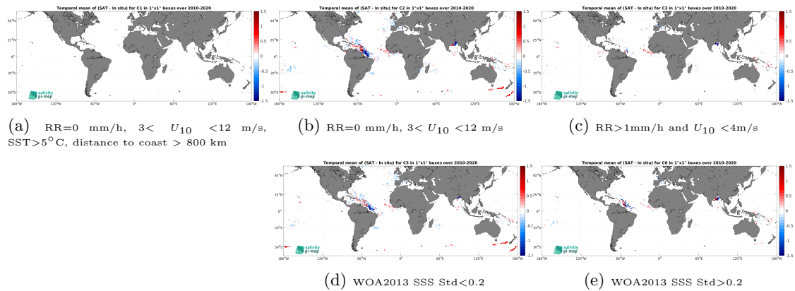
Figure 13: Temporal mean gridded over spatial boxes of size 1^\circ \times 1^\circ of \Delta\text{SSS} (SMOS SSS L4 v1 - Daily (CMEMS-CNR) - Surface drifters) for 5 different subdatasets corresponding to:RR=0 mm/h, 3 < U_{10} < 12 m/s, SST >5^\circ\text{C} , distance to coast > 800 km (a), RR=0 mm/h, 3 < U_{10} < 12 m/s (b), RR >1 mm/h and U_{10} < 4 m/s (c), WOA2013 SSS Std <0.2 (d), WOA2013 SSS Std >0.2 (e).
