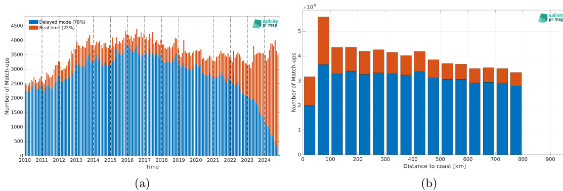
Figure 2: Number of match-ups between Argo and SMOS SSS L4 v1 - Daily (CMEMS-CNR) SSS as a function of time (a) and as function of the distance to coast (b) over the SMOS coastal zone (<800km) 60N-60S Pi-MEP region and for the full satellite product period.
