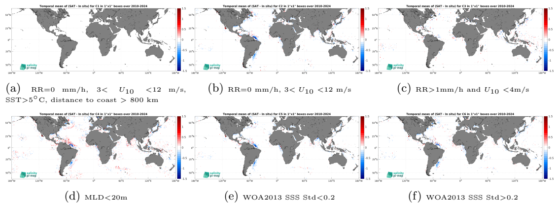
Figure 14: Temporal mean gridded over spatial boxes of size 1^\circ \times 1^\circ of \Delta SSS (SMOS SSS L4 v1 - Daily (CMEMS-CNR) - Argo) for 6 different subdatasets corresponding to:RR=0 mm/h, 3 < U_{10} < 12 m/s, SST > 5^\circ\text{C} , distance to coast > 800 km (a), RR=0 mm/h, 3 < U_{10} < 12 m/s (b), RR > 1 mm/h and U_{10} < 4 m/s (c),MLD < 20 m (d),WOA2013 SSS Std < 0.2 (e),WOA2013 SSS Std > 0.2 (f).
