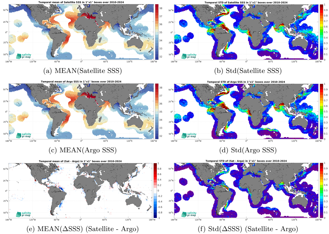
Figure 7: Temporal mean (left) and Std (right) of SSS from SMOS SSS L4 v1 - Daily (CMEMS-CNR) (top), Argo (middle), and of \Delta SSS (Satellite - Argo). Only match-up pairs are used to generate these maps.
