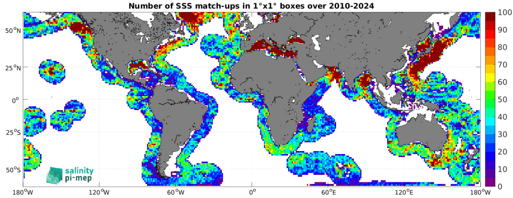
Figure 5: Number of SSS match-ups between Argo SSS and the SMOS SSS L4 v1 - Daily (CMEMS-CNR) SSS product for the SMOS coastal zone (<800km) 60N-60S Pi-MEP region over 1^\circ \times 1^\circ boxes and for the full satellite product period.
