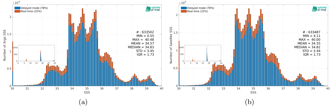
Figure 3: Histograms of SSS from Argo (a) and SMOS SSS L4 v1 - Daily (CMEMS-CNR) (b) considering all match-up pairs per bins of 0.1 over the SMOS coastal zone (<800km) 60N-60S Pi-MEP region and for the full satellite product period.
