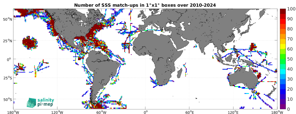
Figure 5: Number of SSS match-ups between TSG (SAMOS) SSS and the SMOS SSS L4 OI v346 - Weekly (CMEMS-CATDS-LOPS) SSS product for the SMOS coastal zone (<800km) 60N-60S Pi-MEP region over 1^\circ \times 1^\circ boxes and for the full satellite product period.
