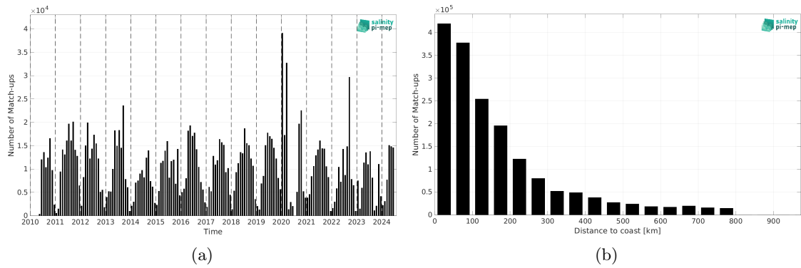
Figure 2: Number of match-ups between TSG (SAMOS) and SMOS SSS L4 OI v346 - Weekly (CMEMS-CATDS-LOPS) SSS as a function of time (a) and as function of the distance to coast (b) over the SMOS coastal zone (<800km) 60N-60S Pi-MEP region and for the full satellite product period.
