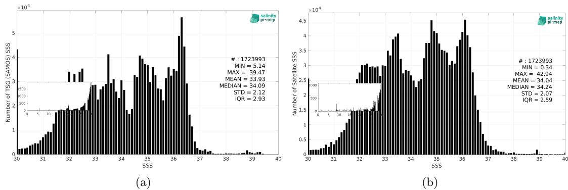
Figure 3: Histograms of SSS from TSG (SAMOS) (a) and SMOS SSS L4 OI v346 - Weekly (CMEMS-CATDS-LOPS) (b) considering all match-up pairs per bins of 0.1 over the SMOS coastal zone (<800km) 60N-60S Pi-MEP region and for the full satellite product period.
