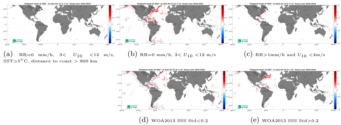
Figure 14: Temporal mean gridded over spatial boxes of size 1^\circ \times 1^\circ of \Delta\text{SSS} (SMOS SSS L4 OI v346 - Weekly (CMEMS-CATDS-LOPS) - TSG (SAMOS)) for 5 different subdatasets corresponding to:RR=0 mm/h, 3 < U_{10} < 12 m/s, SST > 5^\circ\text{C} , distance to coast > 800 km (a), RR=0 mm/h, 3 < U_{10} < 12 m/s (b), RR > 1 mm/h and U_{10} < 4 m/s (c), WOA2013 SSS Std < 0.2 (d), WOA2013 SSS Std > 0.2 (e).
