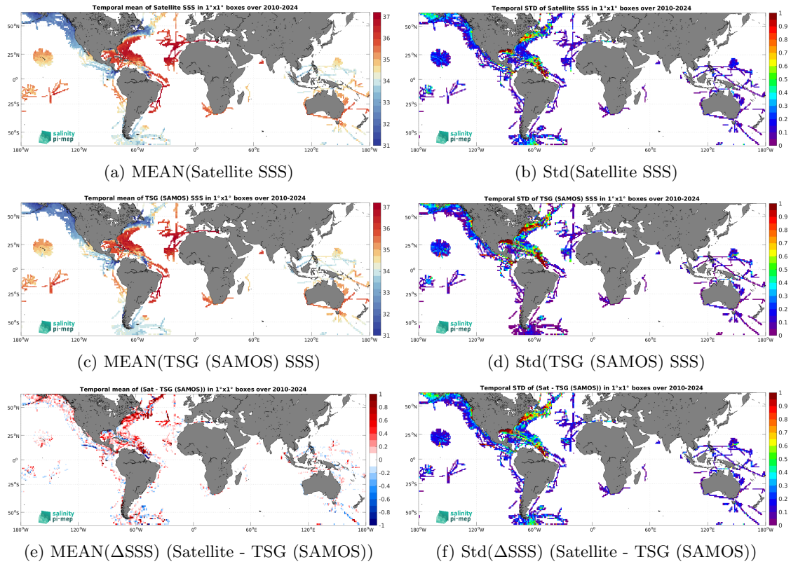
Figure 7: Temporal mean (left) and Std (right) of SSS from SMOS SSS L4 OI v346 - Weekly (CMEMS-CATDS-LOPS) (top), TSG (SAMOS) (middle), and of \Delta SSS (Satellite - TSG (SAMOS)). Only match-up pairs are used to generate these maps.
