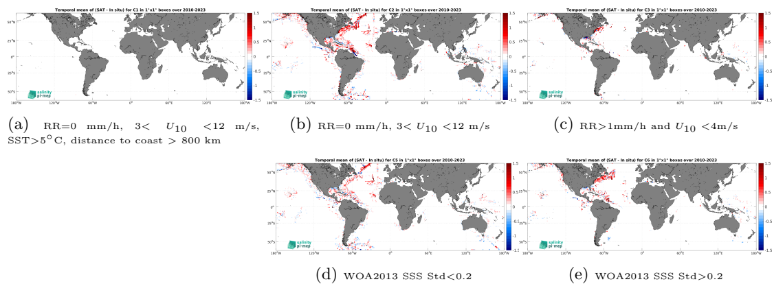
Figure 14: Temporal mean gridded over spatial boxes of size 1^\circ \times 1^\circ of \Delta SSS (SMOS SSS L4 OI v346 - Weekly (CMEMS-CATDS-LOPS) - TSG (SAMOS)) for 5 different subdatasets corresponding to:RR=0 mm/h, 3 < U_{10} < 12 m/s, SST >5^\circ C, distance to coast > 800 km (a), RR=0 mm/h, 3 < U_{10} < 12 m/s (b), RR >1 mm/h and U_{10} < 4 m/s (c), WOA2013 SSS Std <0.2 (d), WOA2013 SSS Std >0.2 (e).
