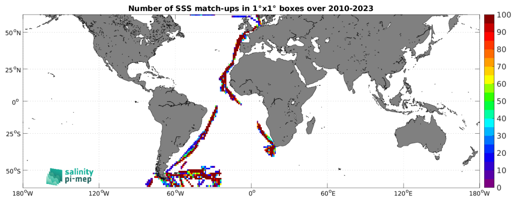
Figure 5: Number of SSS match-ups between TSG (Polarstern) SSS and the SMOS SSS L4 OI v346 - Weekly (CMEMS-CATDS-LOPS) SSS product for the SMOS coastal zone ( <800\text{km} ) 60N-60S Pi-MEP region over 1^\circ \times 1^\circ boxes and for the full satellite product period.
