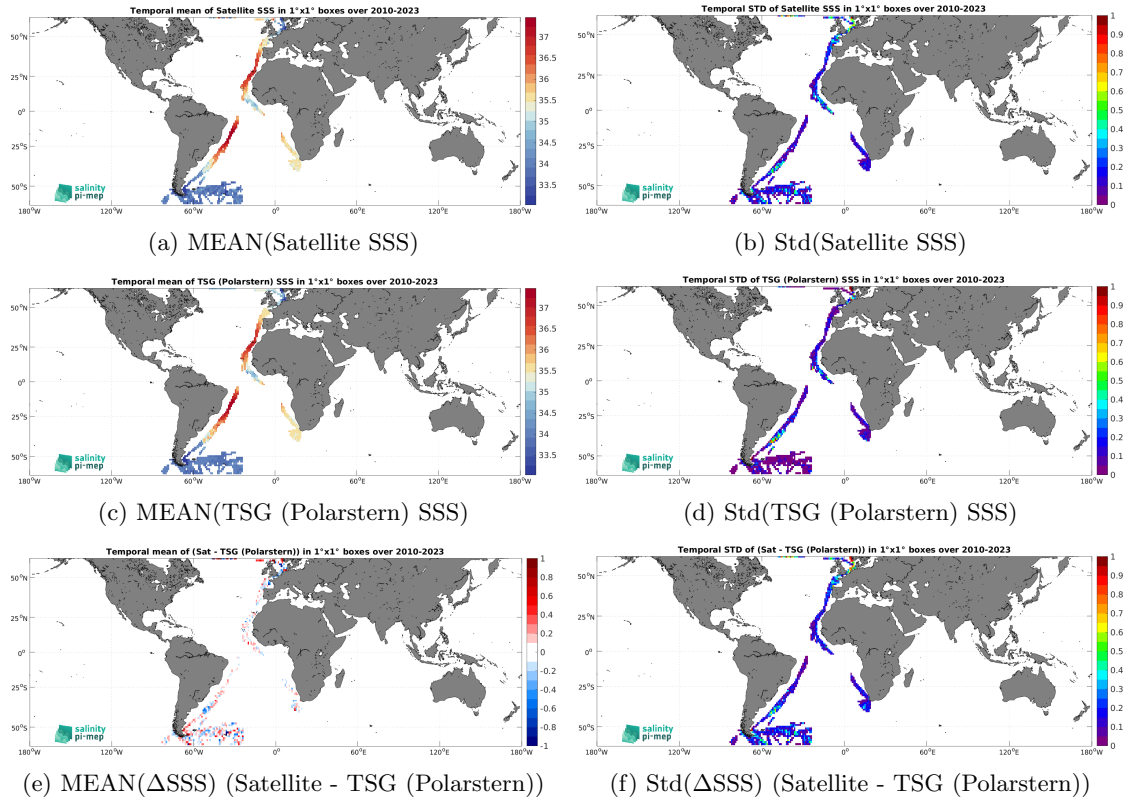
Figure 7: Temporal mean (left) and Std (right) of SSS from SMOS SSS L4 OI v346 - Weekly (CMEMS-CATDS-LOPS) (top), TSG (Polarstern) (middle), and of \Delta SSS (Satellite - TSG (Polarstern)). Only match-up pairs are used to generate these maps.
