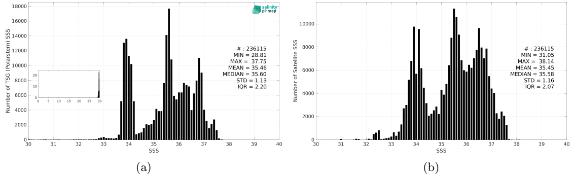
Figure 3: Histograms of SSS from TSG (Polarstern) (a) and SMOS SSS L4 OI v346 - Weekly (CMEMS-CATDS-LOPS) (b) considering all match-up pairs per bins of 0.1 over the SMOS coastal zone (<800km) 60N-60S Pi-MEP region and for the full satellite product period.
