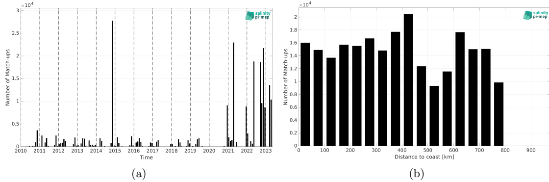
Figure 2: Number of match-ups between TSG (Polarstern) and SMOS SSS L4 OI v346 - Weekly (CMEMS-CATDS-LOPS) SSS as a function of time (a) and as function of the distance to coast (b) over the SMOS coastal zone (<800km) 60N-60S Pi-MEP region and for the full satellite product period.
