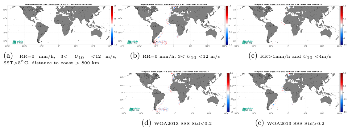
Figure 14: Temporal mean gridded over spatial boxes of size 1^\circ \times 1^\circ of \Delta SSS (SMOS SSS L4 OI v346 - Weekly (CMEMS-CATDS-LOPS) - TSG (Polarstern)) for 5 different subdatasets corresponding to:RR=0 mm/h, 3 < U_{10} < 12 m/s, SST >5^\circ\text{C} , distance to coast > 800 km (a), RR=0 mm/h, 3 < U_{10} < 12 m/s (b), RR >1 mm/h and U_{10} < 4 m/s (c), WOA2013 SSS Std <0.2 (d), WOA2013 SSS Std >0.2 (e).
