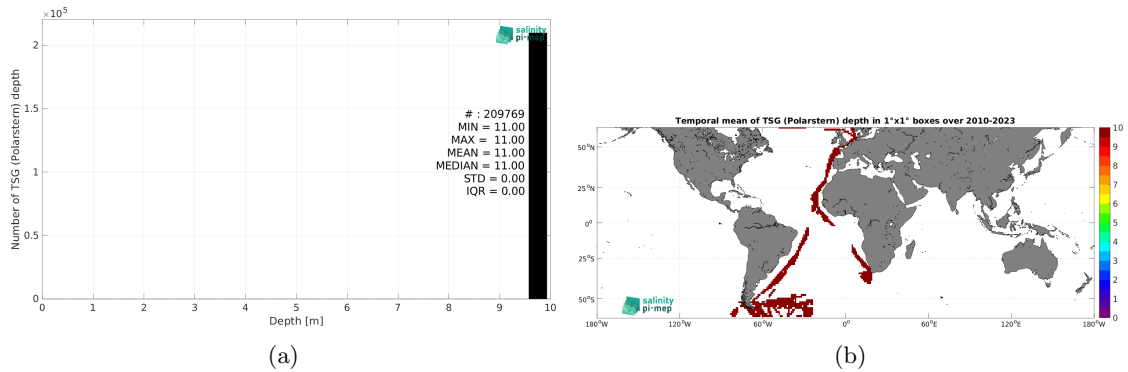
Figure 4: Histograms of the depth of the upper level SSS measurements from TSG (Polarstern) in the Match-up DataBase for the SMOS coastal zone ( <800\text{km} ) 60\text{N} - 60\text{S} Pi-MEP region (a) and temporal mean spatial distribution of pressure of the in situ SSS data over 1^\circ \times 1^\circ boxes and for the full satellite product period (b).
