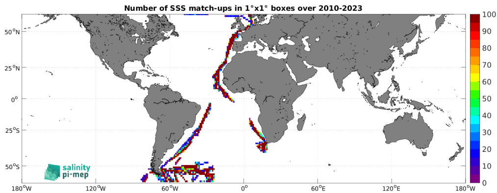
Figure 5: Number of SSS match-ups between TSG (Polarstern) SSS and the SMOS SSS L4 OI v346 - Weekly (CMEMS-CATDS-LOPS) SSS product for the SMOS coastal zone ( <800\text{km} ) 60\text{N} - 60\text{S} Pi-MEP region over 1^\circ \times 1^\circ boxes and for the full satellite product period.
