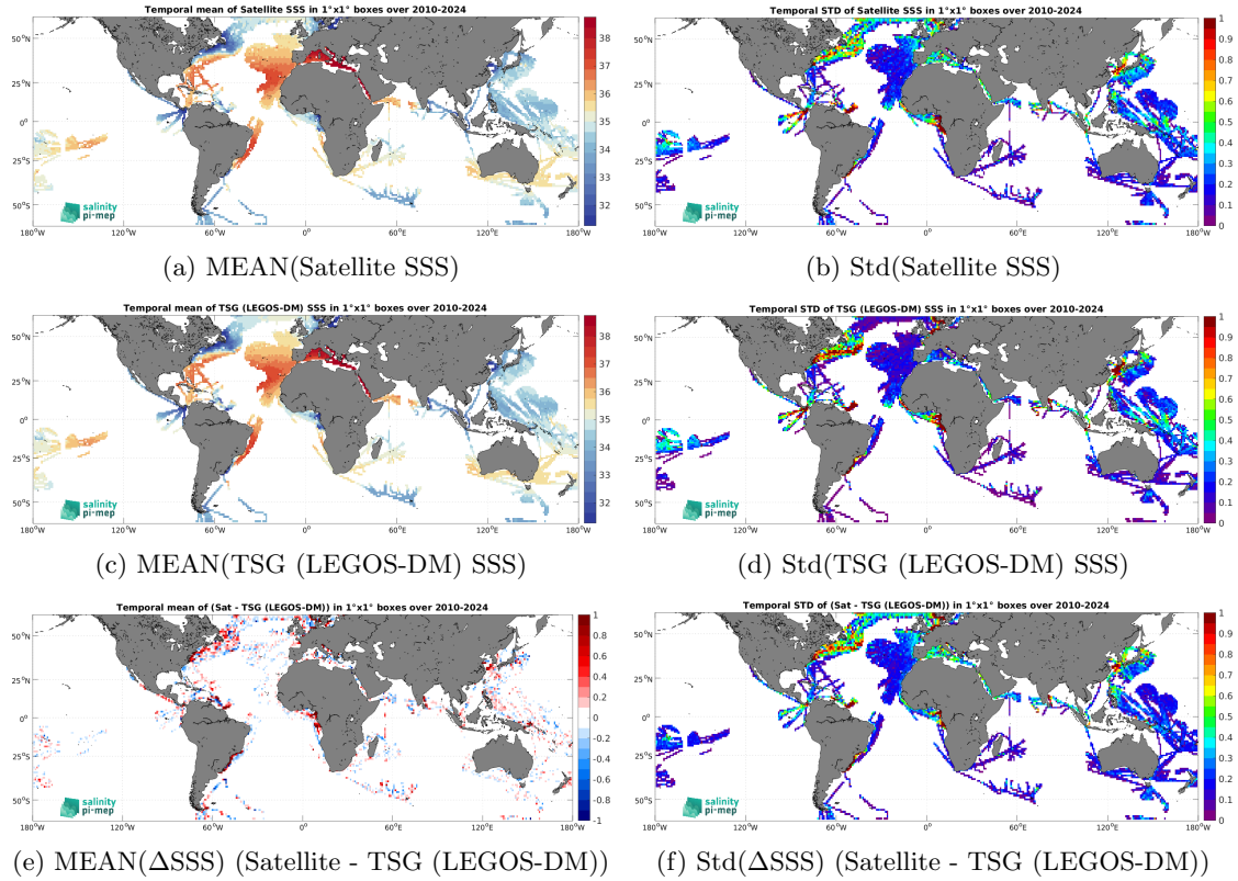
Figure 7: Temporal mean (left) and Std (right) of SSS from SMOS SSS L4 OI v346 - Weekly (CMEMS-CATDS-LOPS) (top), TSG (LEGOS-DM) (middle), and of \Delta SSS (Satellite - TSG (LEGOS-DM)). Only match-up pairs are used to generate these maps.
