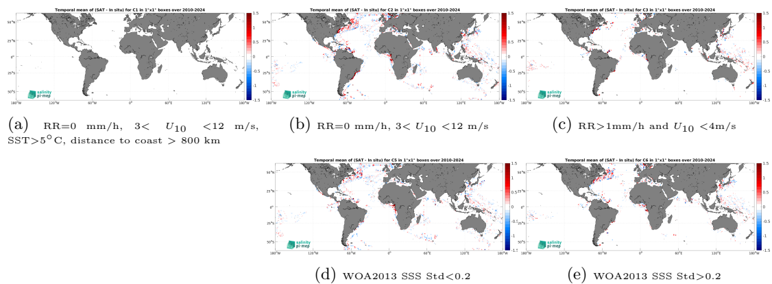
Figure 14: Temporal mean gridded over spatial boxes of size 1^\circ \times 1^\circ of \Delta SSS (SMOS SSS L4 OI v346 - Weekly (CMEMS-CATDS-LOPS) - TSG (LEGOS-DM)) for 5 different subdatasets corresponding to:RR=0 mm/h, 3 < U_{10} < 12 m/s, SST >5^\circ\text{C} , distance to coast > 800 km (a), RR=0 mm/h, 3 < U_{10} < 12 m/s (b), RR >1 mm/h and U_{10} < 4 m/s (c), WOA2013 SSS Std <0.2 (d), WOA2013 SSS Std >0.2 (e).
