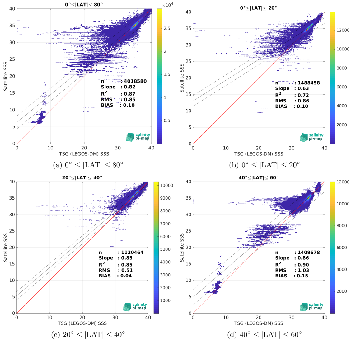
Figure 10: Contour maps of the concentration of SMOS SSS L4 OI v346 - Weekly (CMEMS-CATDS-LOPS) SSS (y-axis) versus TSG (LEGOS-DM) SSS (x-axis) at match-up pairs for different latitude bands. For each plot, the red line shows x=y . The black thin and dashed lines indicate a linear fit through the data cloud and the \pm 95\% confidence levels, respectively. The number match-up pairs n , the slope and R^2 coefficient of the linear fit, the root mean square (RMS) and the mean bias between satellite and in situ data are indicated for each latitude band in each plots.
