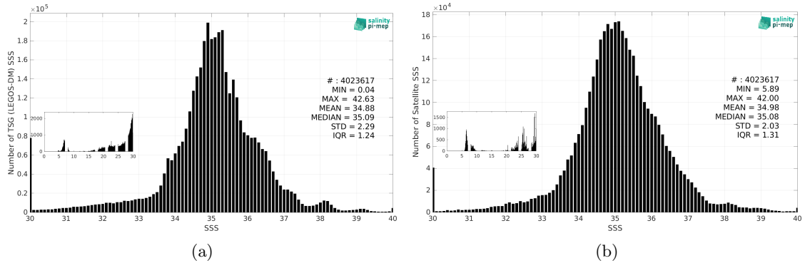
Figure 3: Histograms of SSS from TSG (LEGOS-DM) (a) and SMOS SSS L4 OI v346 - Weekly (CMEMS-CATDS-LOPS) (b) considering all match-up pairs per bins of 0.1 over the SMOS coastal zone (<800km) 60N-60S Pi-MEP region and for the full satellite product period.
