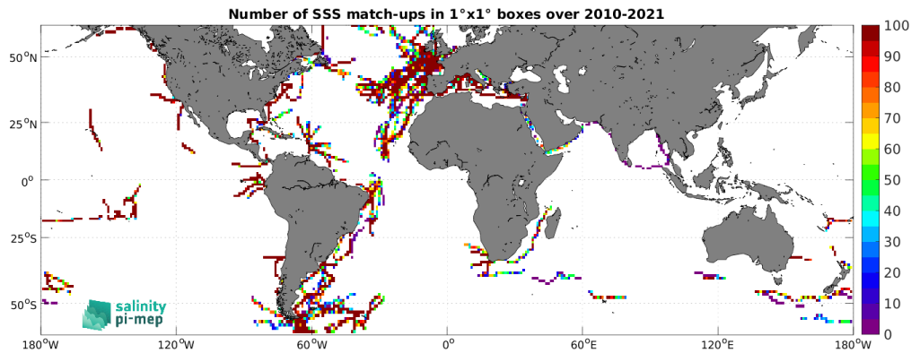
Figure 5: Number of SSS match-ups between TSG (GOSUD-Sailing-ship) SSS and the SMOS SSS L4 OI v346 - Weekly (CMEMS-CATDS-LOPS) SSS product for the SMOS coastal zone (<800km) 60N-60S Pi-MEP region over 1^\circ \times 1^\circ boxes and for the full satellite product period.
