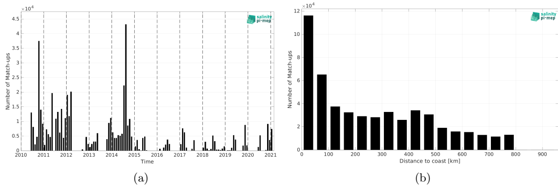
Figure 2: Number of match-ups between TSG (GOSUD-Sailing-ship) and SMOS SSS L4 OI v346 - Weekly (CMEMS-CATDS-LOPS) SSS as a function of time (a) and as function of the distance to coast (b) over the SMOS coastal zone (<800km) 60N-60S Pi-MEP region and for the full satellite product period.
