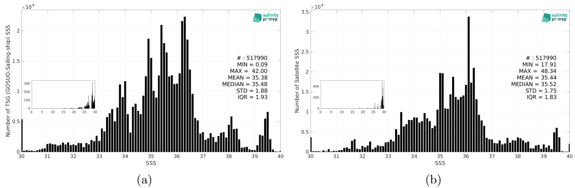
Figure 3: Histograms of SSS from TSG (GOSUD-Sailing-ship) (a) and SMOS SSS L4 OI v346 - Weekly (CMEMS-CATDS-LOPS) (b) considering all match-up pairs per bins of 0.1 over the SMOS coastal zone (<800km) 60N-60S Pi-MEP region and for the full satellite product period.
