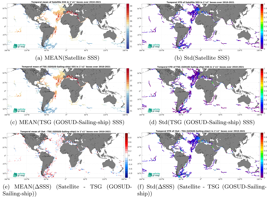
Figure 7: Temporal mean (left) and Std (right) of SSS from SMOS SSS L4 OI v346 - Weekly (CMEMS-CATDS-LOPS) (top), TSG (GOSUD-Sailing-ship) (middle), and of \Delta SSS (Satellite - TSG (GOSUD-Sailing-ship)). Only match-up pairs are used to generate these maps.
