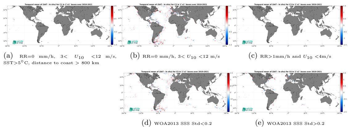
Figure 14: Temporal mean gridded over spatial boxes of size 1^\circ \times 1^\circ of \Delta SSS (SMOS SSS L4 OI v346 - Weekly (CMEMS-CATDS-LOPS) - TSG (GOSUD-Sailing-ship)) for 5 different sub-datasets corresponding to:RR=0 mm/h, 3 < U_{10} < 12 m/s, SST >5^\circ\text{C} , distance to coast > 800 km (a), RR=0 mm/h, 3 < U_{10} < 12 m/s (b), RR >1 mm/h and U_{10} < 4 m/s (c), WOA2013 SSS Std <0.2 (d), WOA2013 SSS Std >0.2 (e).
