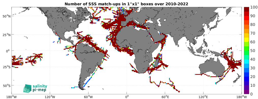
Figure 5: Number of SSS match-ups between TSG (GOSUD-Research-vessel) SSS and the SMOS SSS L4 OI v346 - Weekly (CMEMS-CATDS-LOPS) SSS product for the SMOS coastal zone ( <800\text{km} ) 60\text{N} - 60\text{S} Pi-MEP region over 1^\circ \times 1^\circ boxes and for the full satellite product period.
