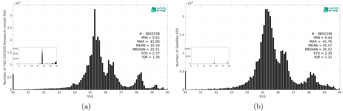
Figure 3: Histograms of SSS from TSG (GOSUD-Research-vessel) (a) and SMOS SSS L4 OI v346 - Weekly (CMEMS-CATDS-LOPS) (b) considering all match-up pairs per bins of 0.1 over the SMOS coastal zone (<800km) 60N-60S Pi-MEP region and for the full satellite product period.
