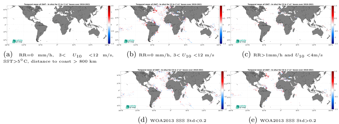
Figure 14: Temporal mean gridded over spatial boxes of size 1^\circ \times 1^\circ of \Delta SSS (SMOS SSS L4 OI v346 - Weekly (CMEMS-CATDS-LOPS) - TSG (GOSUD-Research-vessel)) for 5 different subdatasets corresponding to:RR=0 mm/h, 3 < U_{10} < 12 m/s, SST > 5^\circ\text{C} , distance to coast > 800 km (a), RR=0 mm/h, 3 < U_{10} < 12 m/s (b), RR > 1 mm/h and U_{10} < 4 m/s (c), WOA2013 SSS Std < 0.2 (d), WOA2013 SSS Std > 0.2 (e).
