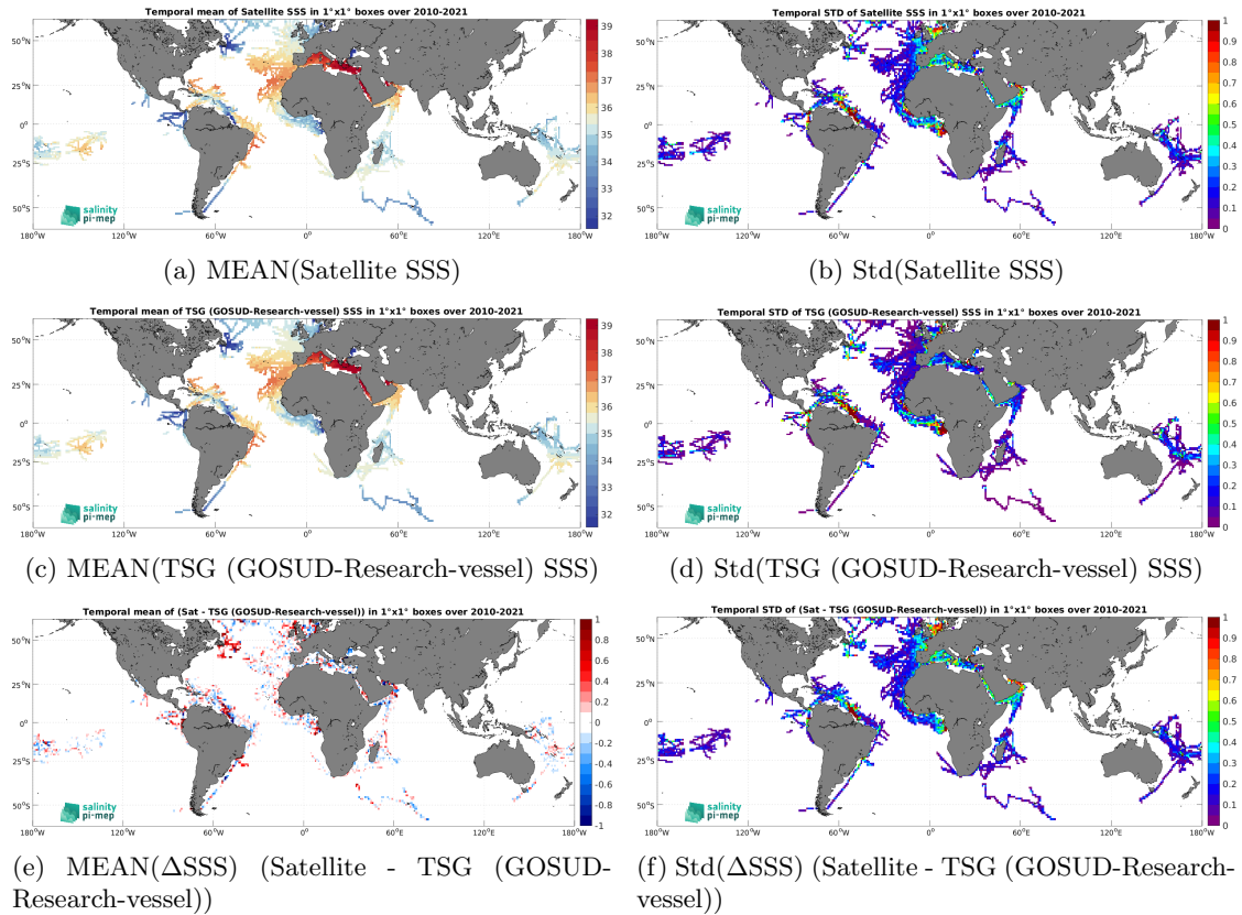
Figure 7: Temporal mean (left) and Std (right) of SSS from SMOS SSS L4 OI v346 - Weekly (CMEMS-CATDS-LOPS) (top), TSG (GOSUD-Research-vessel) (middle), and of \Delta SSS (Satellite - TSG (GOSUD-Research-vessel)). Only match-up pairs are used to generate these maps.
