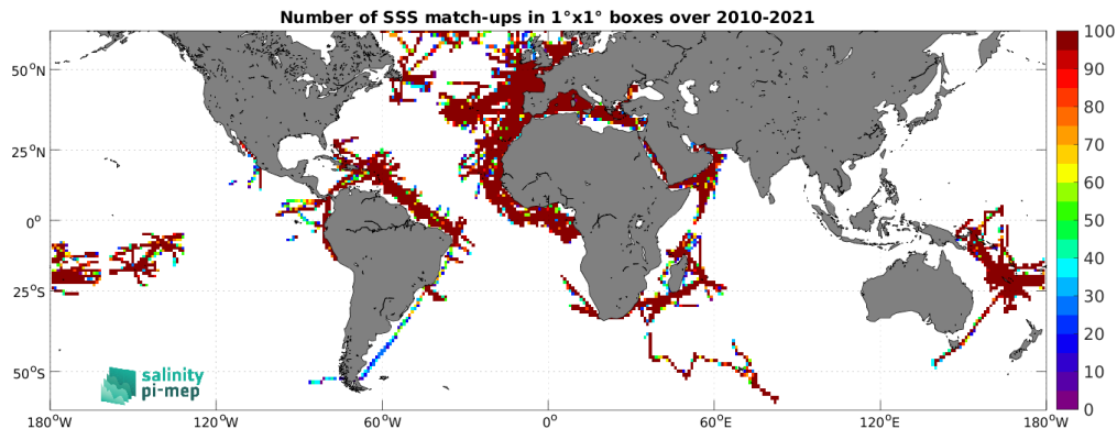
Figure 5: Number of SSS match-ups between TSG (GOSUD-Research-vessel) SSS and the SMOS SSS L4 OI v346 - Weekly (CMEMS-CATDS-LOPS) SSS product for the SMOS coastal zone (<800km) 60N-60S Pi-MEP region over 1^\circ \times 1^\circ boxes and for the full satellite product period.
