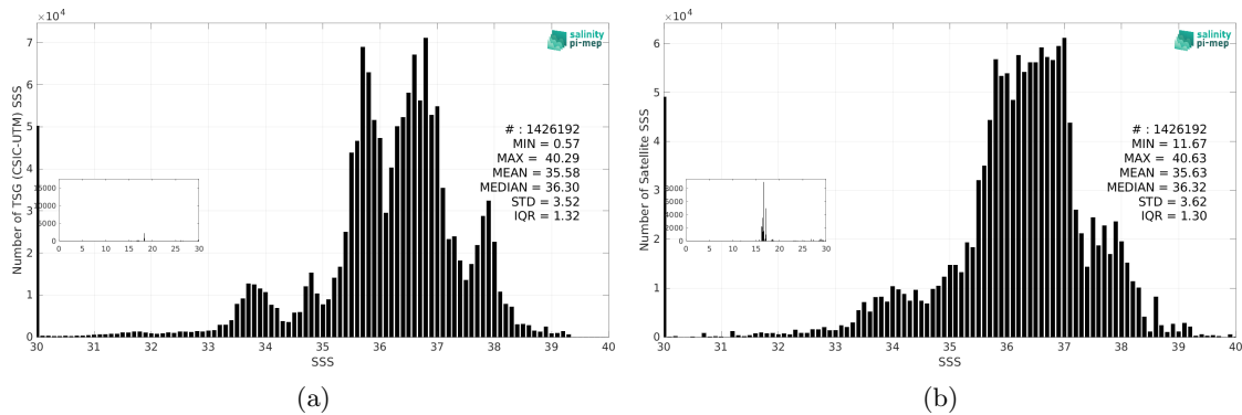
Figure 3: Histograms of SSS from TSG (CSIC-UTM) (a) and SMOS SSS L4 OI v346 - Weekly (CMEMS-CATDS-LOPS) (b) considering all match-up pairs per bins of 0.1 over the SMOS coastal zone (<800km) 60N-60S Pi-MEP region and for the full satellite product period.
